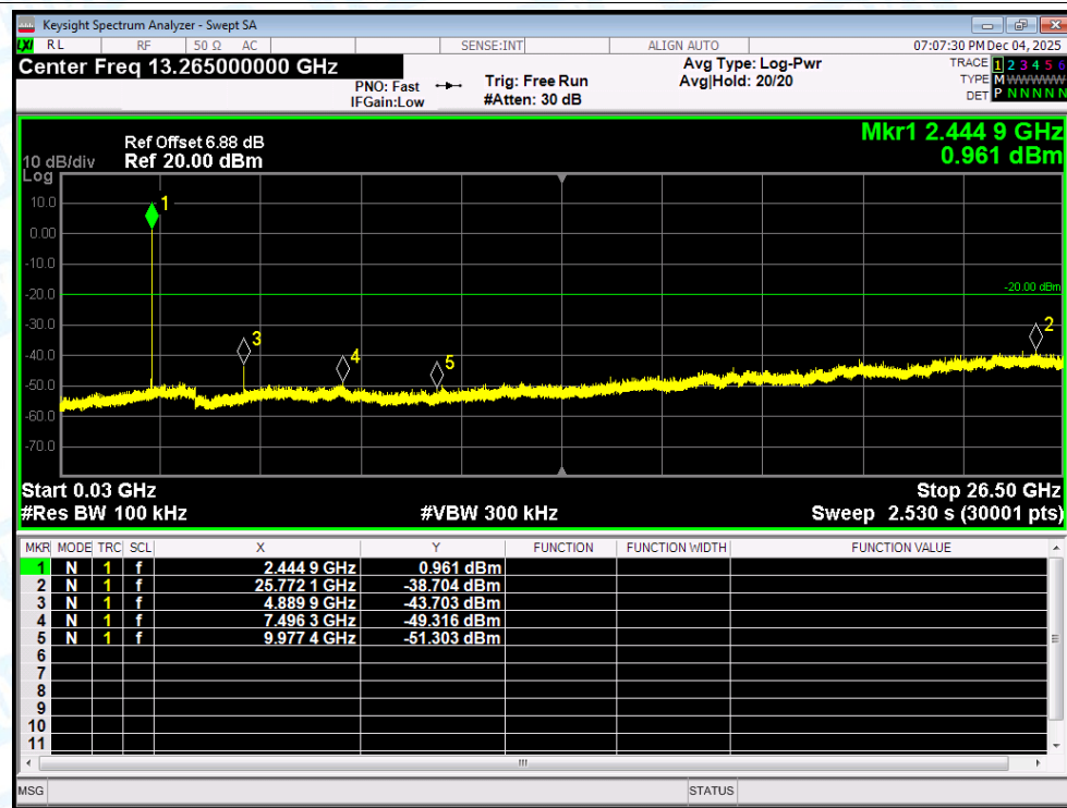
Tx. Spurious NVNT Thread 2445MHz Ant1 Emission
