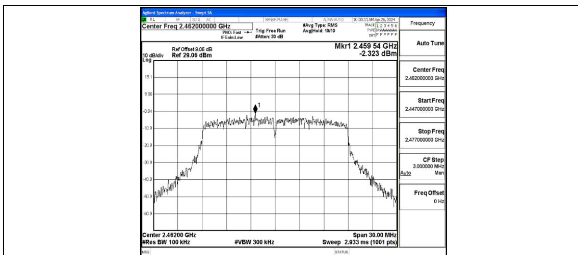
11N20SISO-Ant1-2462-0~Reference-PASS
