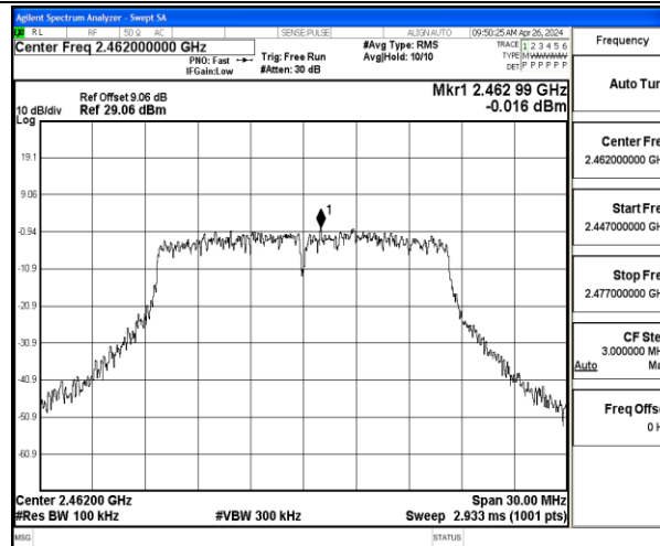
11G-Ant1-2462-0~Reference-PASS
