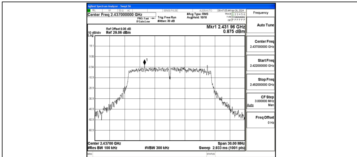
11G-Ant1-2437-0~Reference-PASS
