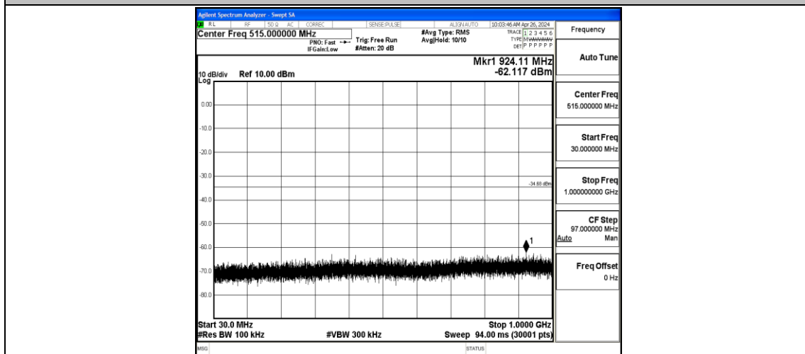
11N40SISO-Ant1-2422-30~1000-PASS
