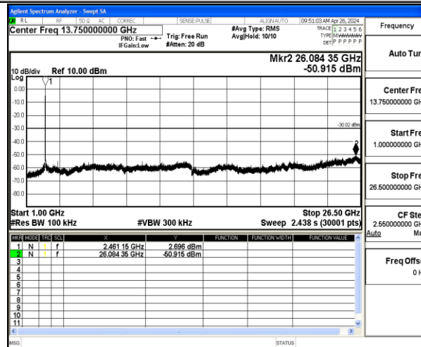
11G-Ant1-2462-1000~26500-PASS
