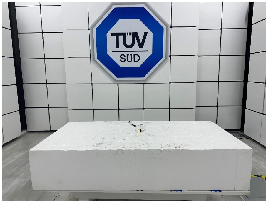
RYGD315 Set-up for Spurious Emissions Front View
