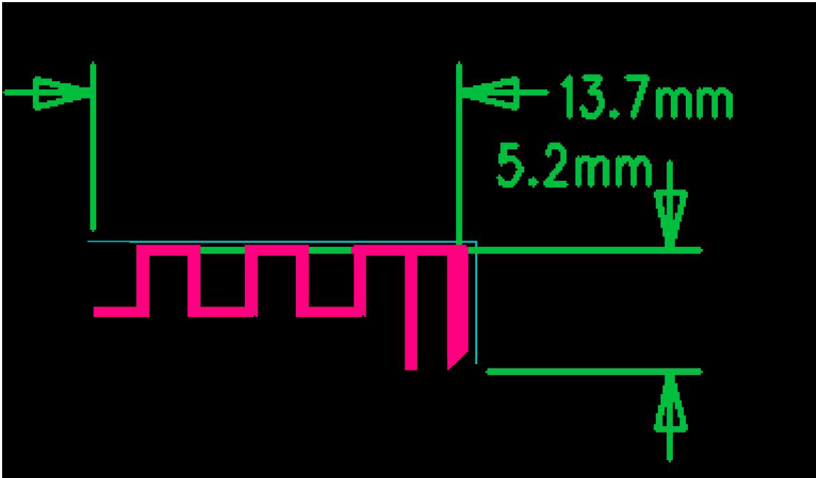
Antenna Photo & Length (mm)
