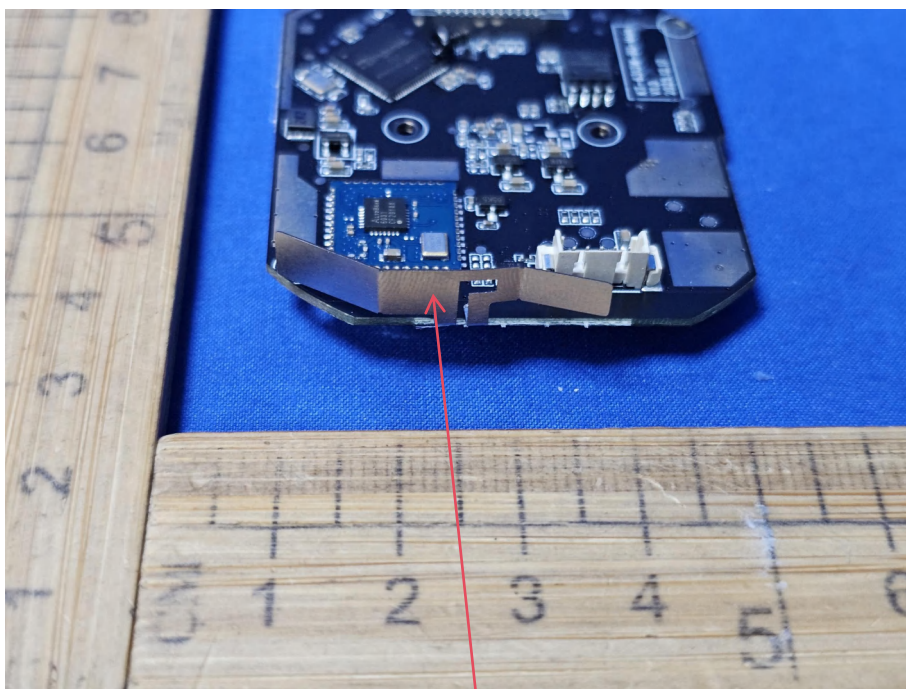
shrapnel antenna
