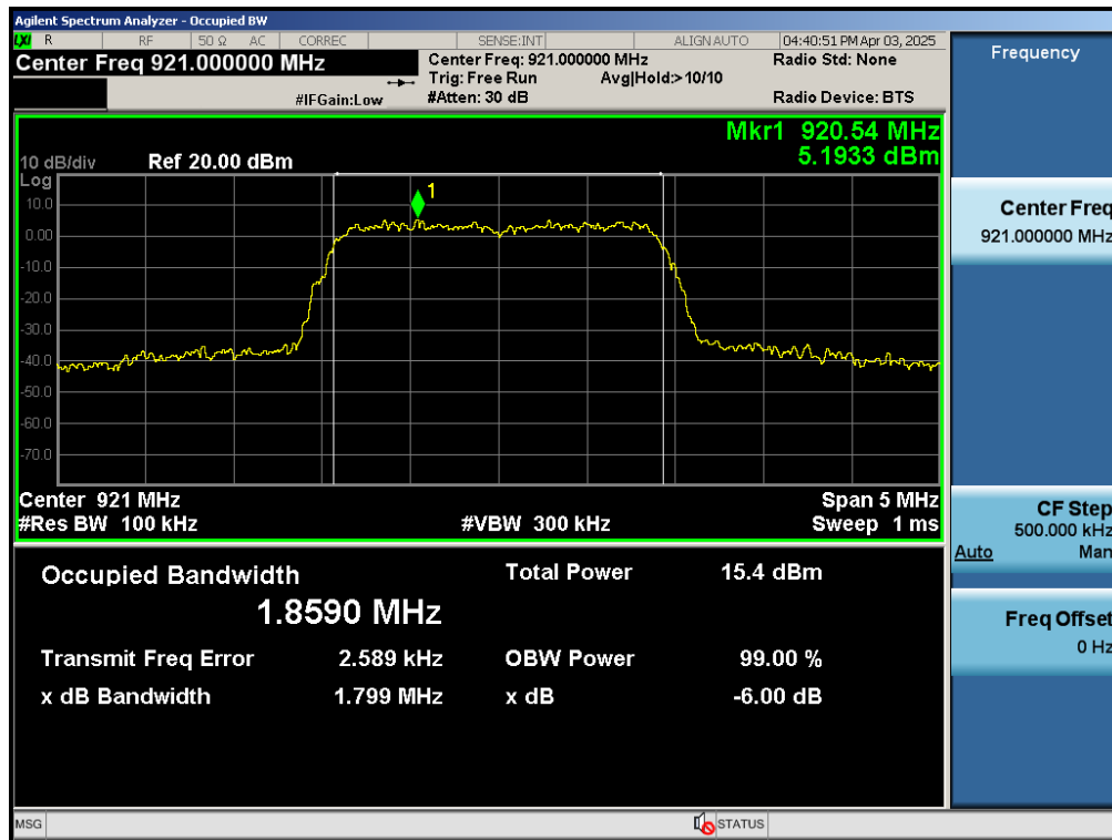
Test_Graph_802.11ah_ANT1_921_BW 2MHz_DTS Bandwidth
