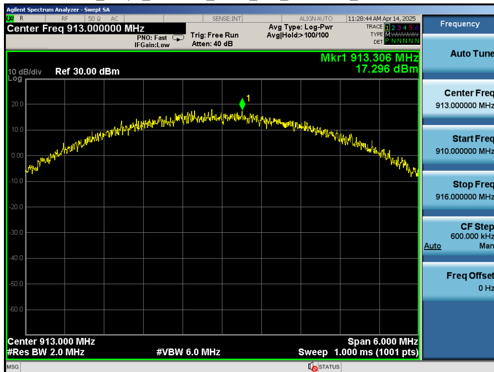
Test_Graph_802.11ah_ANT1_913_BW 2MHz_Peak Power
