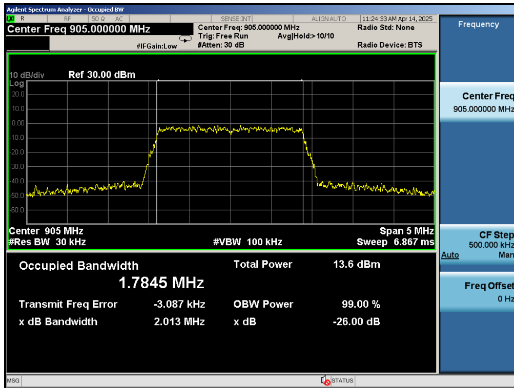
Test_Graph_802.11ah_ANT1_905_BW 2MHz_Occupied Bandwidth
