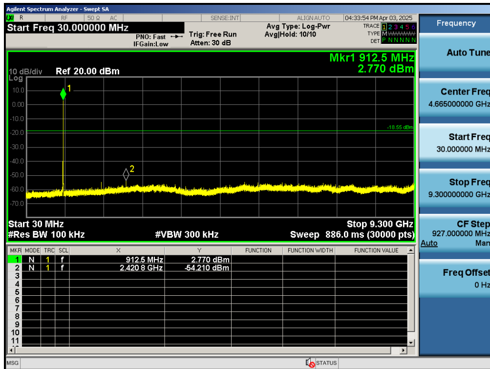
Test_Graph_802.11ah_ANT1_913_BW 2MHz_Frequency Band 3
