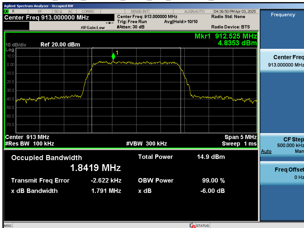
Test_Graph_802.11ah_ANT1_913_BW 2MHz_DTS Bandwidth
