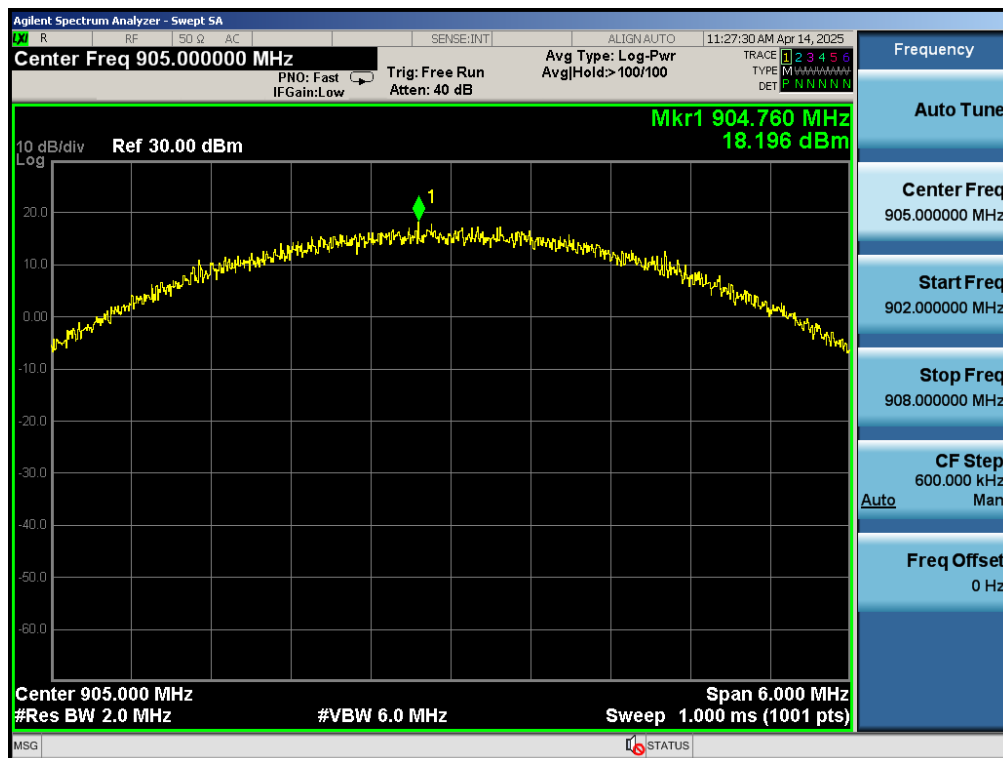
Test_Graph_802.11ah_ANT1_905_BW 2MHz_Peak Power
