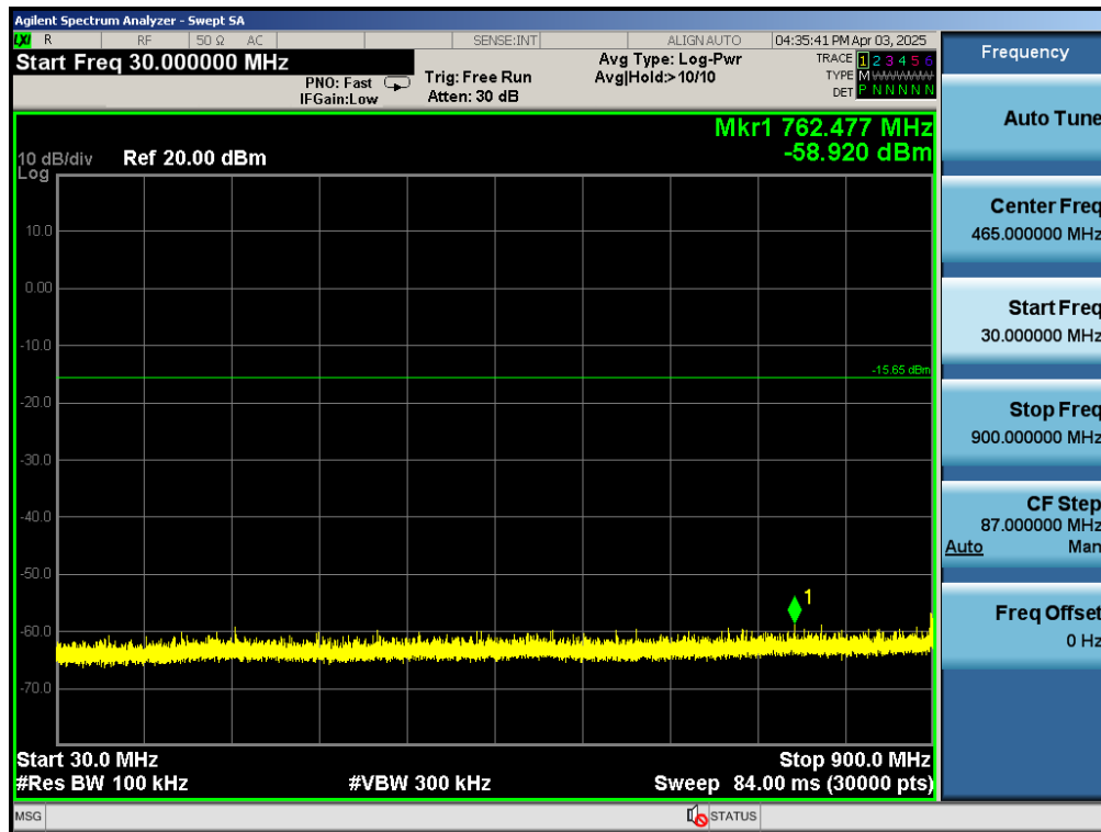
Test_Graph_802.11ah_ANT1_913_BW 2MHz_ Frequency Band 1
