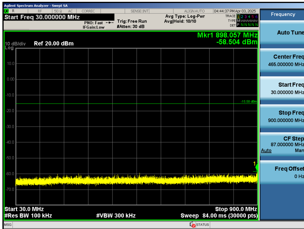
Test_Graph_802.11ah_ANT1_921_BW 2MHz_ Frequency Band 1
