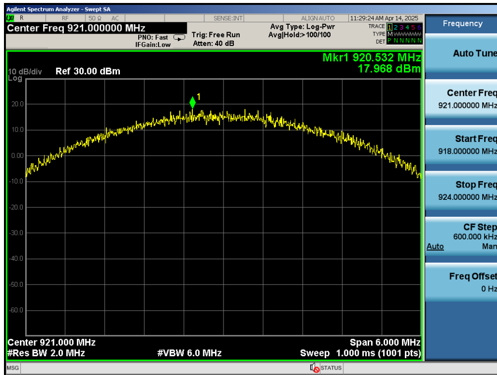
Test_Graph_802.11ah_ANT1_921_BW 2MHz_Peak Power
