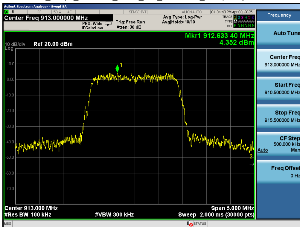
Test_Graph_802.11ah_ANT1_913_BW 2MHz_Reference level
