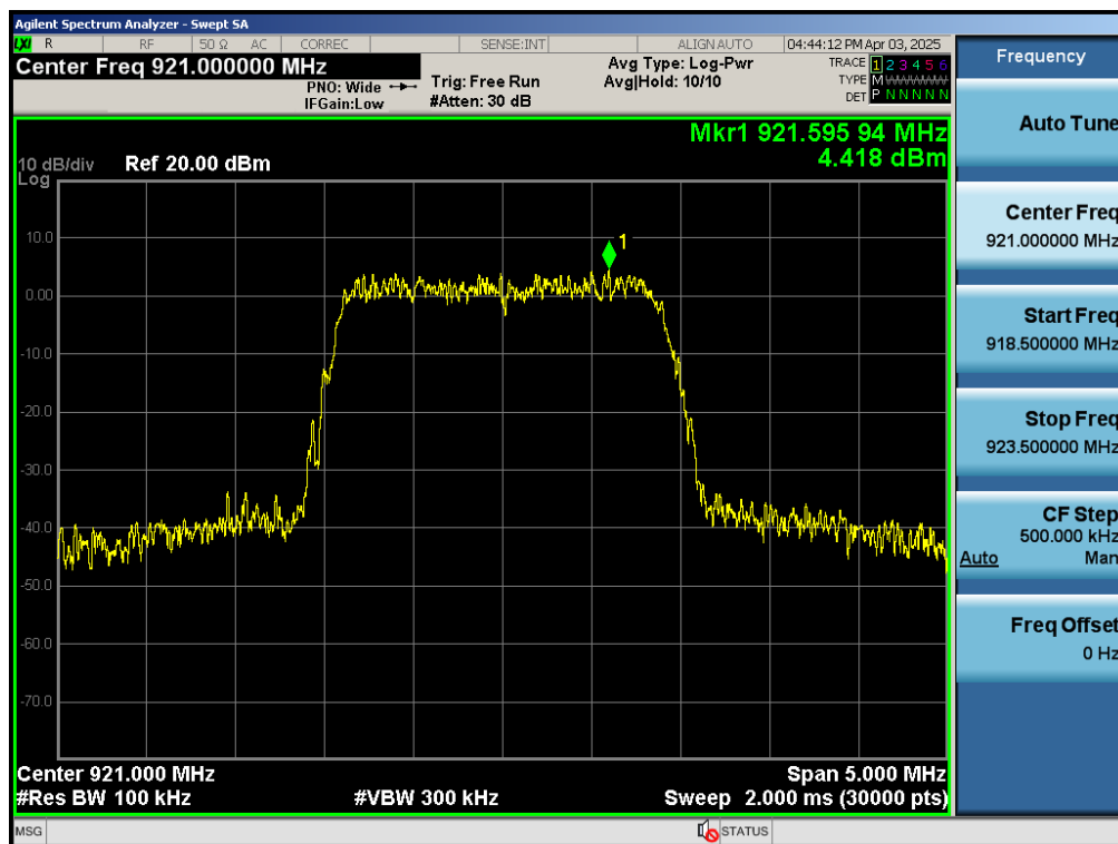
Test_Graph_802.11ah_ANT1_921_BW 2MHz_Reference level
