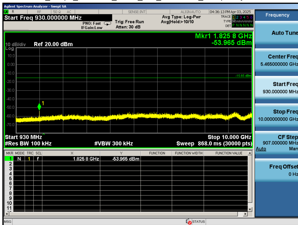
Test_Graph_802.11ah_ANT1_913_BW 2MHz_ Frequency Band 2
