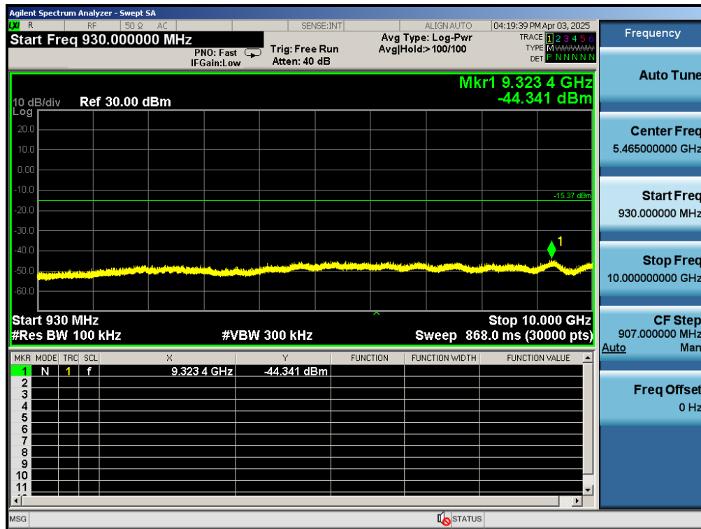
Test_Graph_802.11ah_ANT1_905_BW 2MHz_ Frequency Band 2
