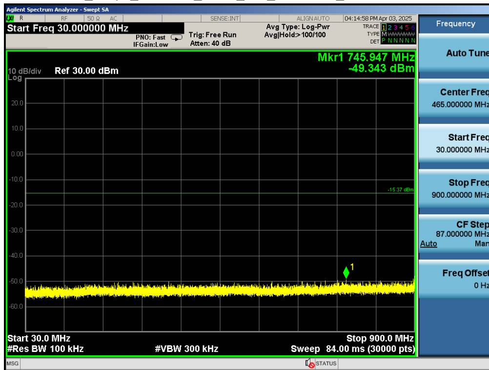
Test_Graph_802.11ah_ANT1_905_BW 2MHz_Frequency Band 1
