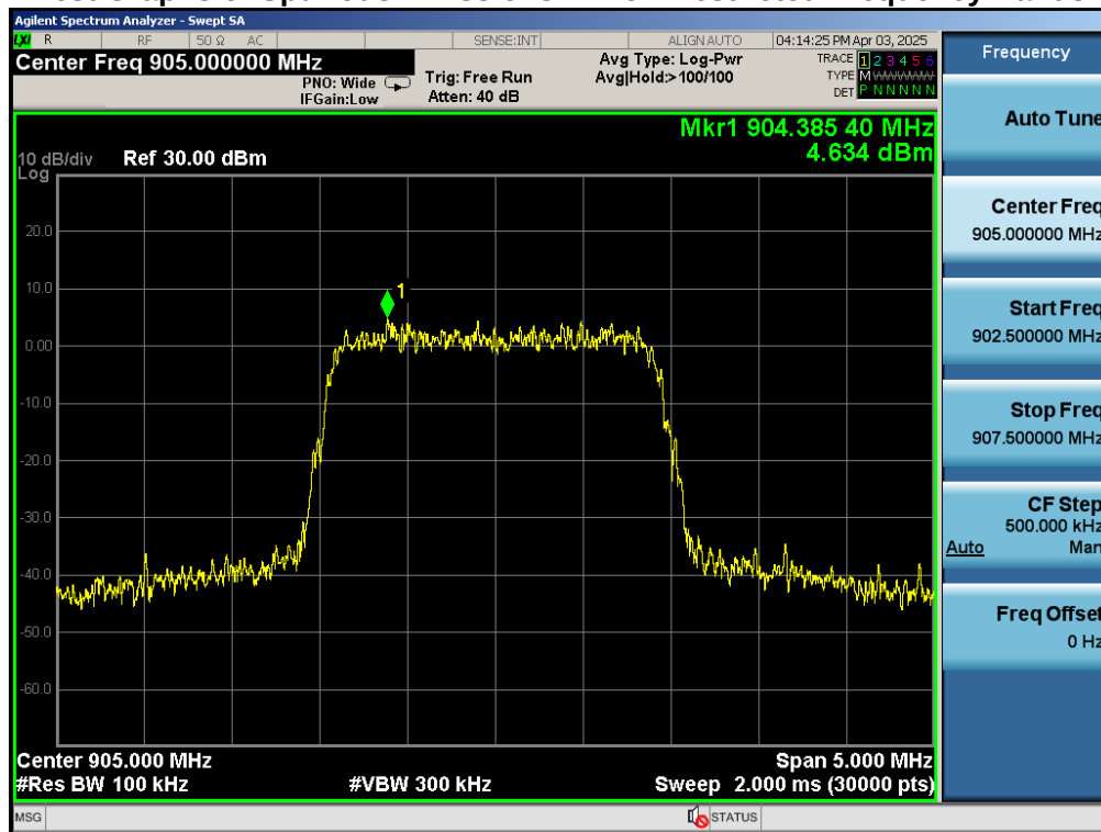
Test_Graph_802.11ah_ANT1_905_BW 2MHz_Reference level
