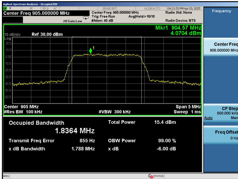
Test_Graph_802.11ah_ANT1_905_BW 2MHz_DTS Bandwidth
