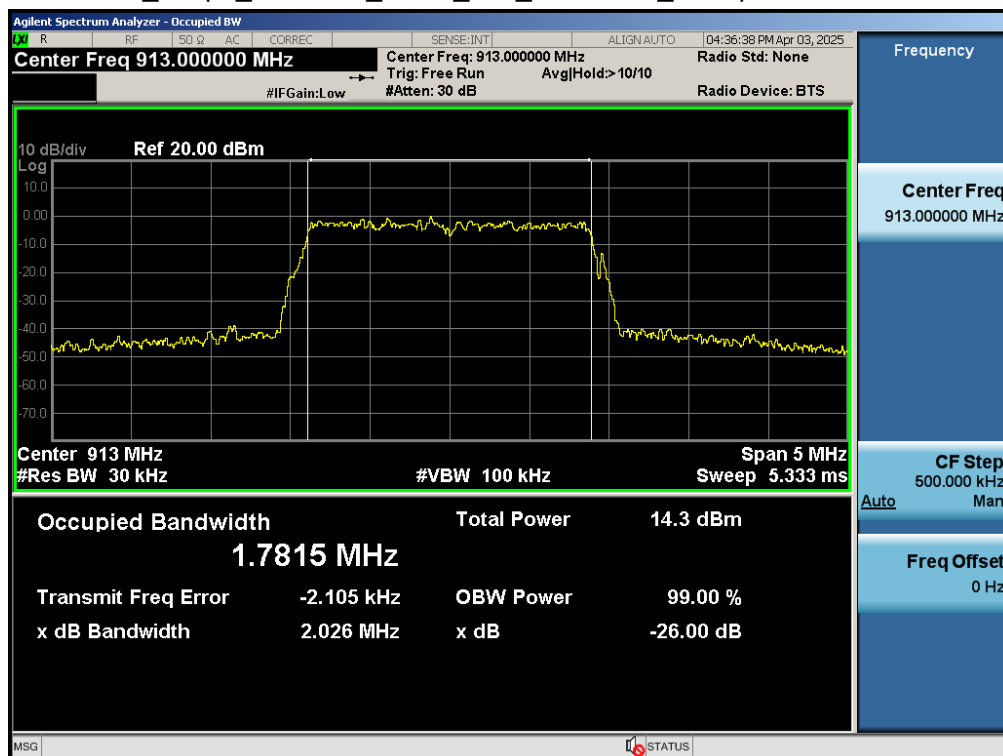
Test_Graph_802.11ah_ANT1_913_BW 2MHz_Occupied Bandwidth
