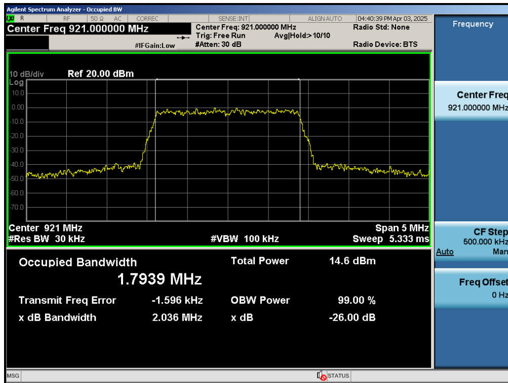
Test_Graph_802.11ah_ANT1_921_BW 2MHz_Occupied Bandwidth
