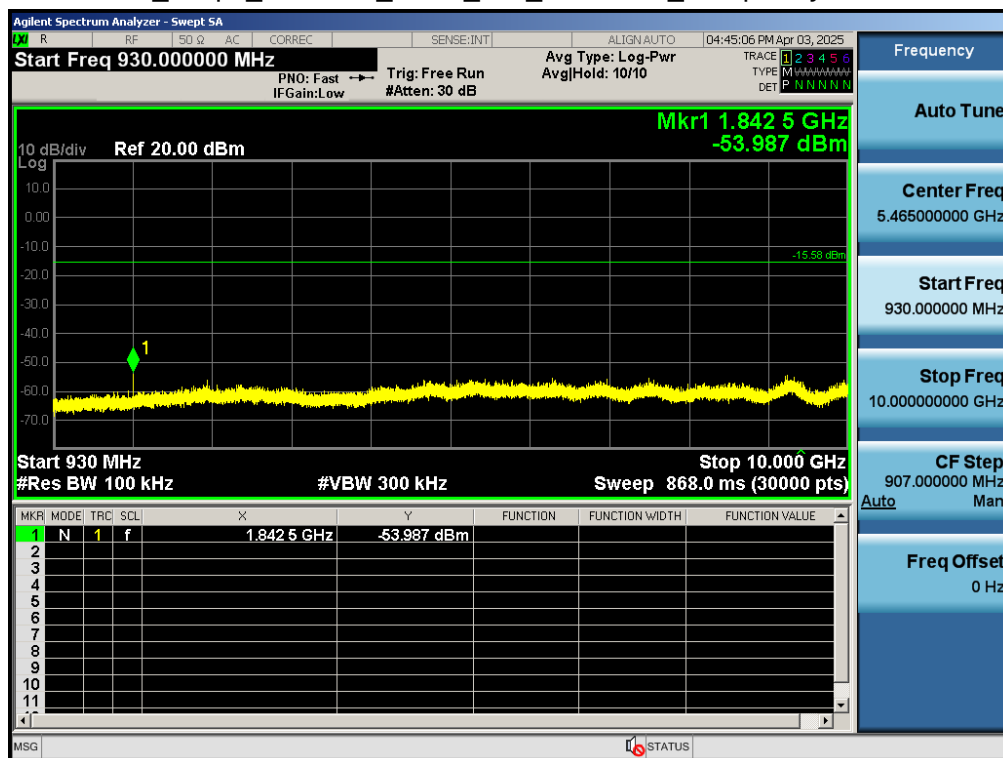
Test_Graph_802.11ah_ANT1_921_BW 2MHz_ Frequency Band 2
