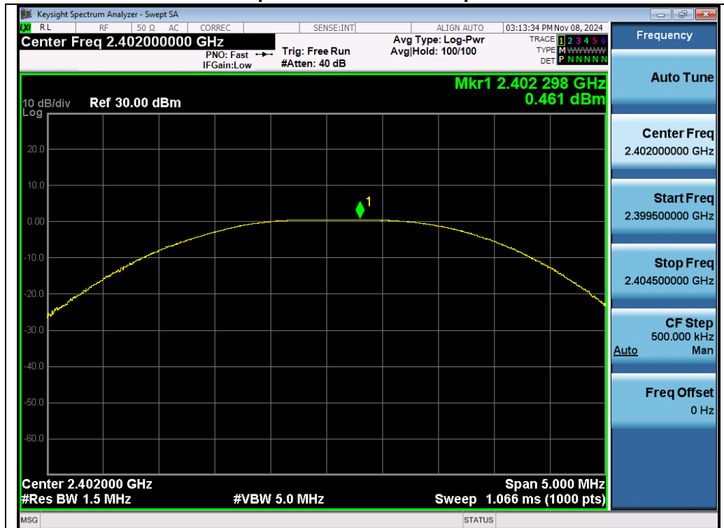
Test_Graph_LE1M_ANT1_2402_1Mbps_Peak Power
