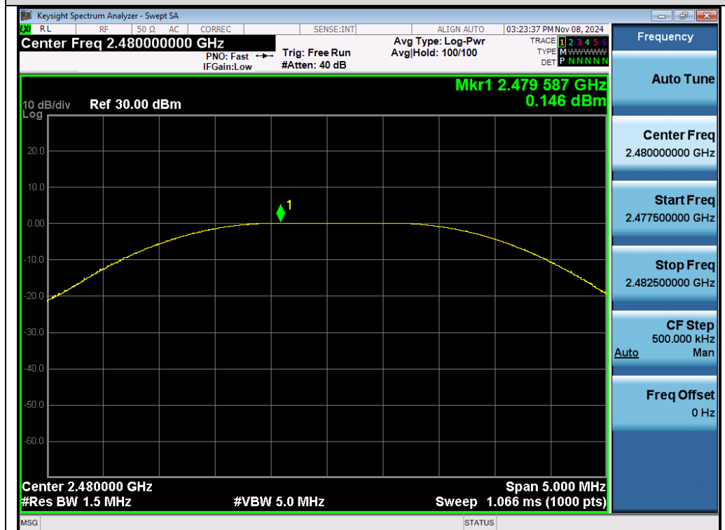
Test_Graph_LE2M_ANT1_2480_2Mbps_Peak Power
