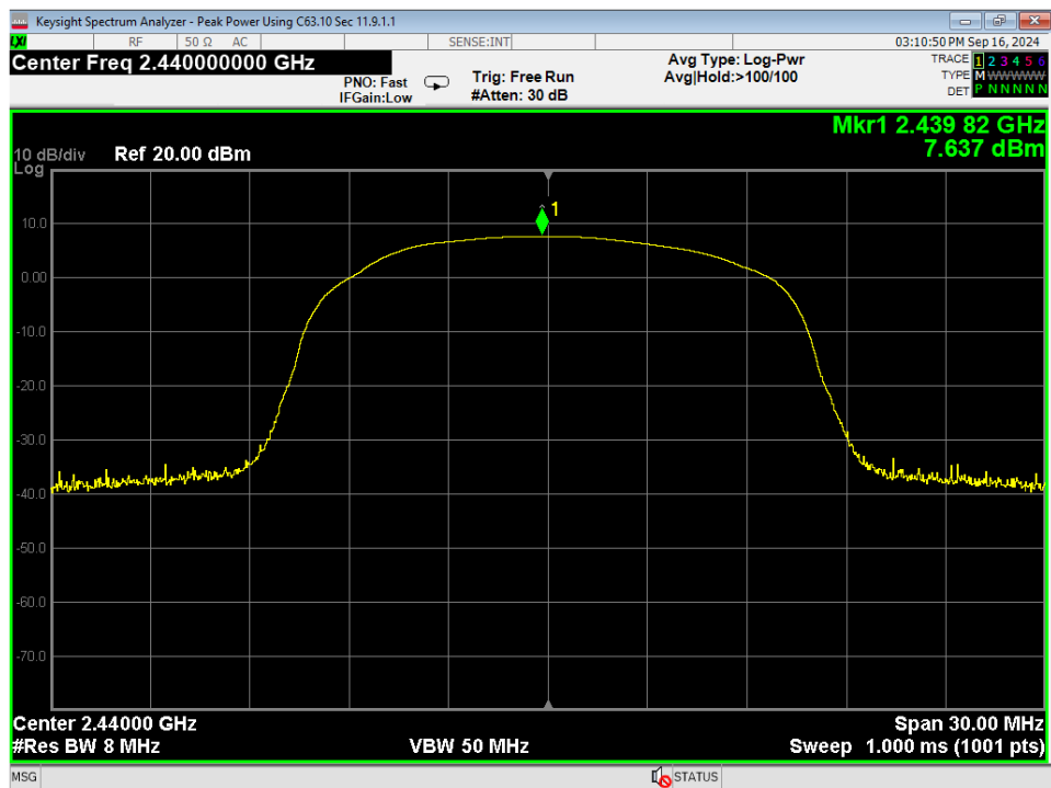
18 Peak Power, Mid Channel, BLE 2MB
