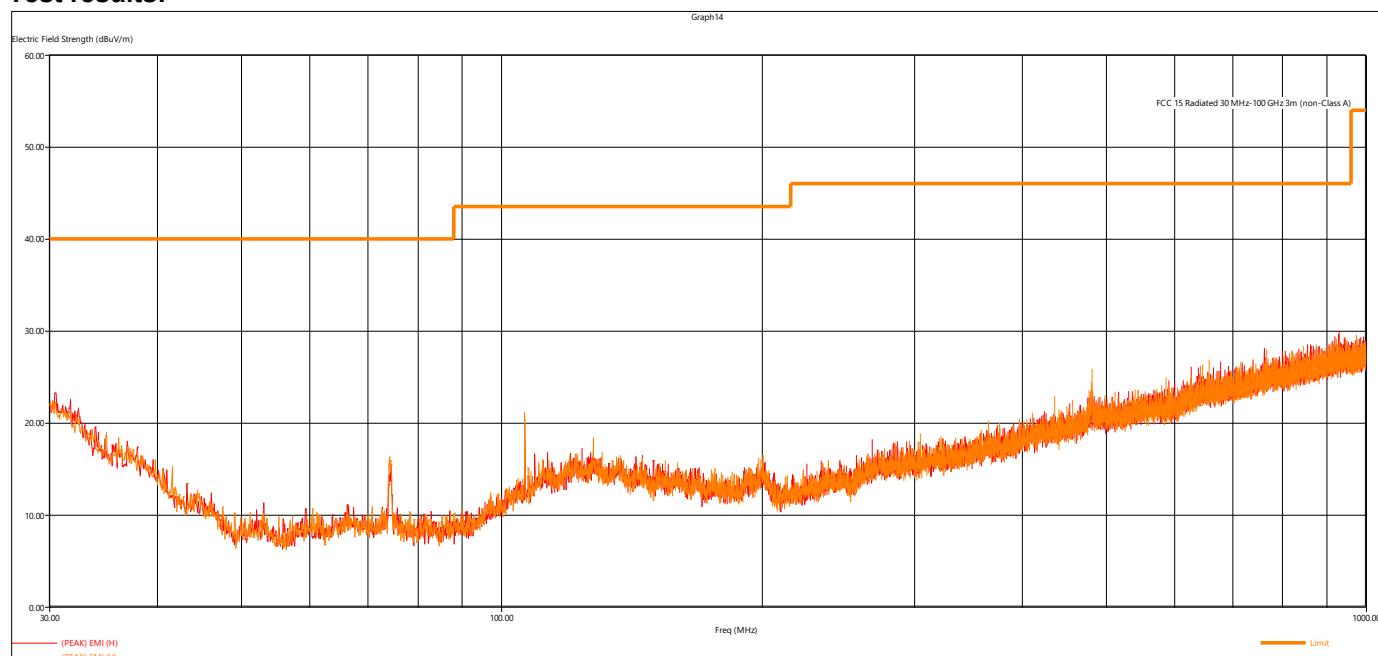
Figure 5 - Radiated Emissions Plot, 30MHz – 1GHz
