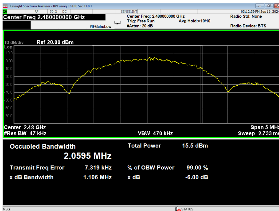
32 Occupied Bandwidth, High Channel, BLE 2MB
