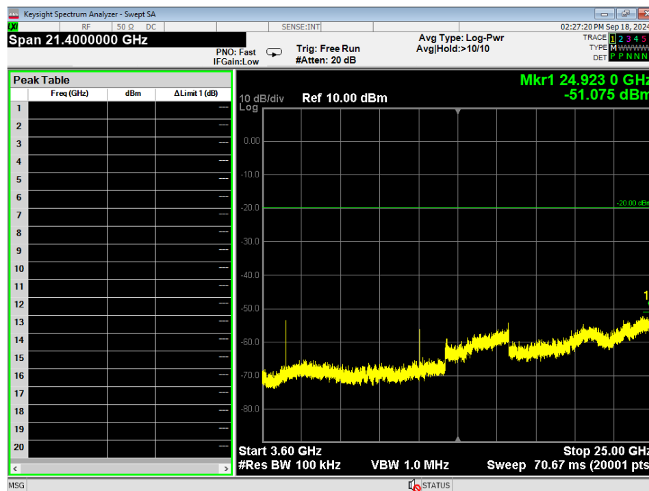
Figure 8 - Conducted Emissions Plot, GMSK 1MB, 3.6GHz – 25GHz, Mid
