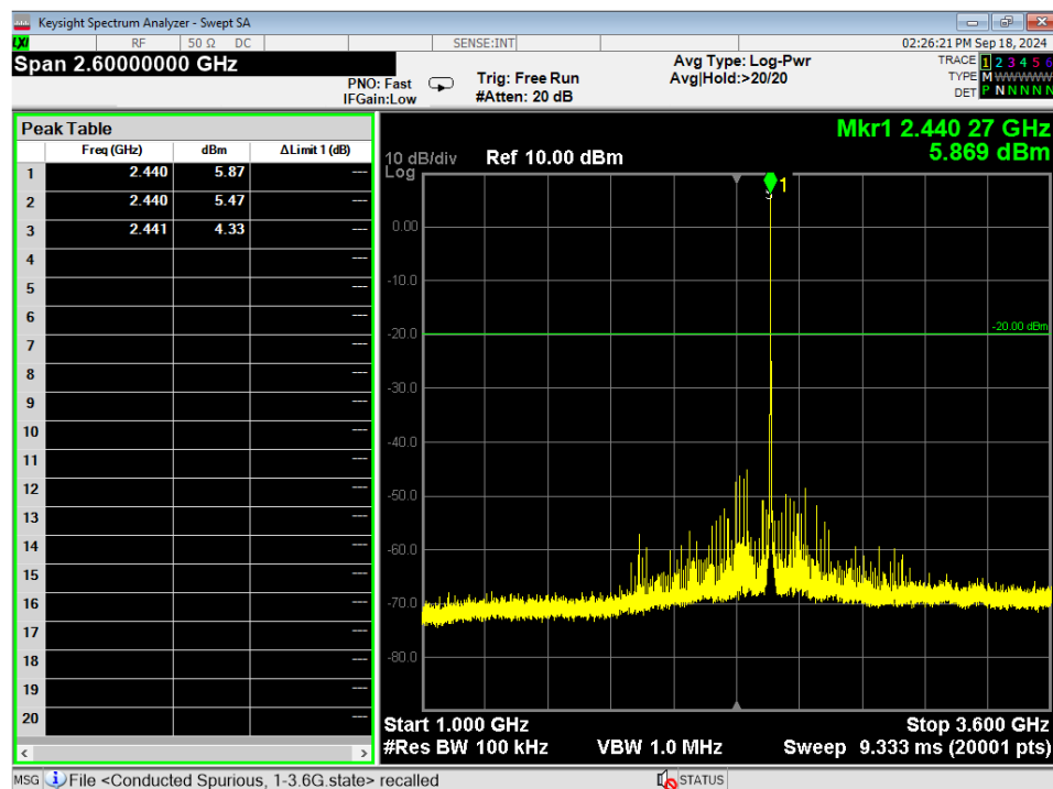
Figure 10 - Conducted Emissions Plot, GMSK 2MB, 1GHz – 3.6GHz, Mid
