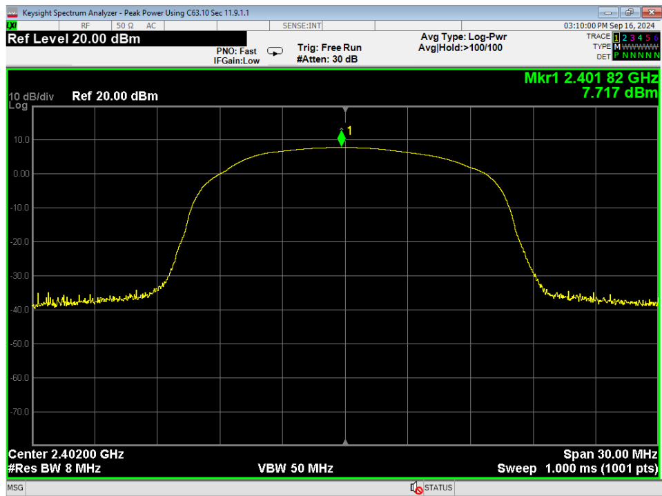
17 Peak Power, Low Channel, BLE 2MB
