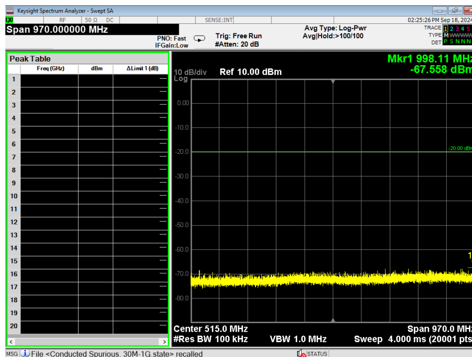
Figure 9 - Conducted Emissions Plot, GMSK 2MB, 30MHz – 1GHz, Mid
