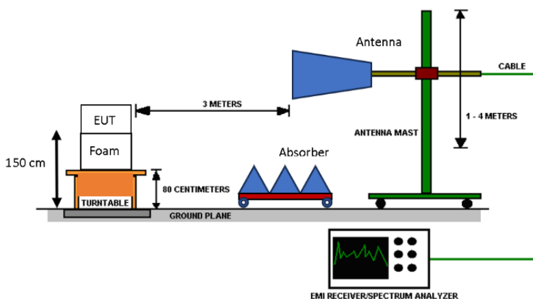
Figure 4 - Radiated Emissions Test Setup
