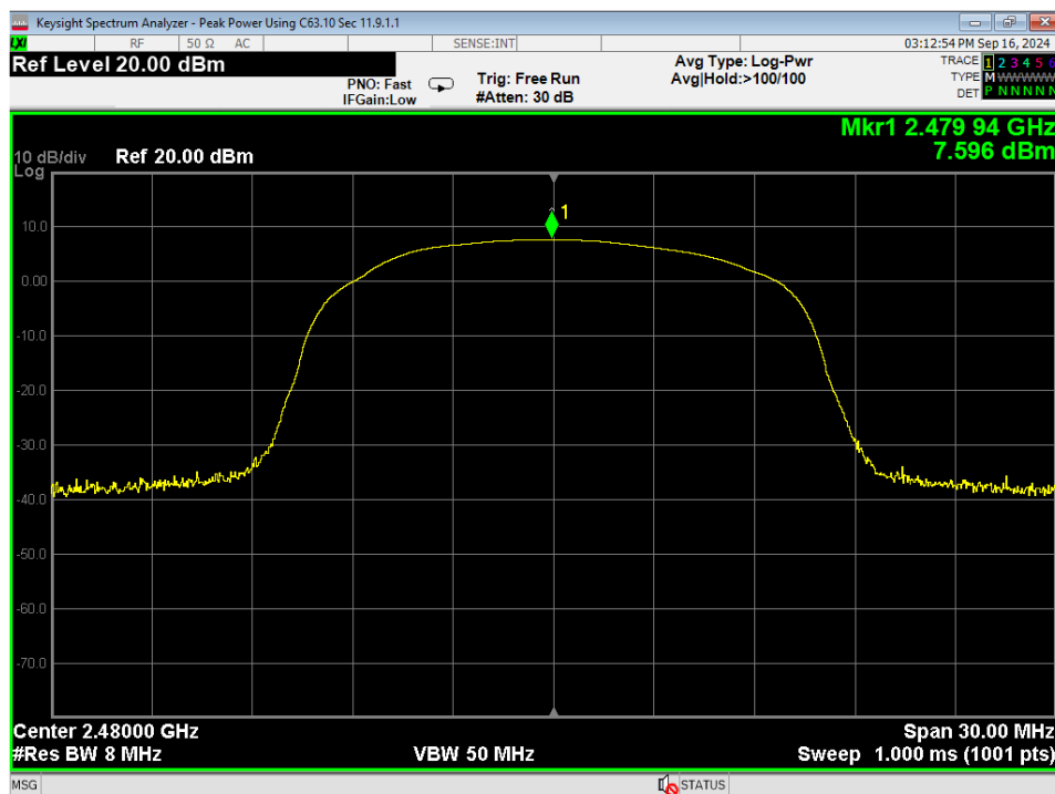
19 Peak Power, High Channel, BLE 2MB
