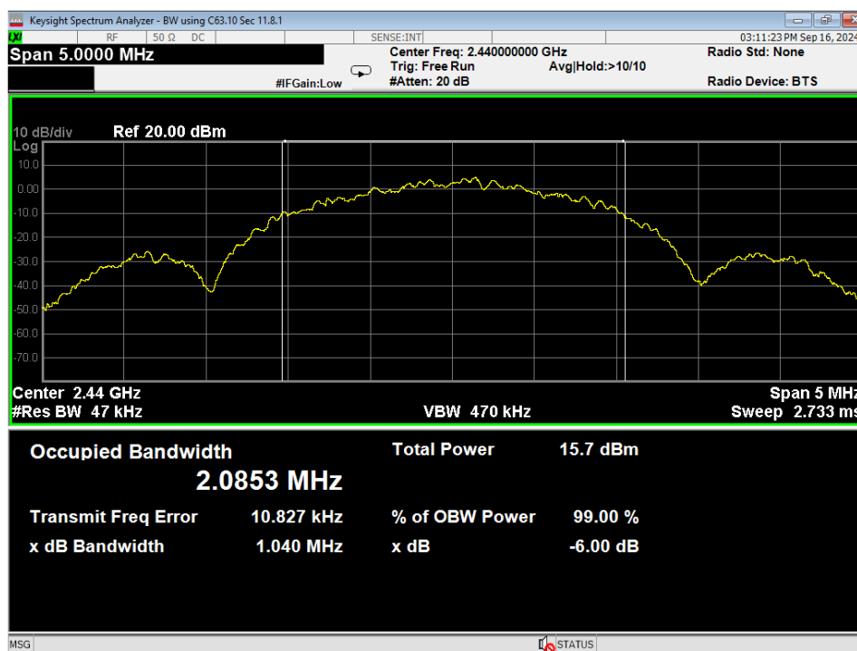
31 Occupied Bandwidth, Mid Channel, BLE 2MB
