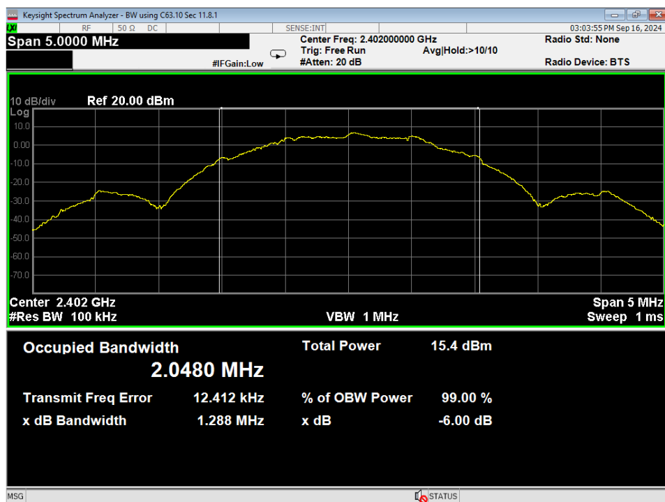
20 6dB Bandwidth, Low Channel, BLE 2MB
