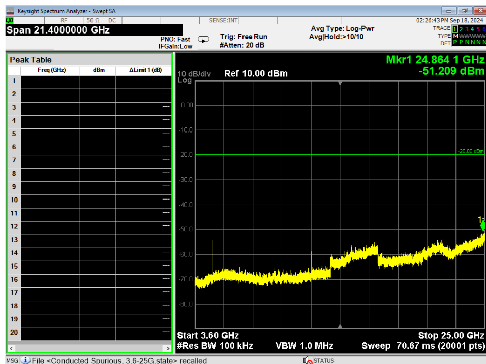
Figure 11 - Conducted Emissions Plot, GMSK 2MB, 3.6GHz – 25GHz, Mid
