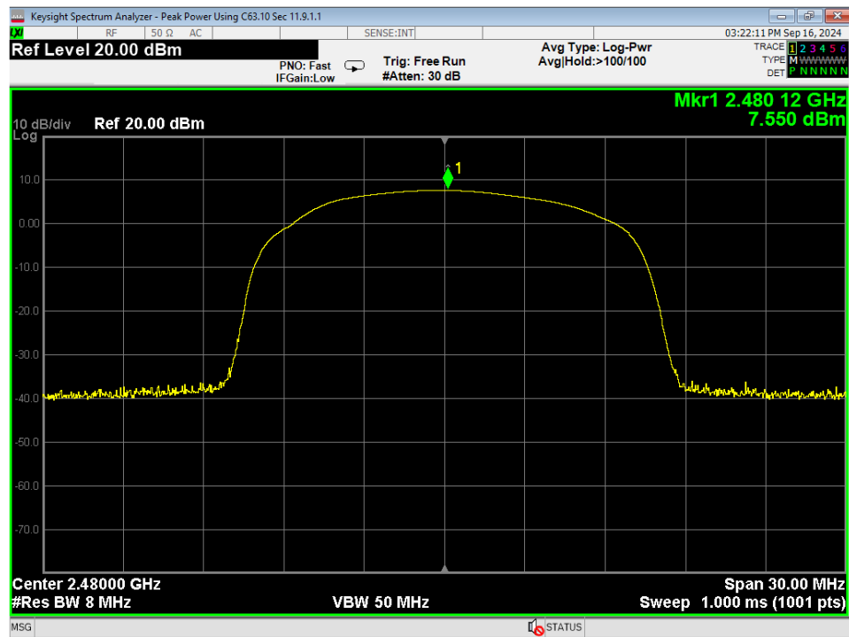
03 Peak Power, High Channel, BLE 1MB
