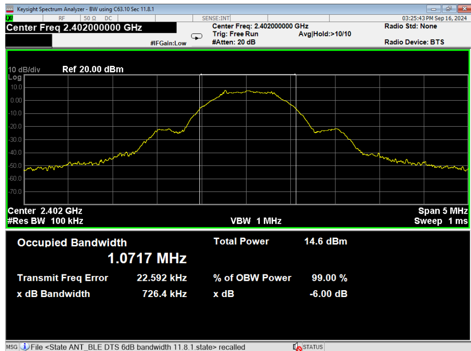
04 6dB Bandwidth, Low Channel, BLE 1MB
