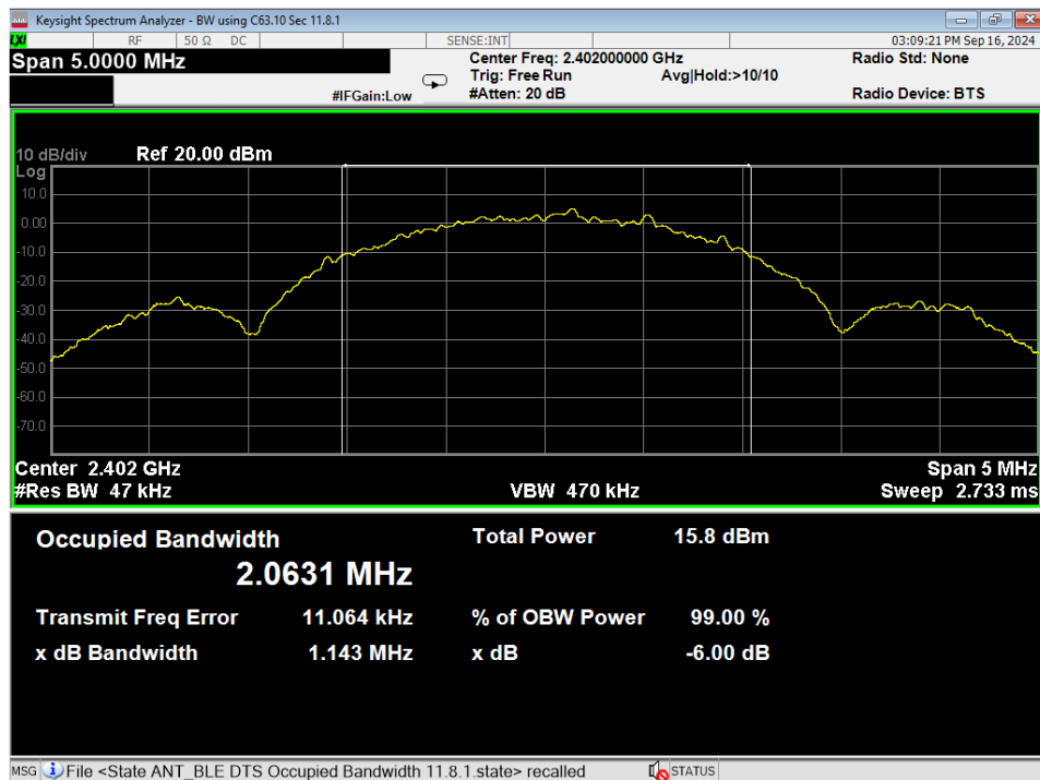
30 Occupied Bandwidth, Low Channel, BLE 2MB
