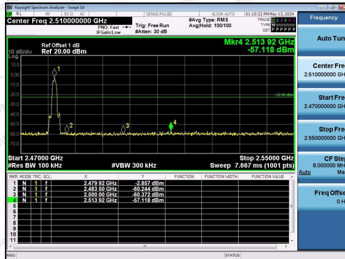
3DH5-Ant1-2480-PASS
