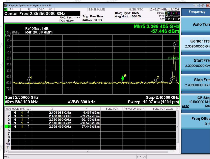
DH5-Ant1-2402-PASS
