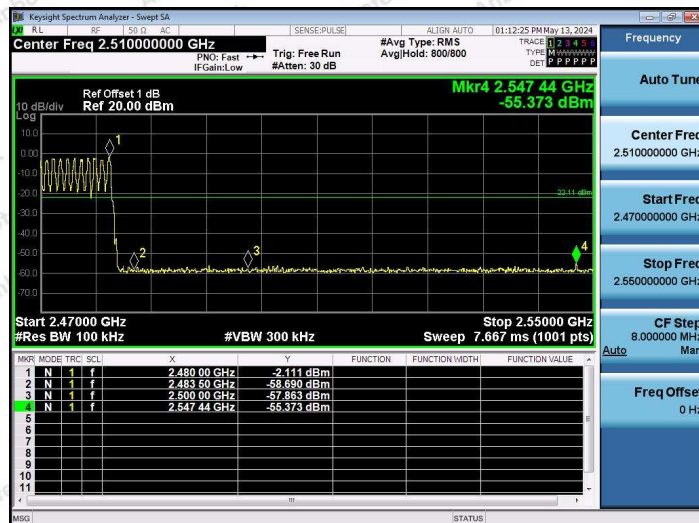
DH5-Ant1-Hop_2480-PASS
