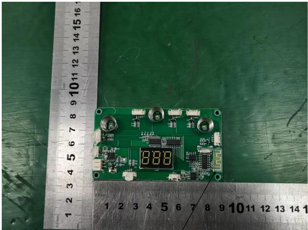
PCB ANTENNA
