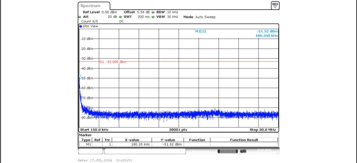
Band4-20MHz-16QAM-20175-1-0-Low-0.15-30--51.52-PASS
