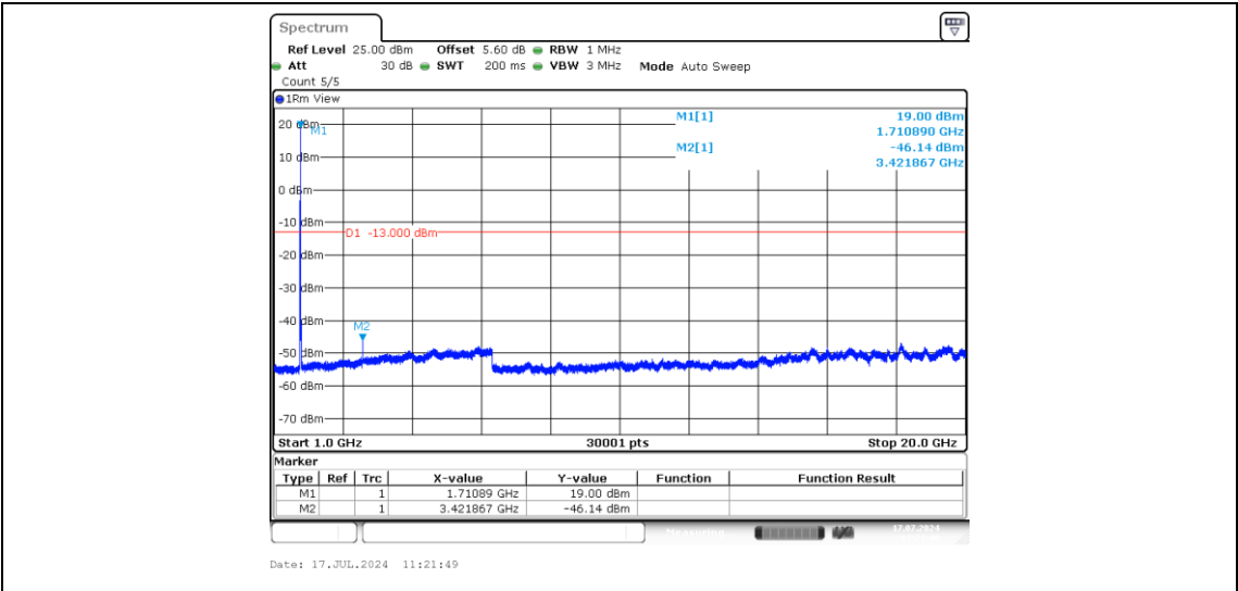
Band4-20MHz-16QAM-20050-1-0-Low-1000-20000--46.14-PASS
