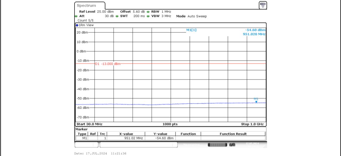
Band4-20MHz-16QAM-20050-1-0-Low-30-1000--54.6-PASS
