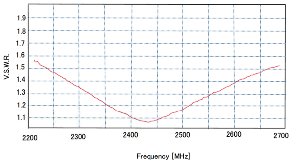
Fig.1 驻波比 VSWR
