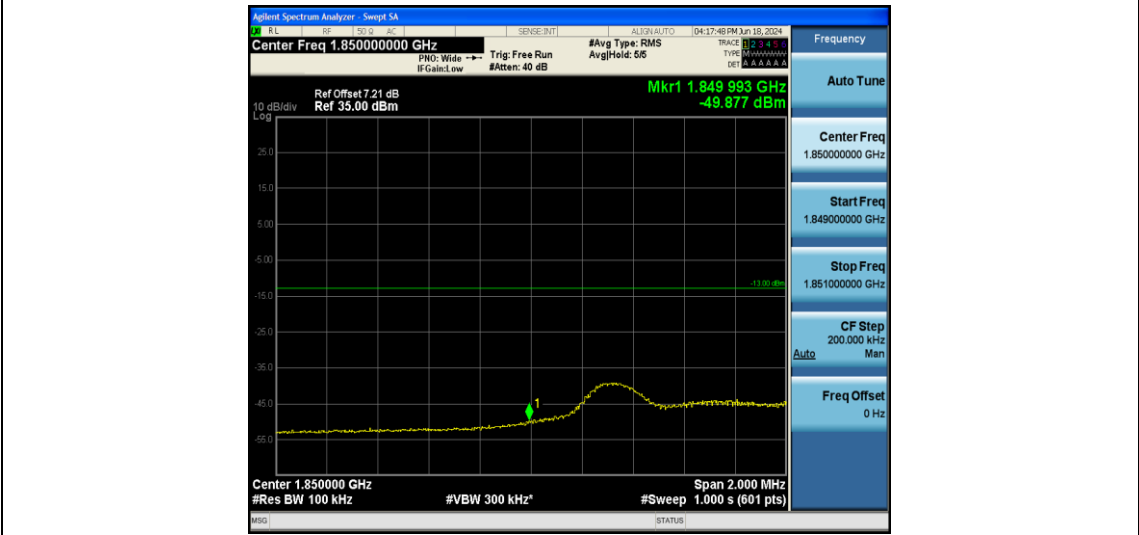
Band2-5MHz-16QAM-18625-25RB#0
