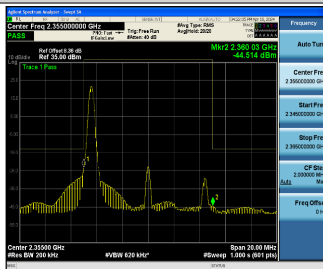
Band40-10MHz-16QAM-39200-1RB#49
