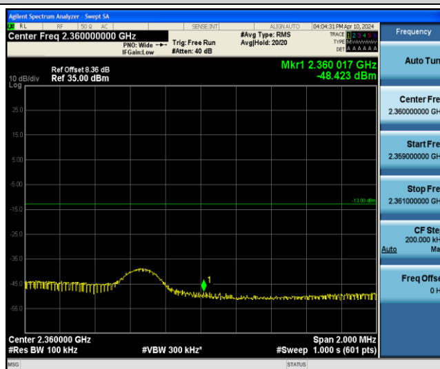
Band40-5MHz-16QAM-39225-1RB#24
