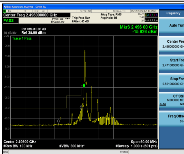
Band41-5MHz-16QAM-39675-1RB#24
