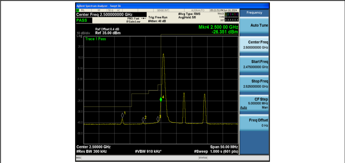
Band7-15MHz-16QAM-20825-1RB#74
