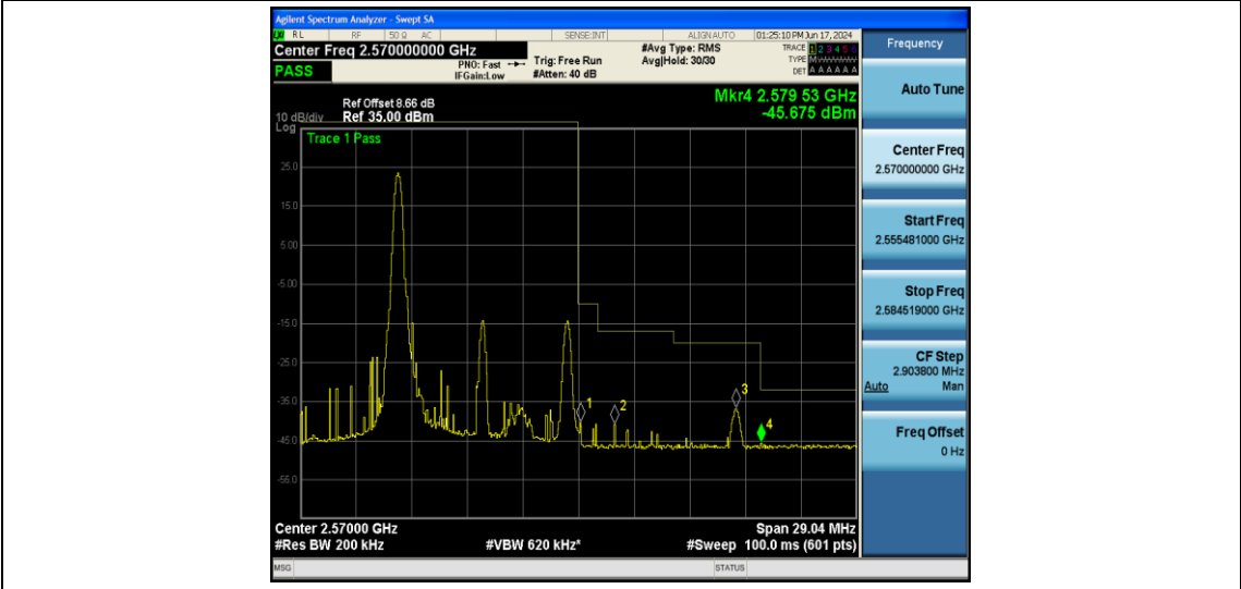
Band7-10MHz-16QAM-21400-1RB#49
