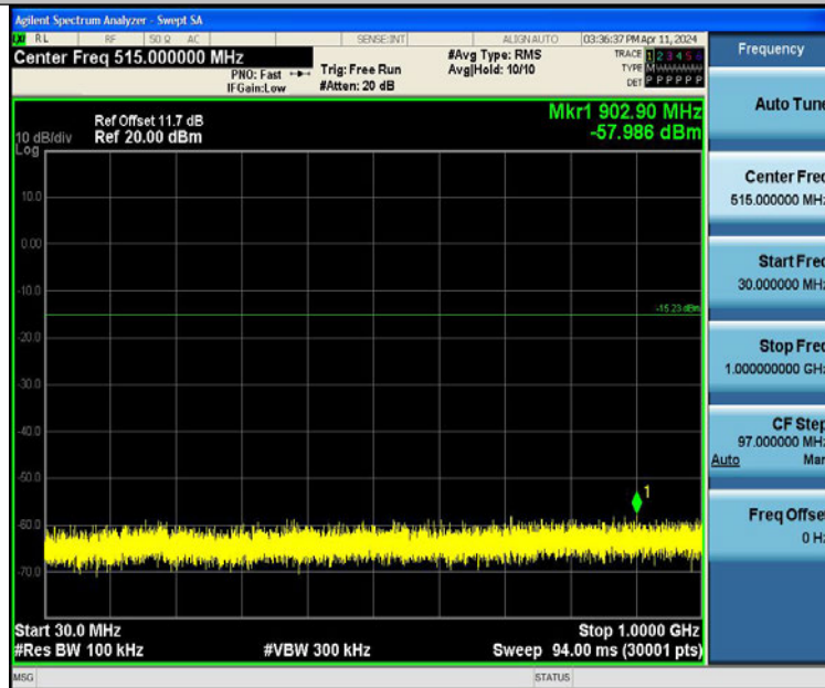
BLE_1M-Ant1-2480-30~1000-PASS
