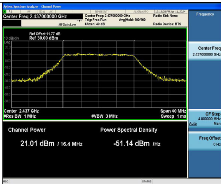
11G-Ant1-2437-PASS
