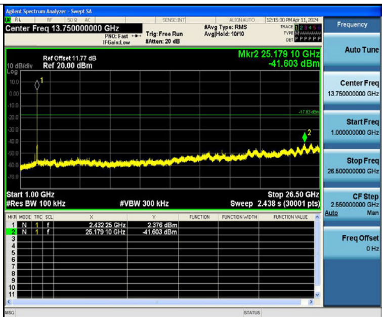
11G-Ant1-2437-1000~26500-PASS
