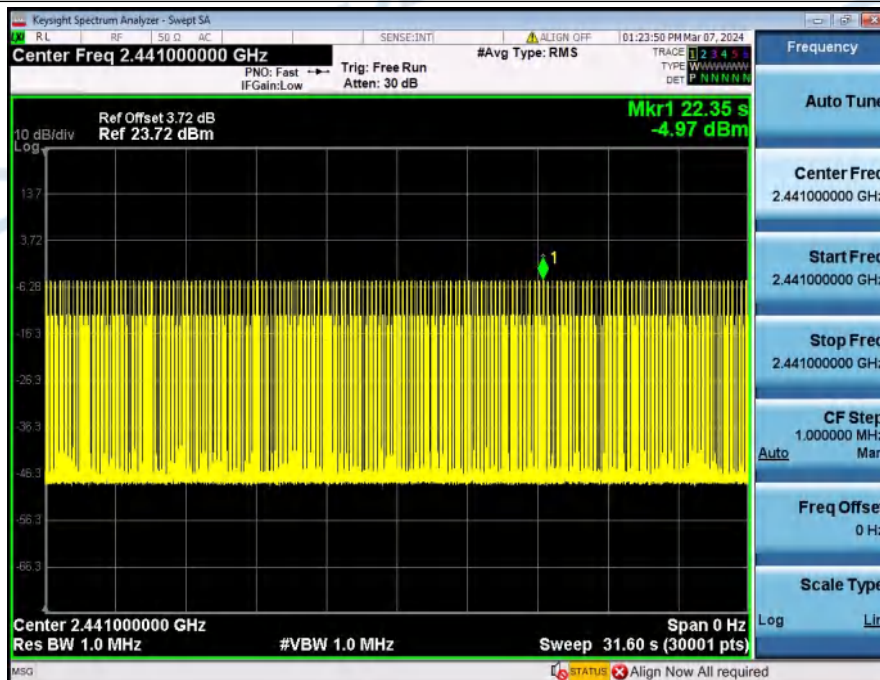
Dwell_Time_(Hopping)_NVNT_ANT1_1-DH1_2441_Accumulated
