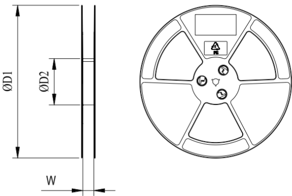
Figure 7-3-2 Tape dimension
