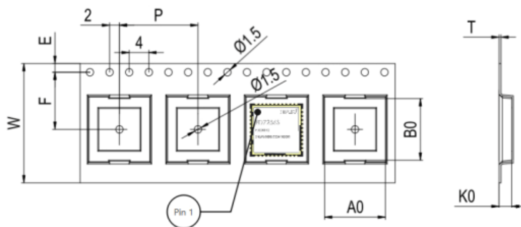
Figure 7-3-1 Tape dimensions
