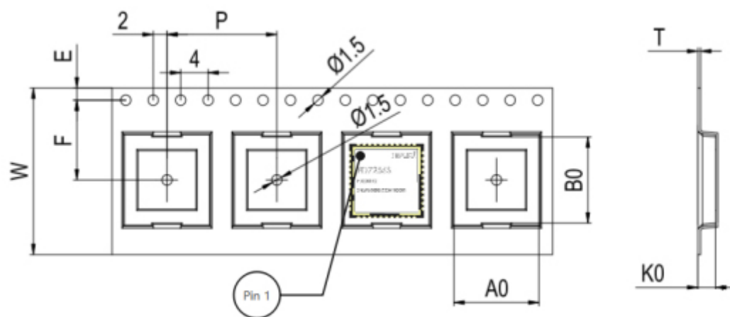
Tape dimensions
