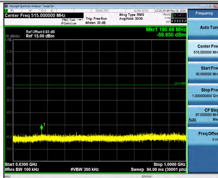
11N20SISO_Ant0_2412_30~1000
