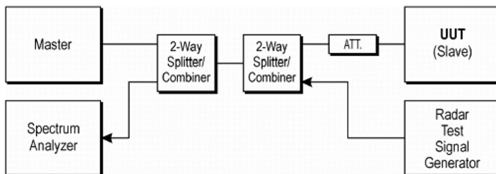
Figure 7-1. Test Setup
