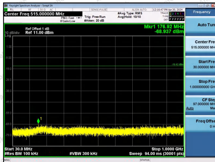
3DH5-Ant0-2480-30~1000-PASS
