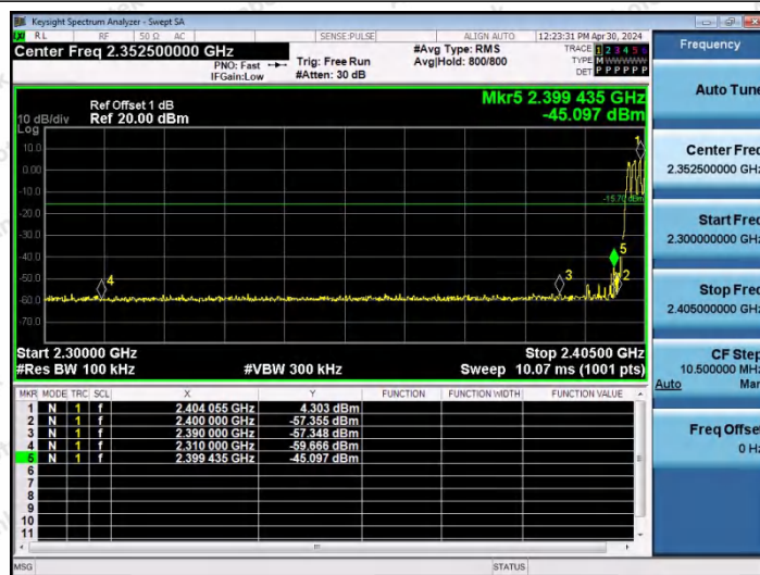
DH5-Ant0-Hop_2402-PASS
