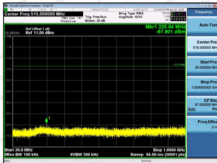
2DH5-Ant0-2402-30~1000-PASS
