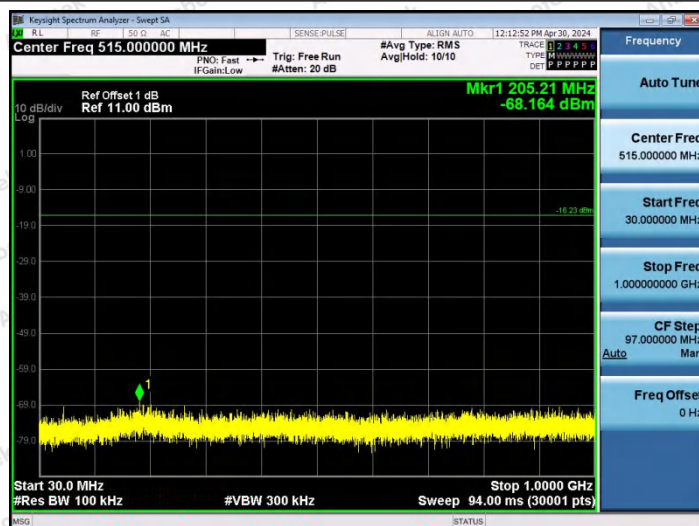
3DH5-Ant0-2402-30~1000-PASS
