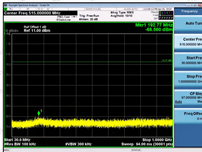
2DH5-Ant0-2441-30~1000-PASS
