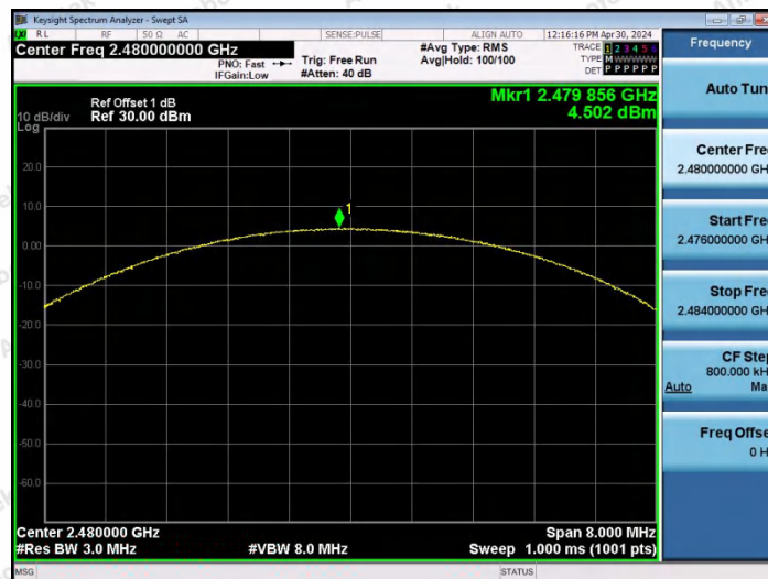
3DH5-Ant0-2480-PASS
