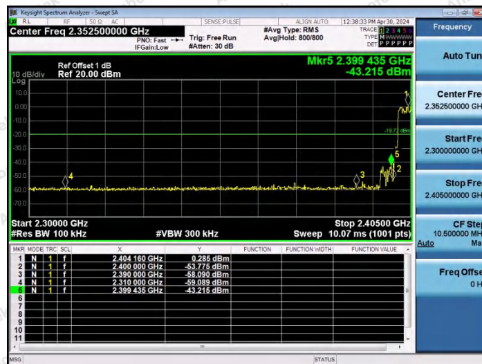
3DH5-Ant0-Hop_2402-PASS
