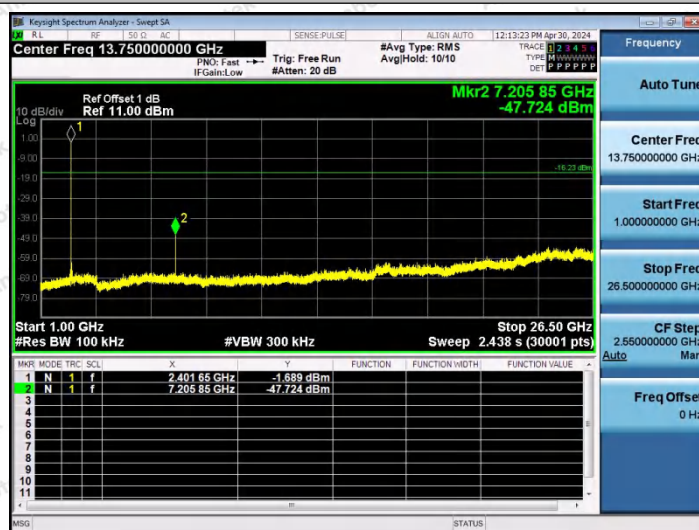
3DH5-Ant0-2402-1000~26500-PASS
