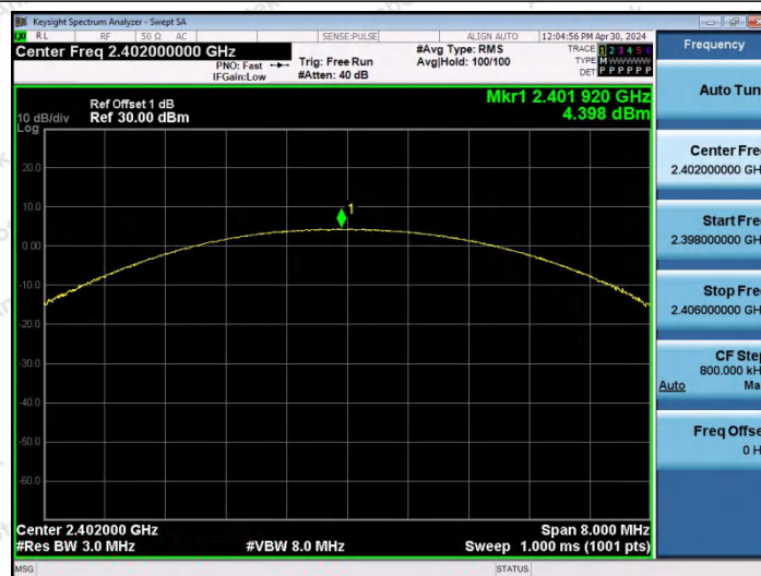
2DH5-Ant0-2402-PASS
