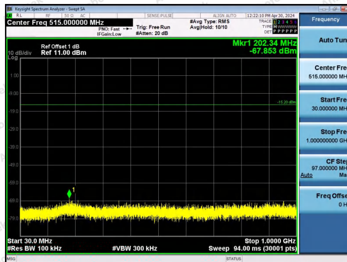
DH5-Ant0-2480-30~1000-PASS
