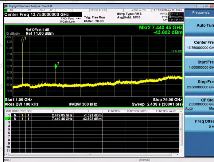
3DH5-Ant0-2480-1000~26500-PASS
