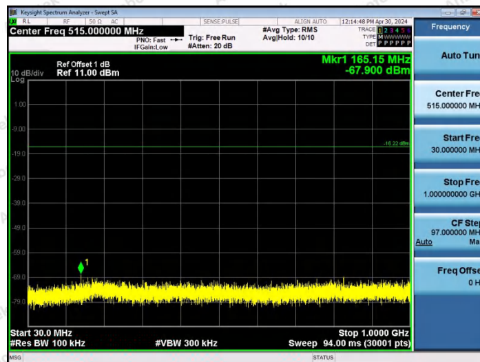
3DH5-Ant0-2441-30~1000-PASS
