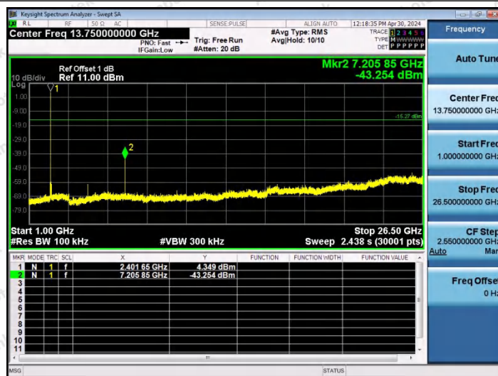
DH5-Ant0-2402-1000~26500-PASS
