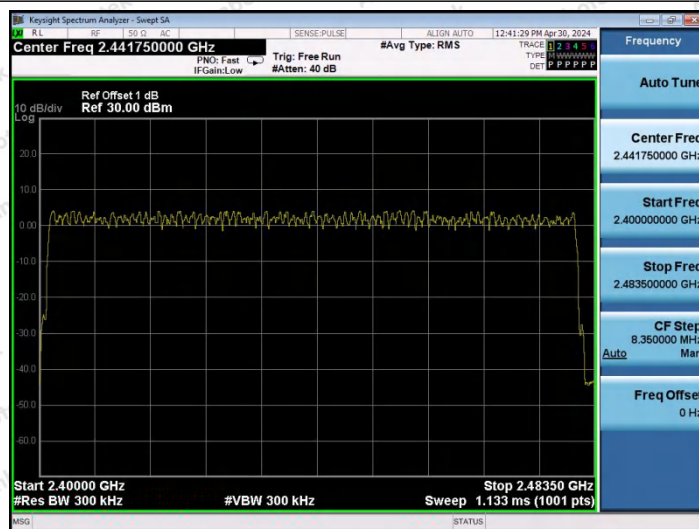
3DH5-Ant0-Hop-PASS
