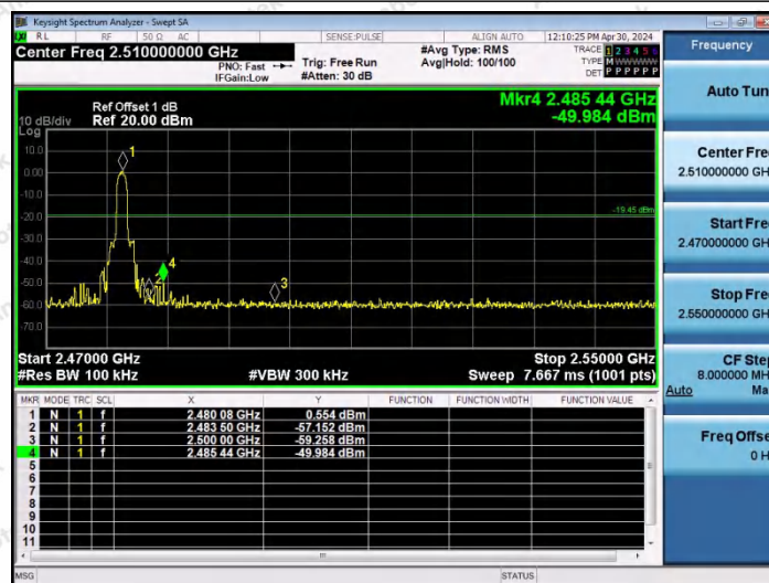
2DH5-Ant0-2480-PASS
