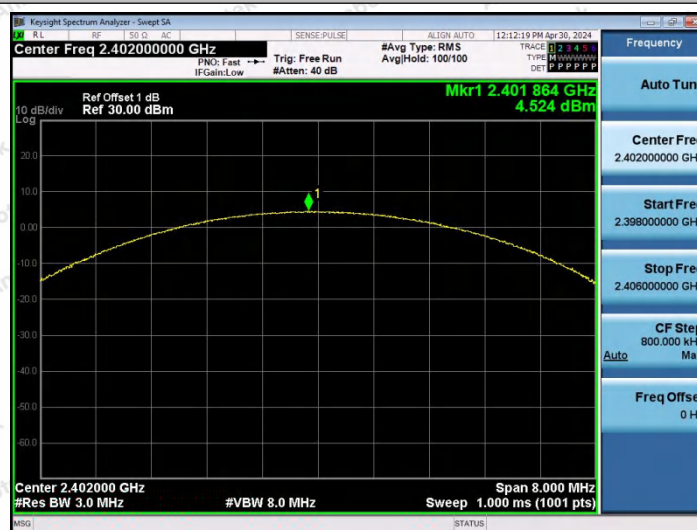
3DH5-Ant0-2402-PASS
