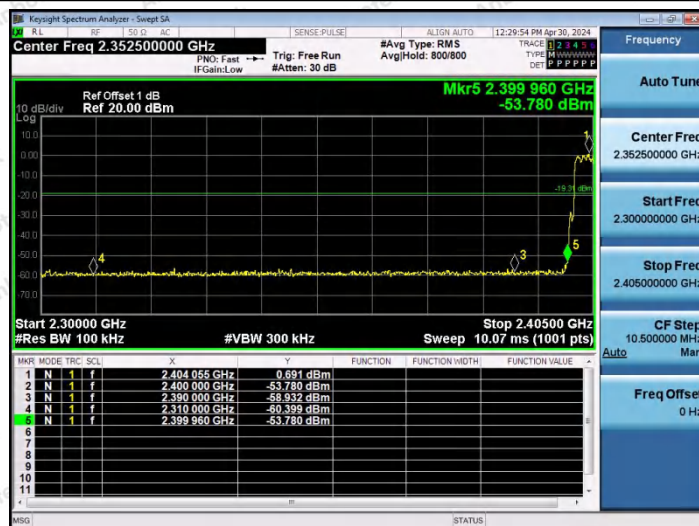
2DH5-Ant0-Hop_2402-PASS
