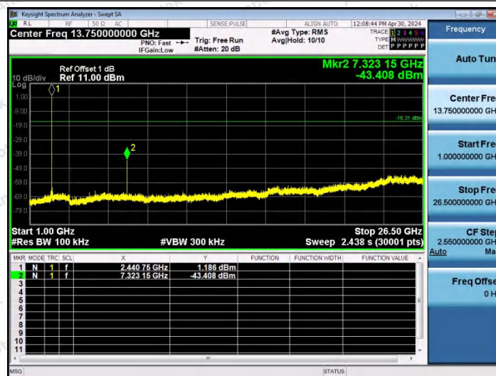
2DH5-Ant0-2441-1000~26500-PASS
