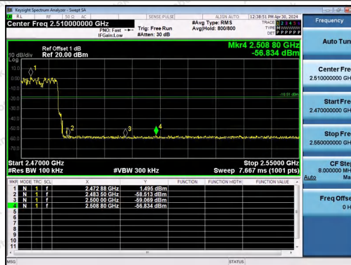
3DH5-Ant0-Hop_2480-PASS
