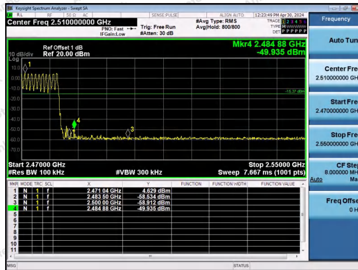
DH5-Ant0-Hop_2480-PASS
