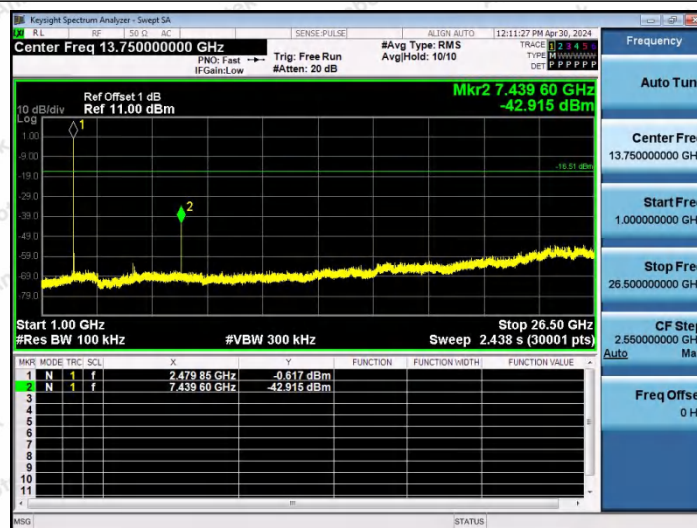
2DH5-Ant0-2480-1000~26500-PASS
