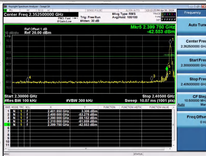
3DH5-Ant0-2402-PASS
