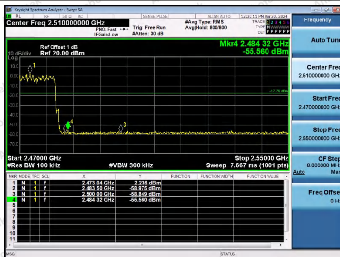
2DH5-Ant0-Hop_2480-PASS
