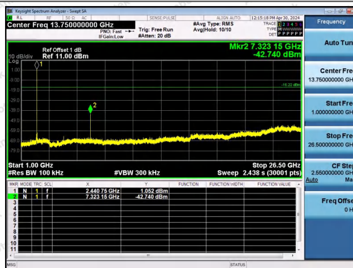
3DH5-Ant0-2441-1000~26500-PASS
