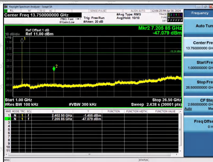
2DH5-Ant0-2402-1000~26500-PASS
