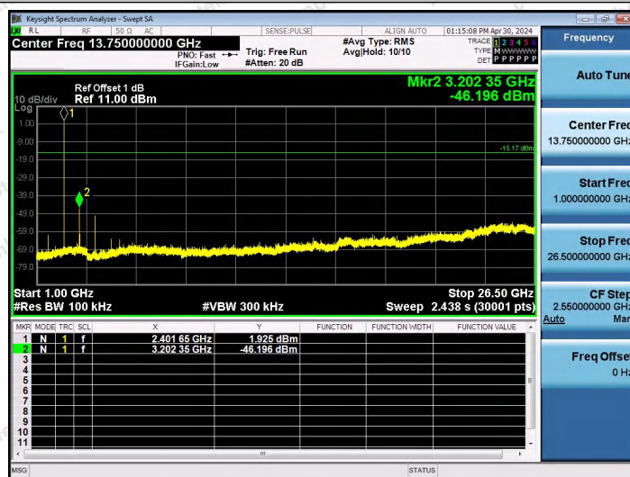
BLE_2M-Ant0-2402-1000~26500-PASS
