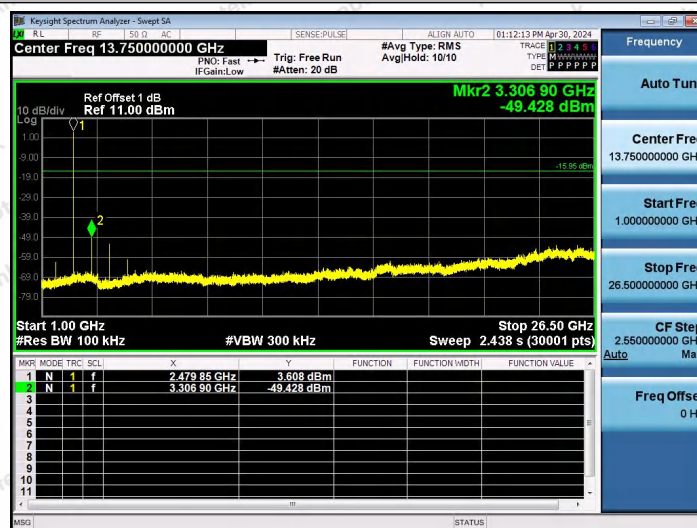
BLE_1M-Ant0-2480-1000~26500-PASS
