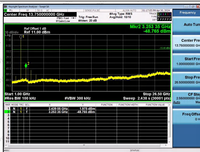
BLE_2M-Ant0-2440-1000~26500-PASS
