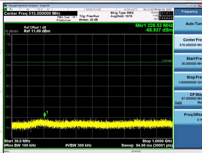
BLE_1M-Ant0-2480-30~1000-PASS
