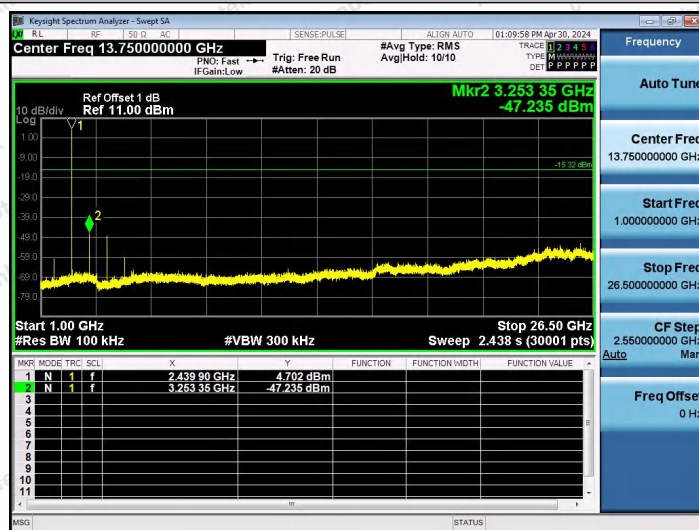
BLE_1M-Ant0-2440-1000~26500-PASS
