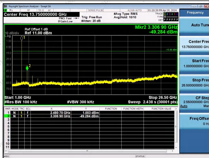
BLE_2M-Ant0-2480-1000~26500-PASS
