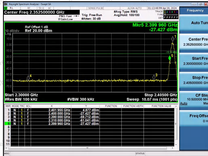
BLE_2M-Ant0-2402-PASS
