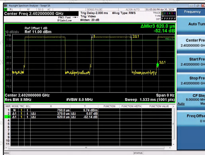
NTNV-BLE_1M-Ant0-2402
