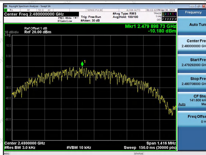
BLE_1M-Ant0-2480-PASS
