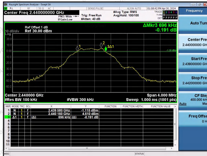
BLE_1M-Ant0-2440-PASS
