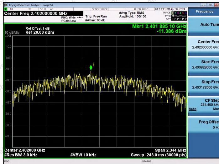
BLE_2M-Ant0-2402-PASS
