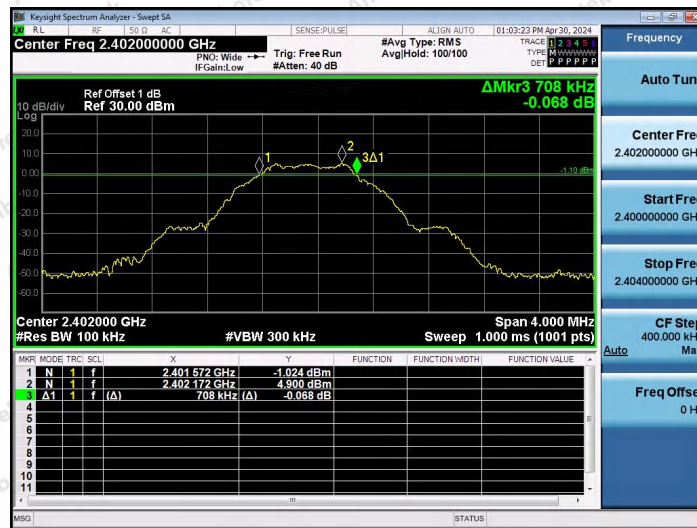
BLE_1M-Ant0-2402-PASS
