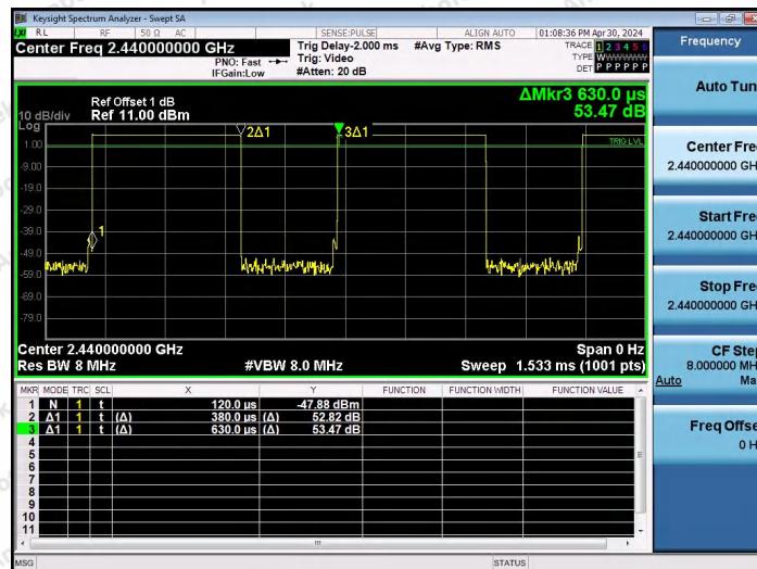
NTNV-BLE_1M-Ant0-2440
