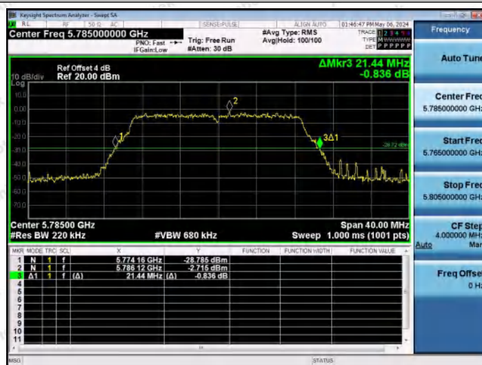
11AC20MIMO-Ant0-5785
