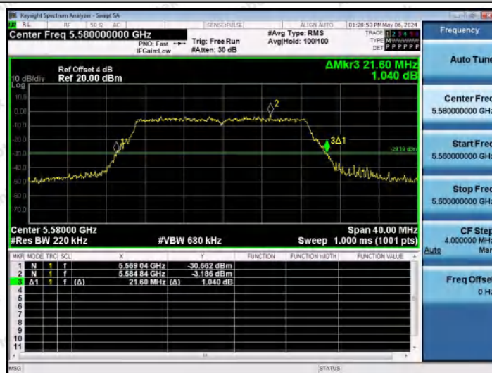
11N20MIMO-Ant0-5580
