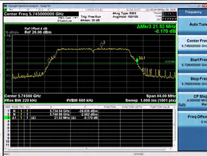
11AC20MIMO-Ant1-5745
