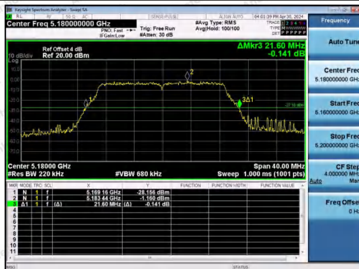
11N20MIMO-Ant0-5180
