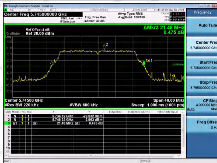
11AC20MIMO-Ant0-5745
