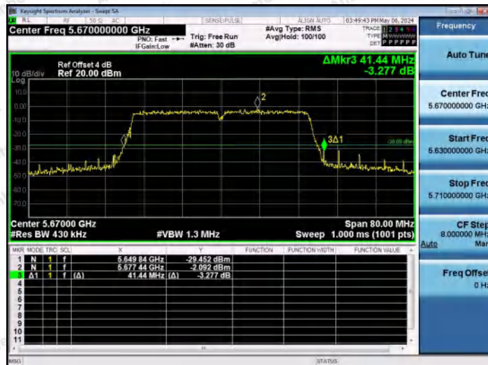
11AC40MIMO-Ant0-5670
