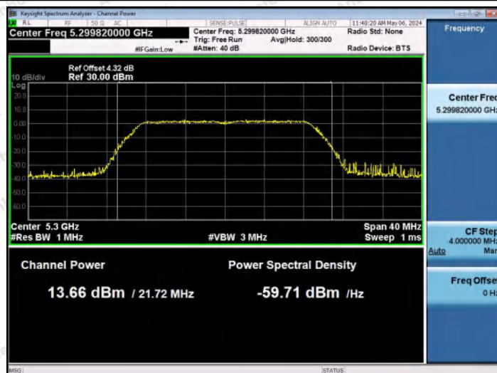
11N20MIMO-Ant1-5300-PASS
