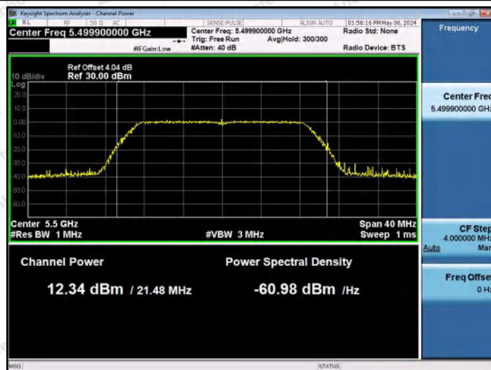
11AC20MIMO-Ant0-5500-PASS
