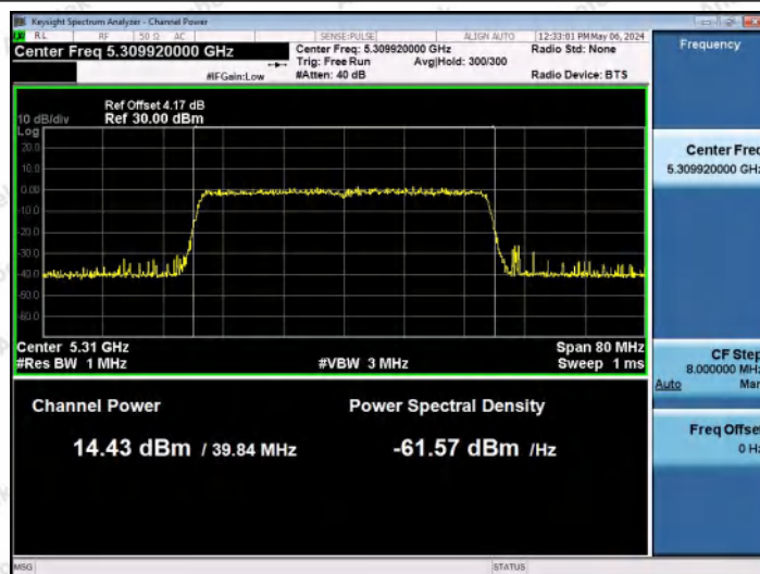
11AX40MIMO-Ant0-5310-PASS
