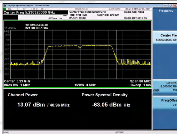
11AC40MIMO-Ant0-5230-PASS
