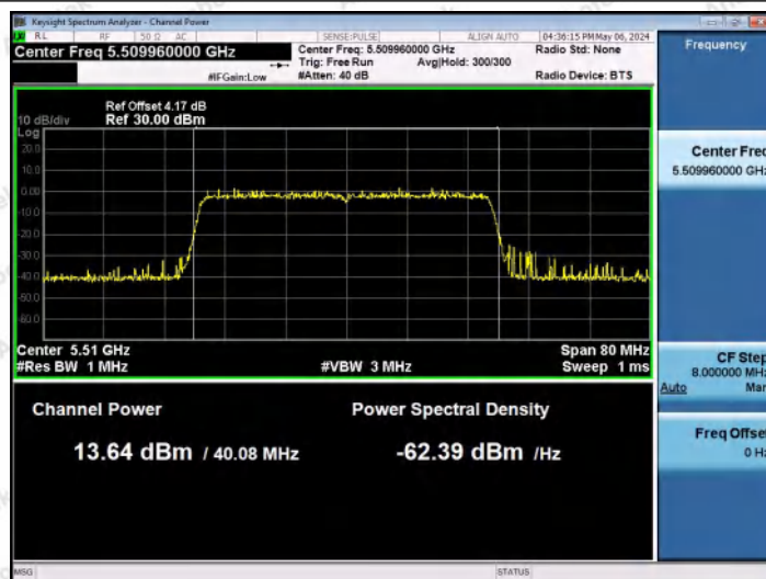
11AX40MIMO-Ant1-5510-PASS
