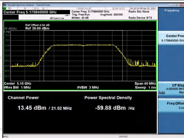
11AC20MIMO-Ant0-5180-PASS
