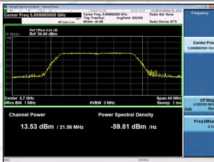
11AC20MIMO-Ant1-5700-PASS
