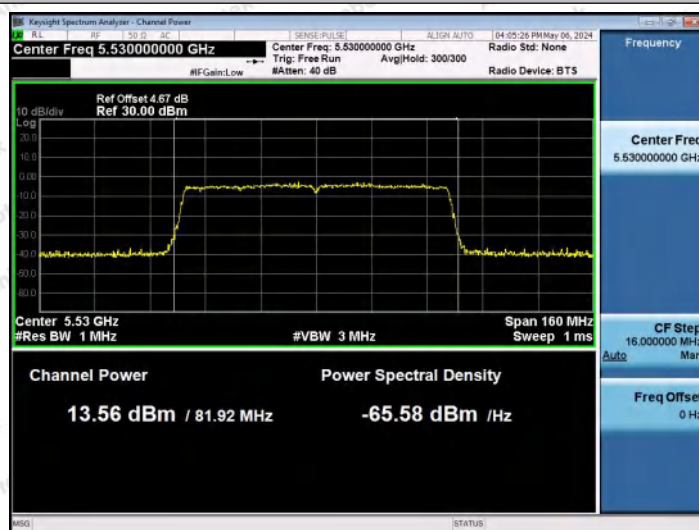
11AC80MIMO-Ant1-5530-PASS
