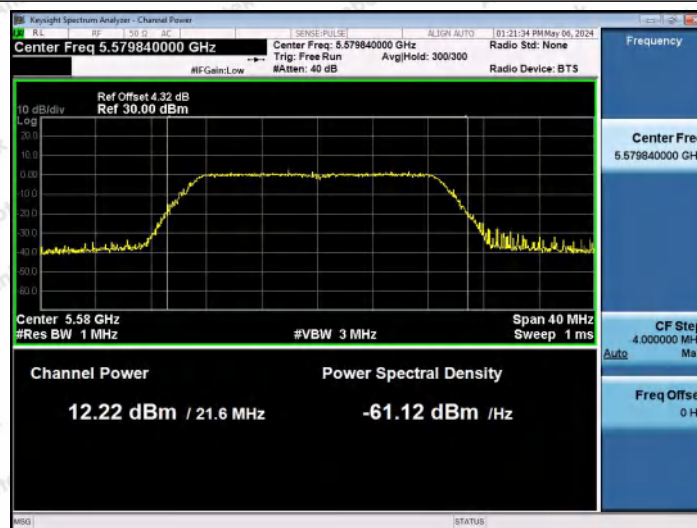
11N20MIMO-Ant0-5580-PASS
