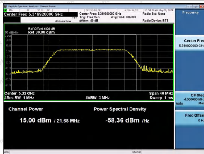
11AC20MIMO-Ant1-5320-PASS
