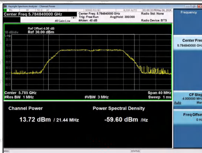
11A-Ant1-5785-PASS
