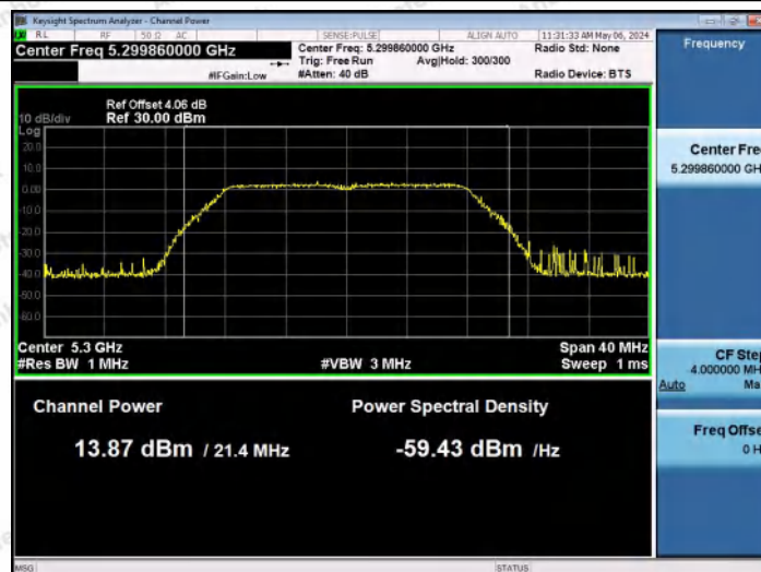
11A-Ant1-5300-PASS
