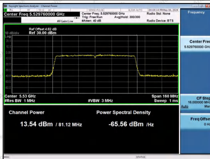
11AC80MIMO-Ant0-5530-PASS
