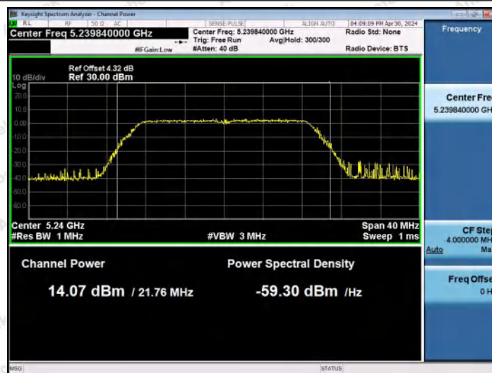
11N20MIMO-Ant0-5240-PASS
