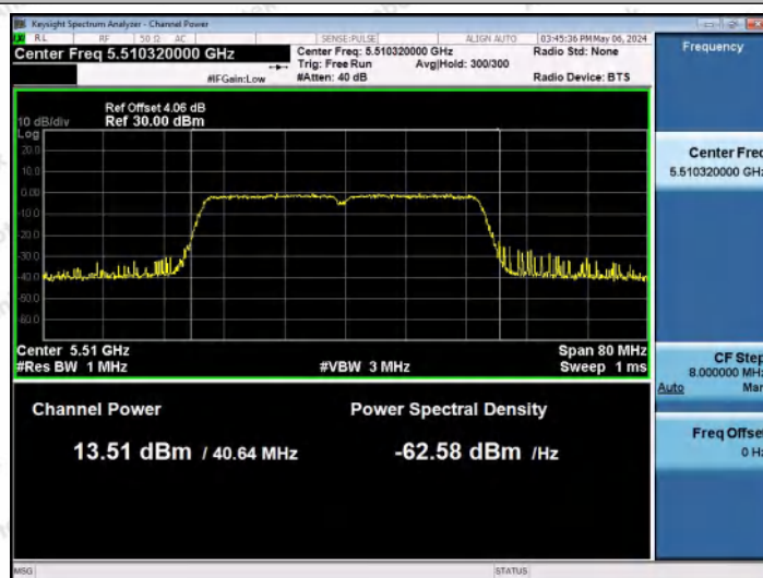
11AC40MIMO-Ant0-5510-PASS
