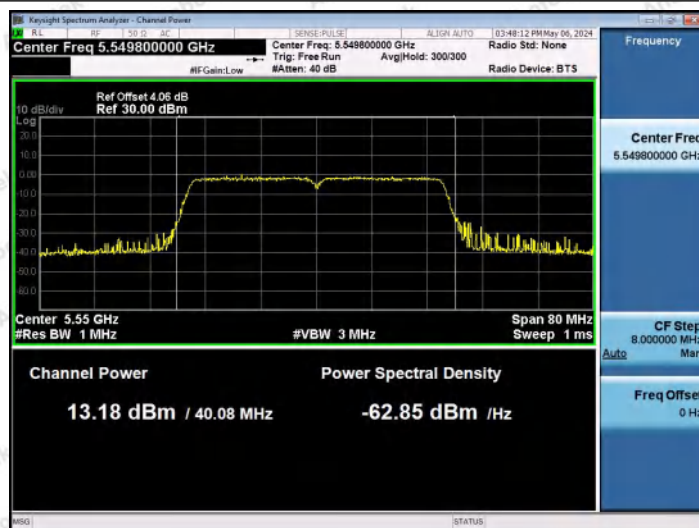
11AC40MIMO-Ant0-5550-PASS
