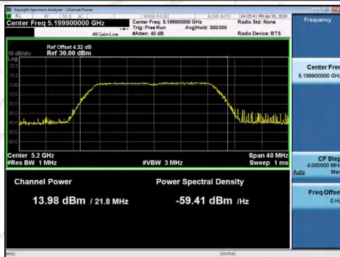
11N20MIMO-Ant0-5200-PASS
