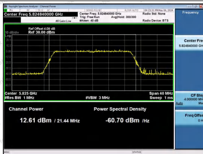
11AX20MIMO-Ant0-5825-PASS
