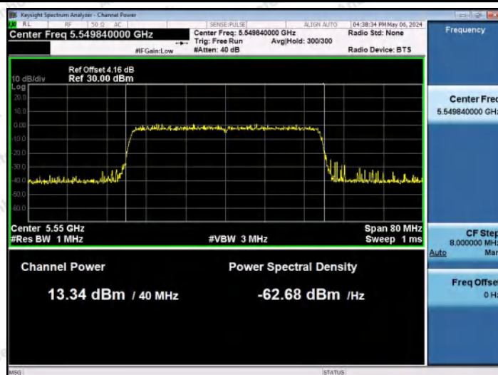
11AX40MIMO-Ant1-5550-PASS
