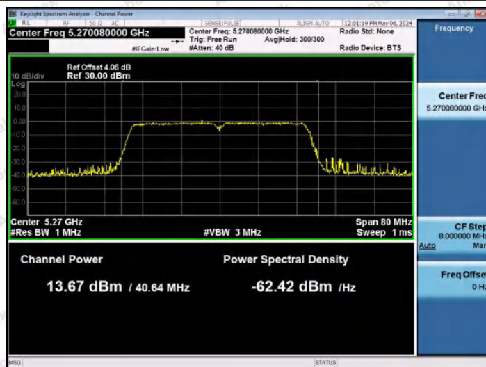
11AC40MIMO-Ant0-5270-PASS
