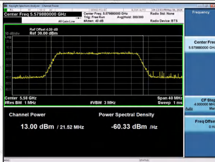
11AX20MIMO-Ant0-5580-PASS
