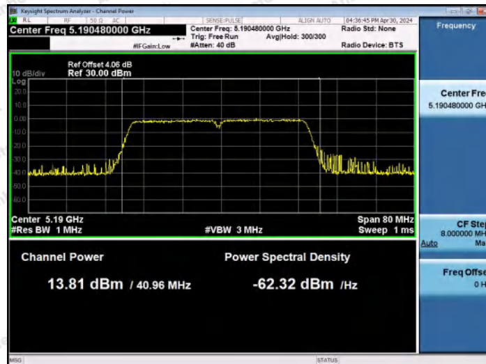
11AC40MIMO-Ant0-5190-PASS
