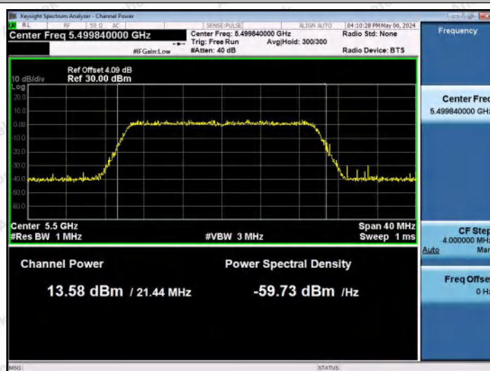
11AX20MIMO-Ant0-5500-PASS
