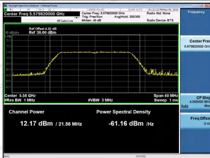
11N20MIMO-Ant1-5580-PASS
