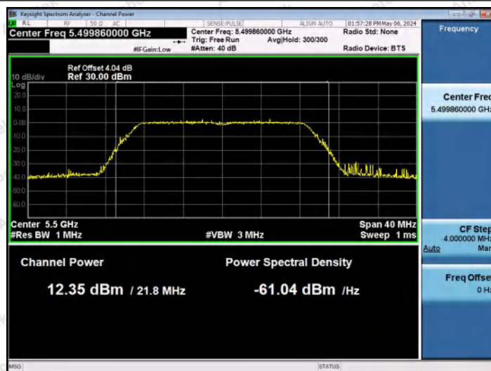
11AC20MIMO-Ant1-5500-PASS
