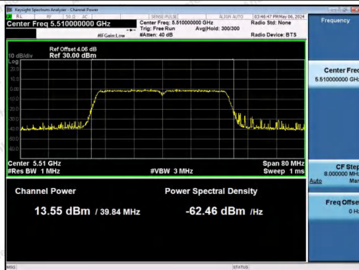
11AC40MIMO-Ant1-5510-PASS
