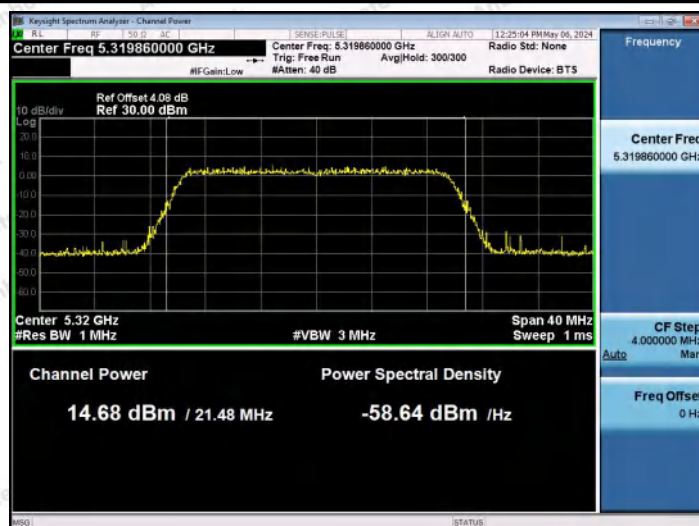
11AX20MIMO-Ant1-5320-PASS
