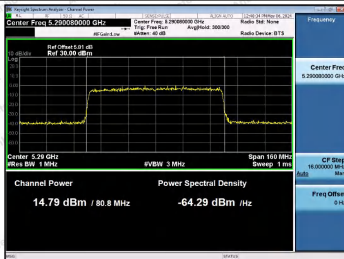
11AX80MIMO-Ant0-5290-PASS
