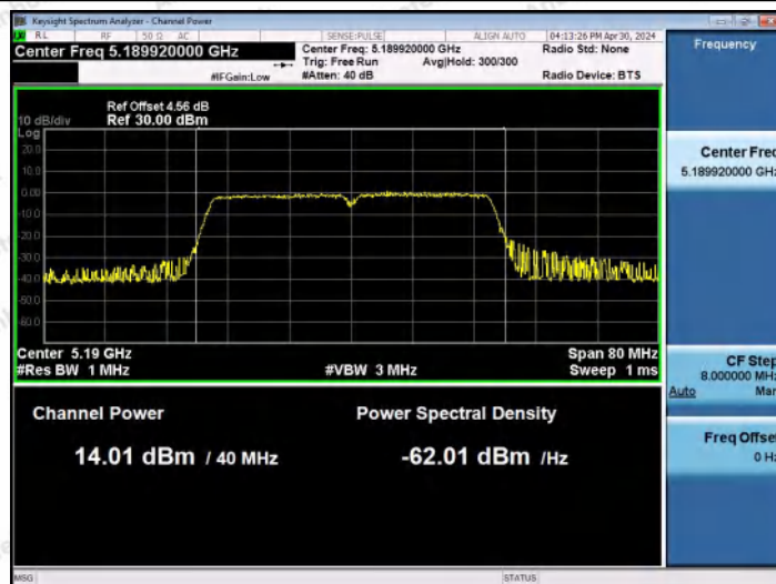
11N40MIMO-Ant0-5190-PASS
