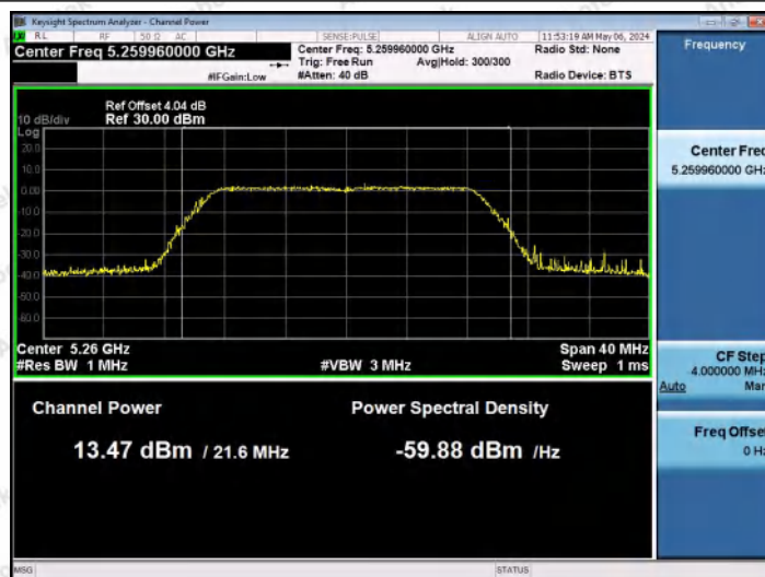
11AC20MIMO-Ant1-5260-PASS
