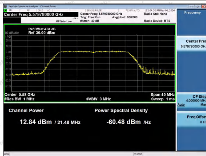
11AC20MIMO-Ant0-5580-PASS
