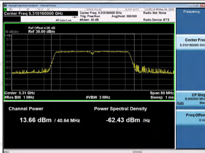
11AC40MIMO-Ant0-5310-PASS
