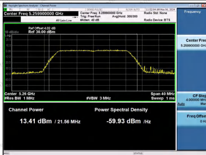
11AC20MIMO-Ant0-5260-PASS
