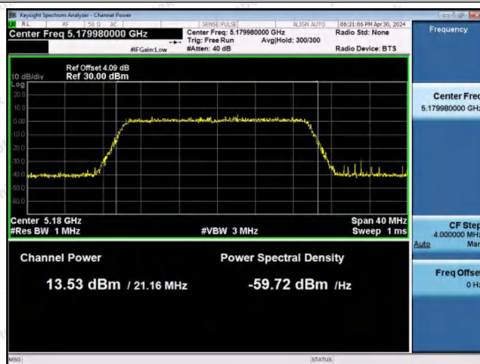
11AX20MIMO-Ant1-5180-PASS
