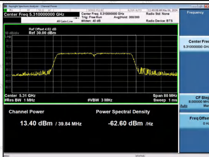
11N40MIMO-Ant0-5310-PASS
