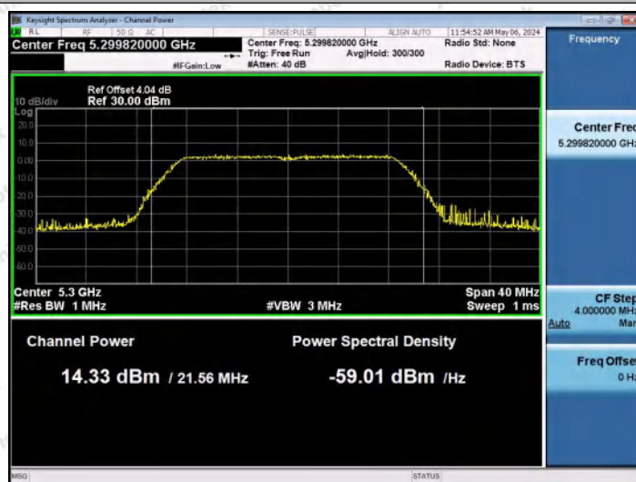
11AC20MIMO-Ant0-5300-PASS
