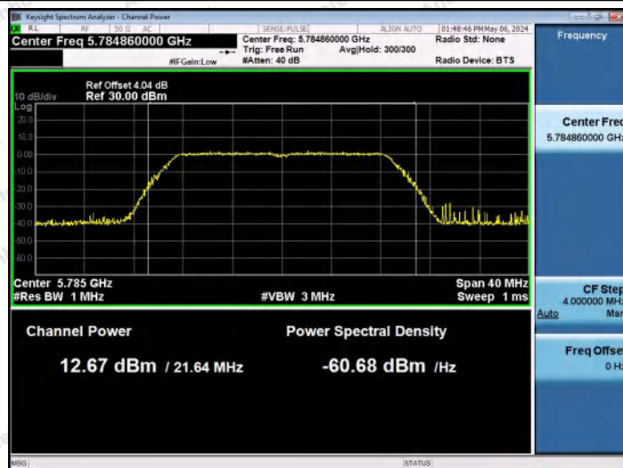
11AC20MIMO-Ant1-5785-PASS
