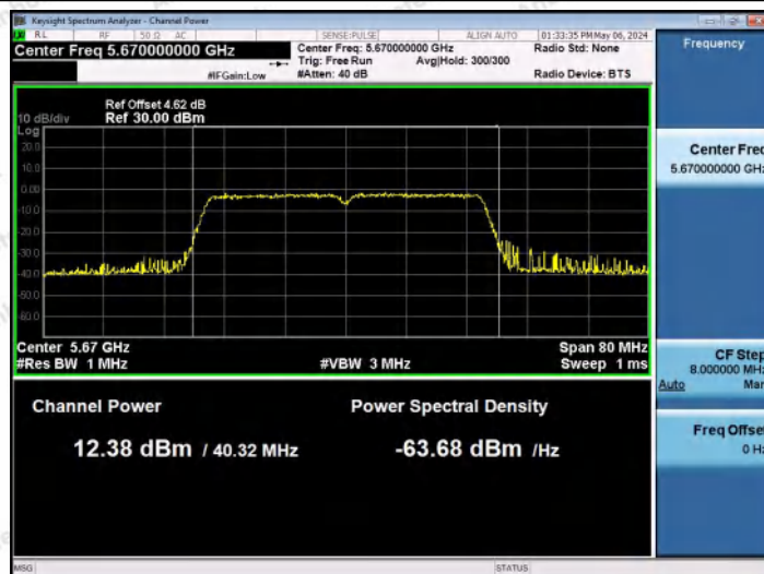
11N40MIMO-Ant0-5670-PASS
