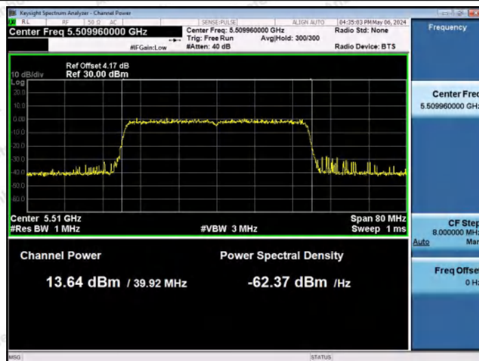
11AX40MIMO-Ant0-5510-PASS
