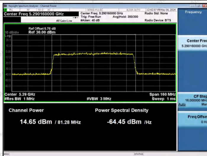
11AX80MIMO-Ant1-5290-PASS
