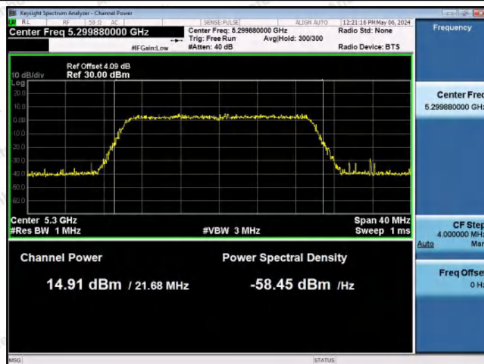
11AX20MIMO-Ant0-5300-PASS
