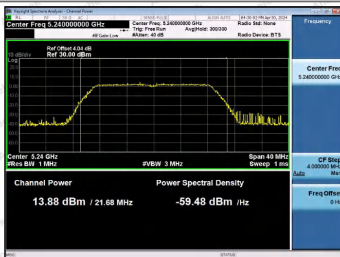
11AC20MIMO-Ant0-5240-PASS
