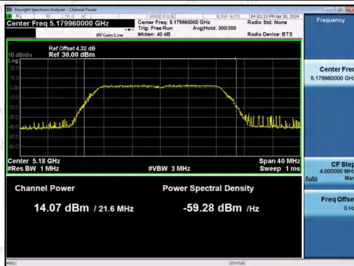
11N20MIMO-Ant0-5180-PASS
