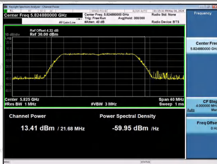
11N20MIMO-Ant1-5825-PASS
