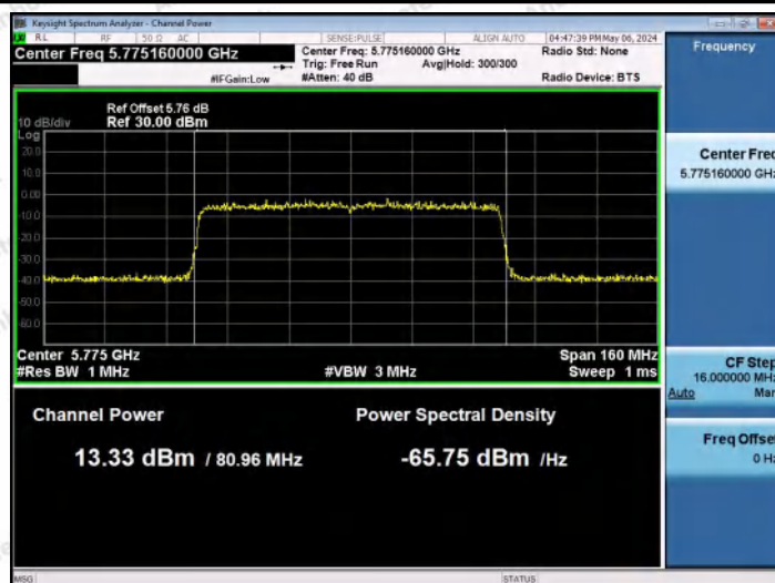
11AX80MIMO-Ant0-5775-PASS
