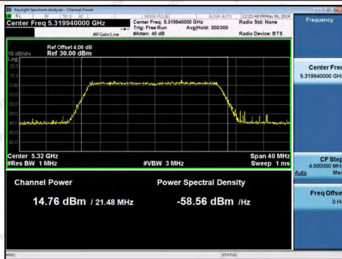
11AX20MIMO-Ant0-5320-PASS
