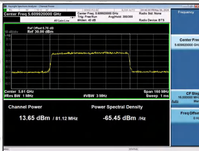
11AX80MIMO-Ant1-5610-PASS
