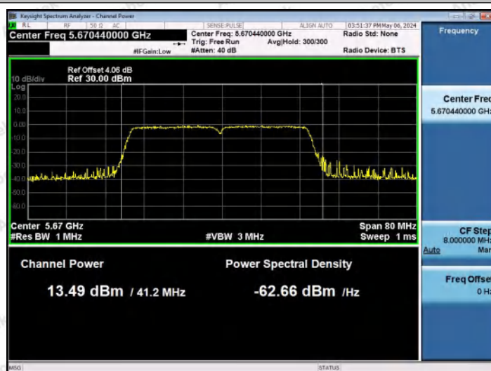
11AC40MIMO-Ant1-5670-PASS
