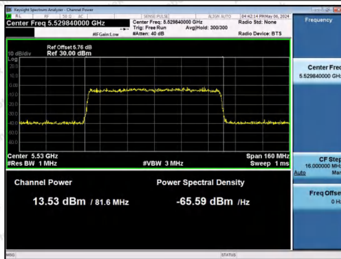
11AX80MIMO-Ant0-5530-PASS
