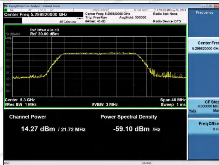
11AC20MIMO-Ant1-5300-PASS
