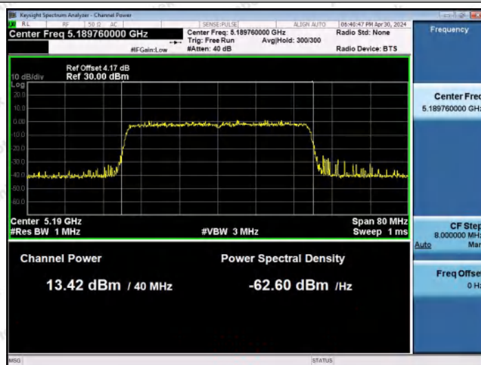
11AX40MIMO-Ant1-5190-PASS
