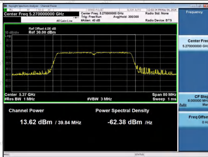
11AC40MIMO-Ant1-5270-PASS
