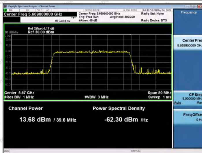
11AX40MIMO-Ant1-5670-PASS
