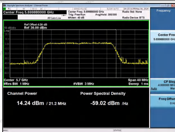
11AX20MIMO-Ant0-5700-PASS
