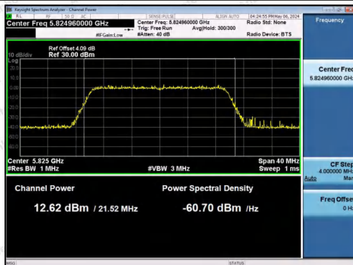
11AX20MIMO-Ant1-5825-PASS
