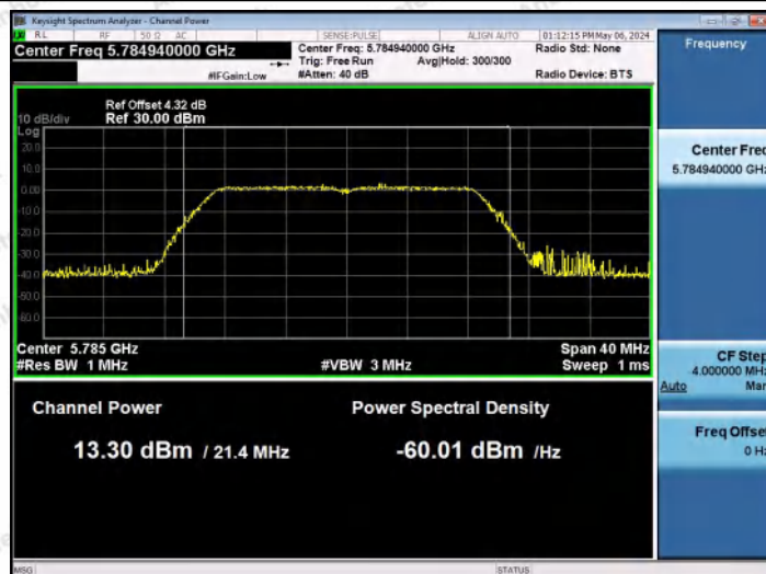
11N20MIMO-Ant1-5785-PASS
