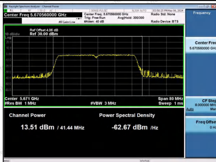
11AC40MIMO-Ant0-5670-PASS
