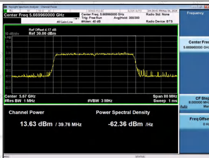
11AX40MIMO-Ant0-5670-PASS
