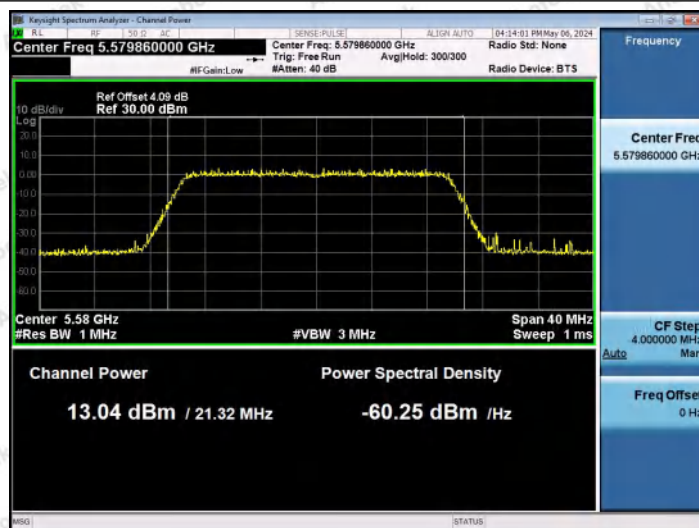
11AX20MIMO-Ant1-5580-PASS
