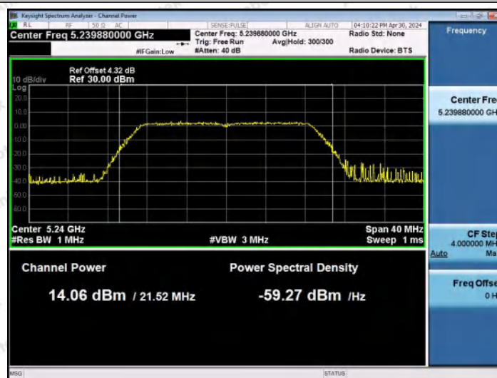
11N20MIMO-Ant1-5240-PASS
