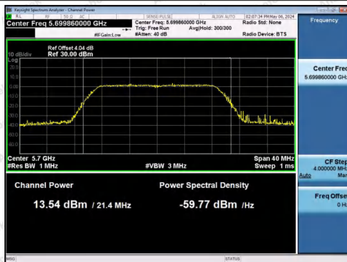
11AC20MIMO-Ant0-5700-PASS
