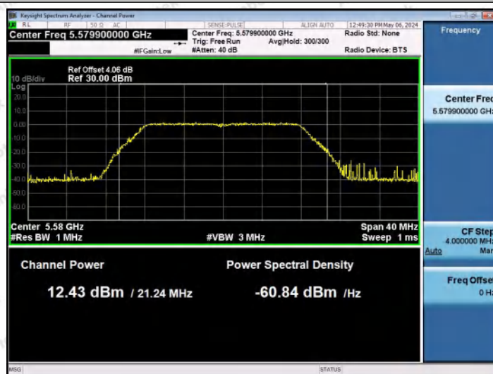
11A-Ant0-5580-PASS
