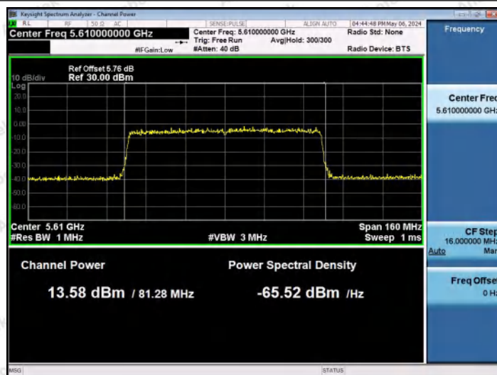
11AX80MIMO-Ant0-5610-PASS
