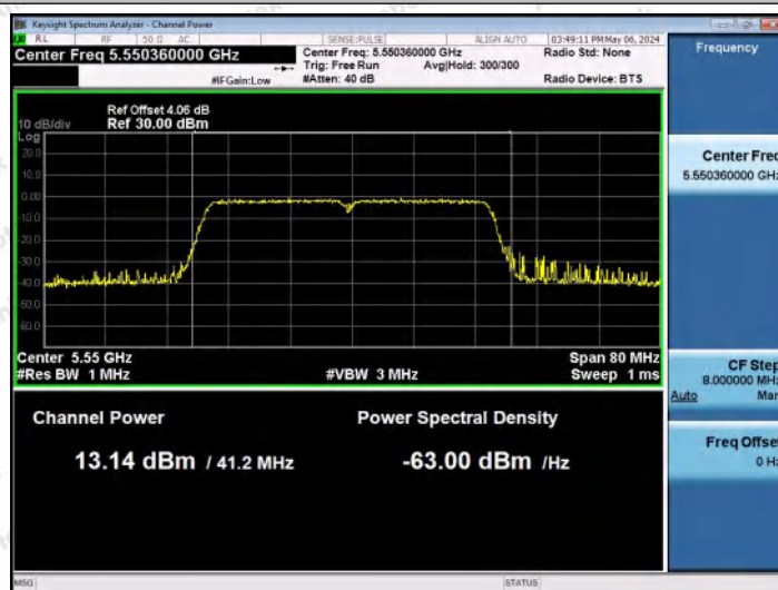
11AC40MIMO-Ant1-5550-PASS
