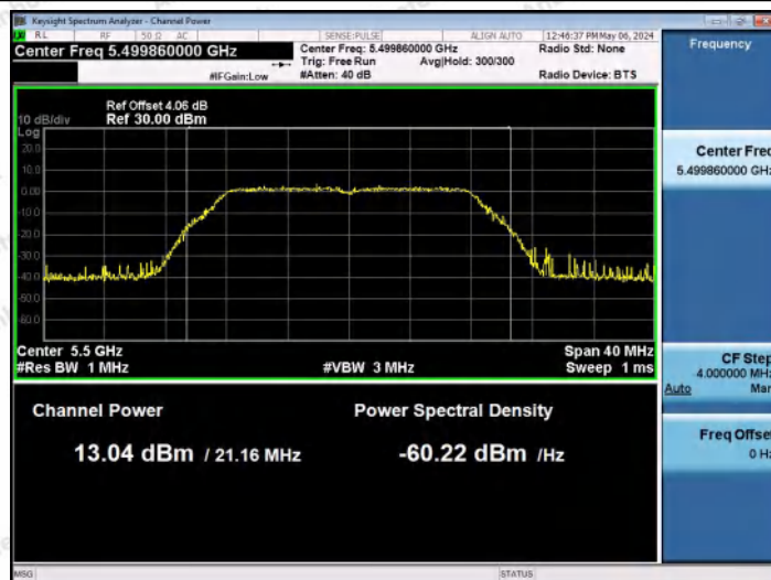
11A-Ant0-5500-PASS
