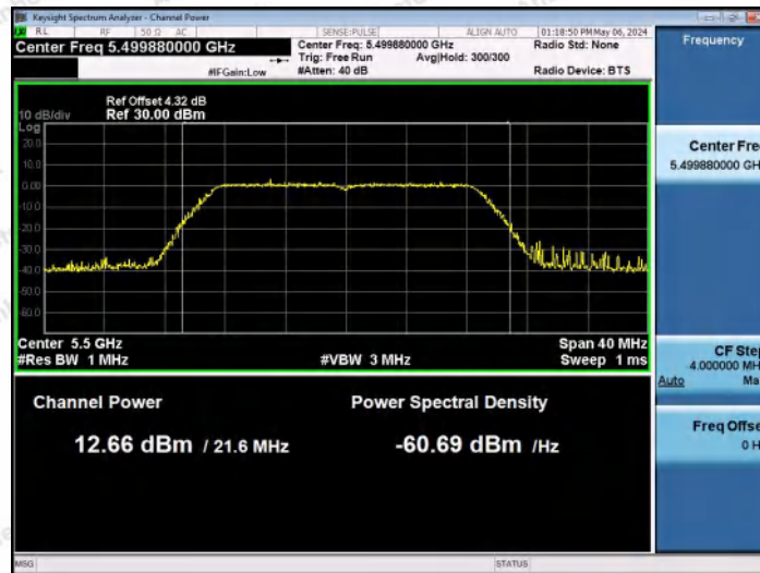
11N20MIMO-Ant0-5500-PASS
