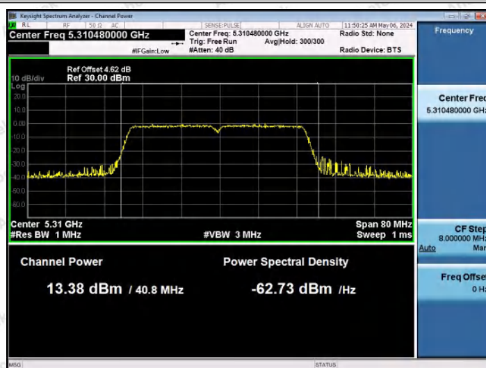
11N40MIMO-Ant1-5310-PASS
