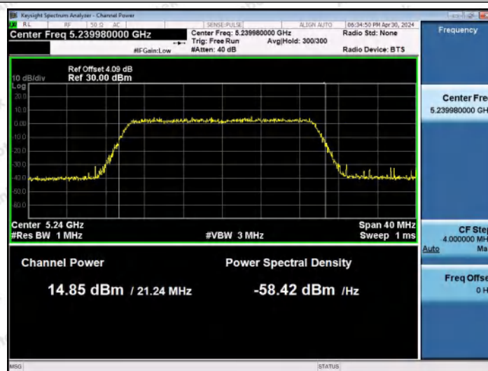
11AX20MIMO-Ant0-5240-PASS
