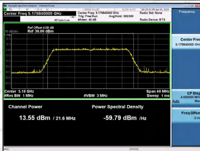
11AX20MIMO-Ant0-5180-PASS
