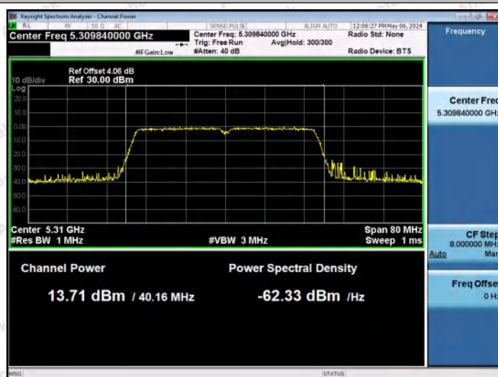
11AC40MIMO-Ant1-5310-PASS
