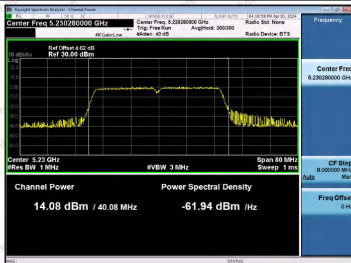
11N40MIMO-Ant1-5230-PASS
