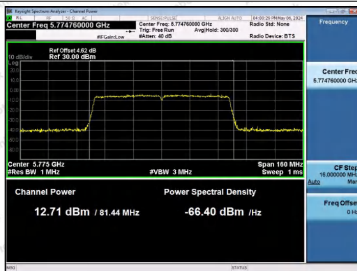
11AC80MIMO-Ant0-5775-PASS
