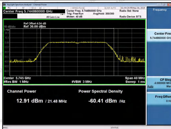
11AC20MIMO-Ant0-5745-PASS
