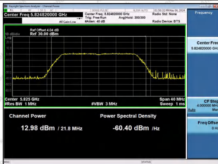
11AC20MIMO-Ant0-5825-PASS
