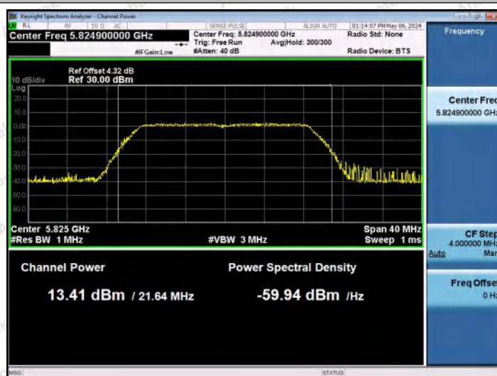
11N20MIMO-Ant0-5825-PASS
