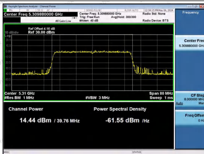
11AX40MIMO-Ant1-5310-PASS
