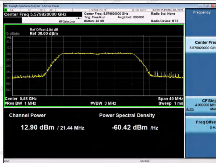
11AC20MIMO-Ant1-5580-PASS
