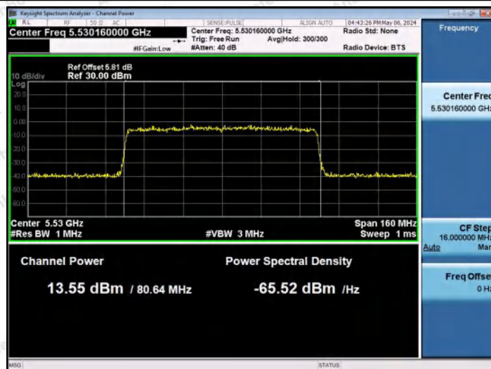
11AX80MIMO-Ant1-5530-PASS
