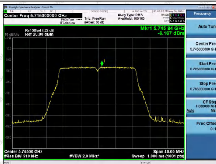
11N20MIMO-Ant0-5745-PASS
