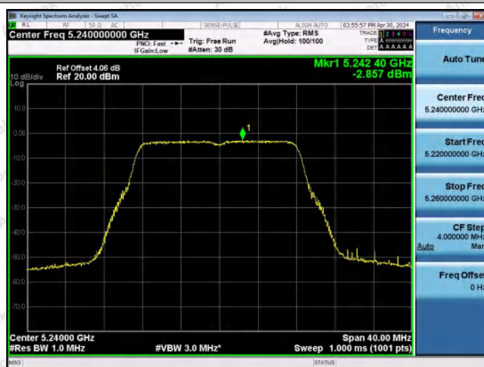
11A-Ant0-5240-PASS
