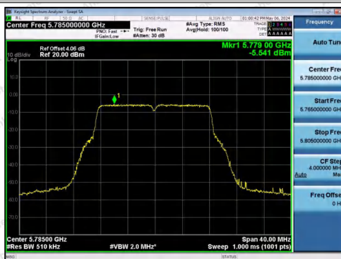
11A-Ant1-5785-PASS
