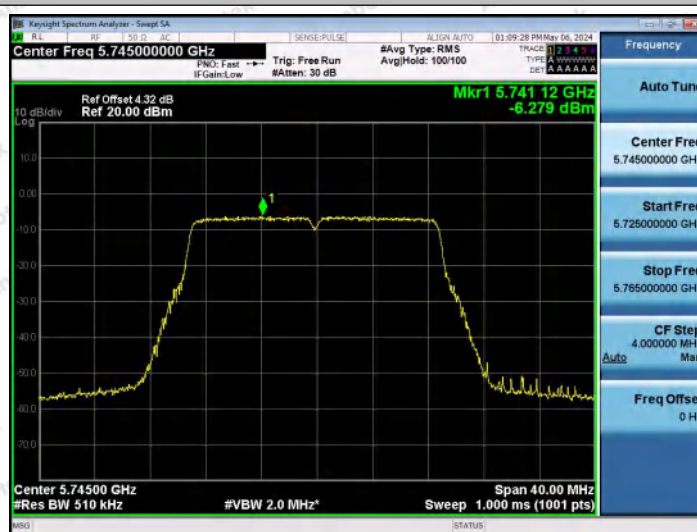
11N20MIMO-Ant1-5745-PASS
