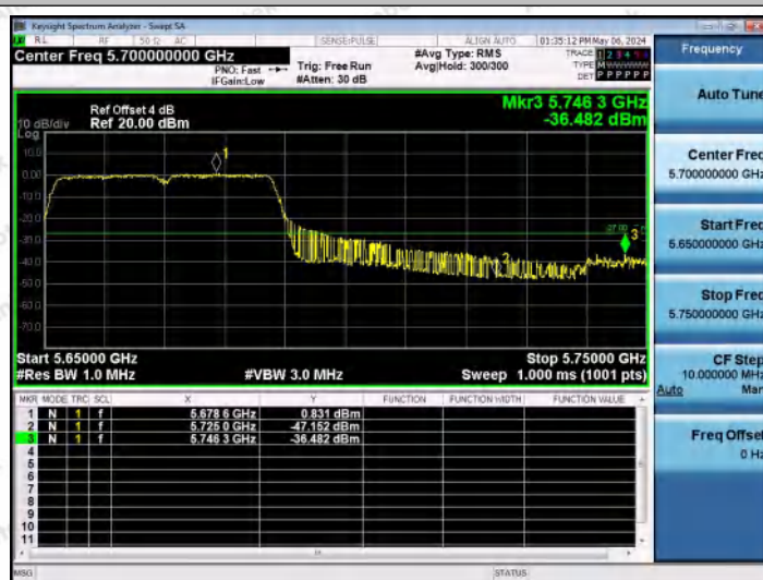
11N40MIMO-Ant1-5670-PASS
