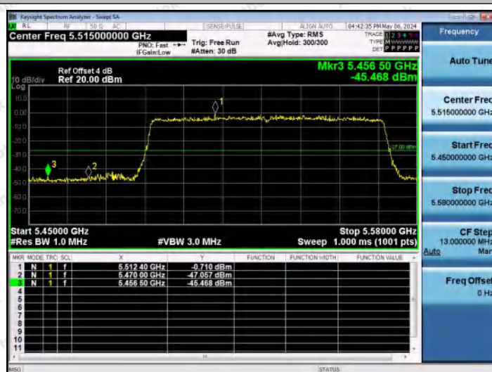
11AX80MIMO-Ant0-5530-PASS
