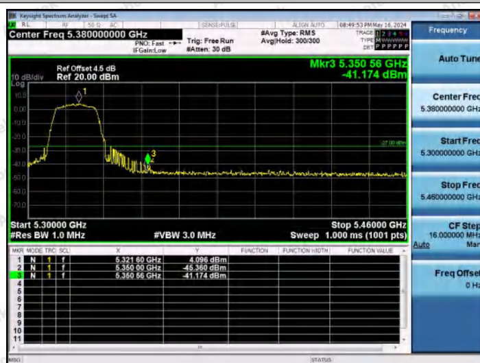
11N20MIMO-Ant1-5320-PASS
