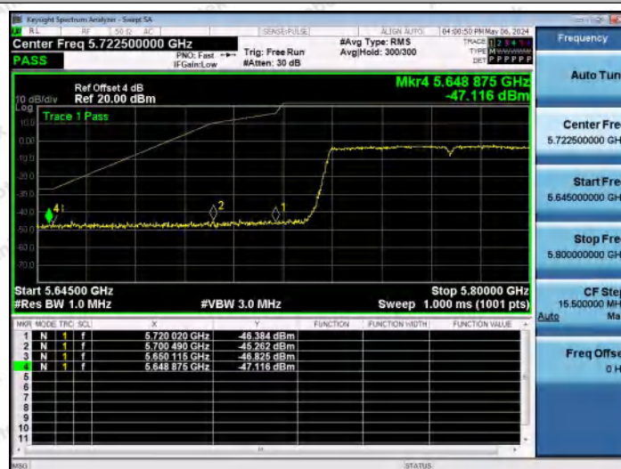
11AC80MIMO-Ant0-5775-PASS
