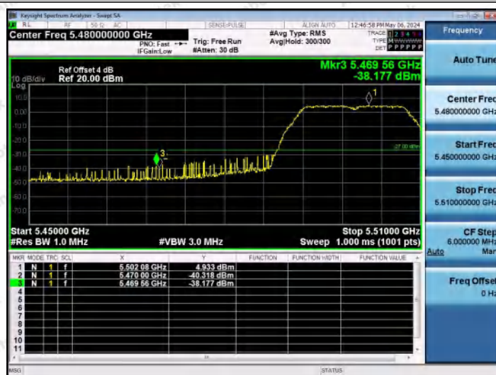
11A-Ant0-5500-PASS
