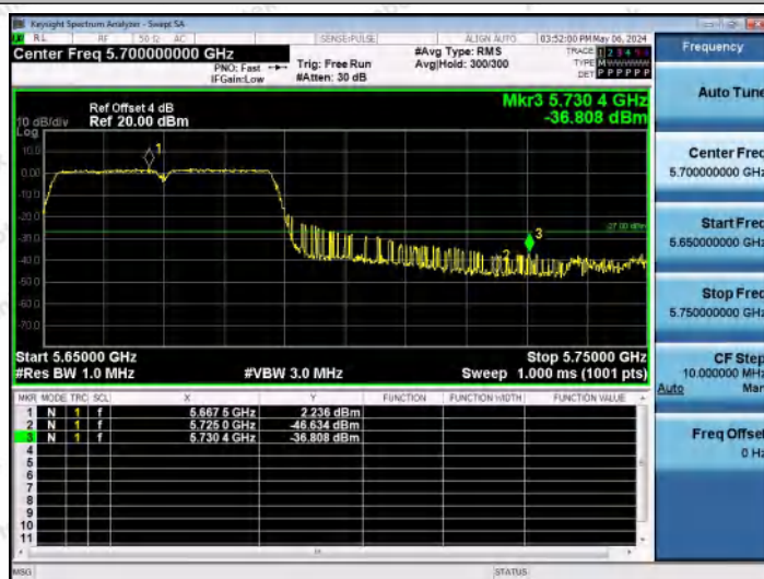
11AC40MIMO-Ant1-5670-PASS
