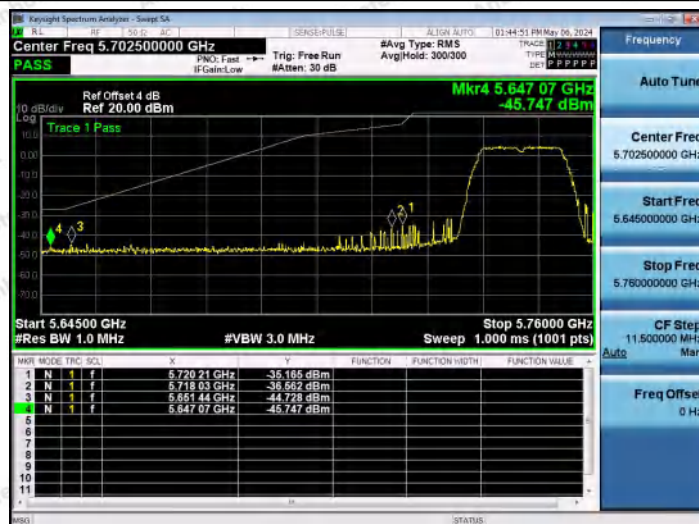
11AC20MIMO-Ant0-5745-PASS
