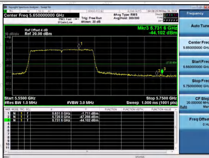
11AC80MIMO-Ant1-5610-PASS
