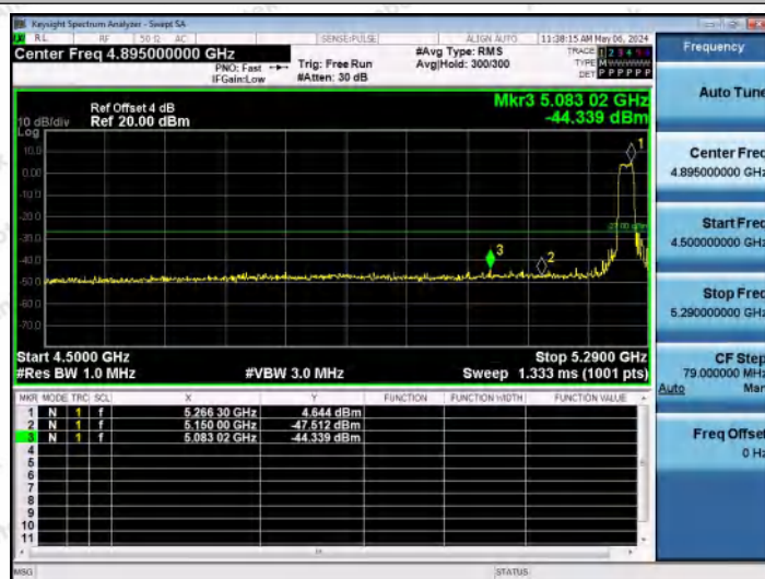
11N20MIMO-Ant1-5260-PASS
