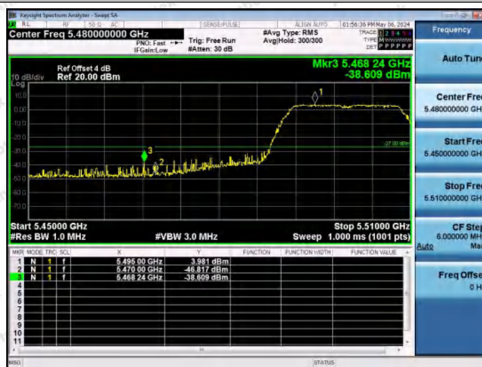
11AC20MIMO-Ant0-5500-PASS
