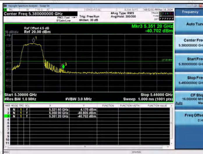
11AC20MIMO-Ant1-5320-PASS
