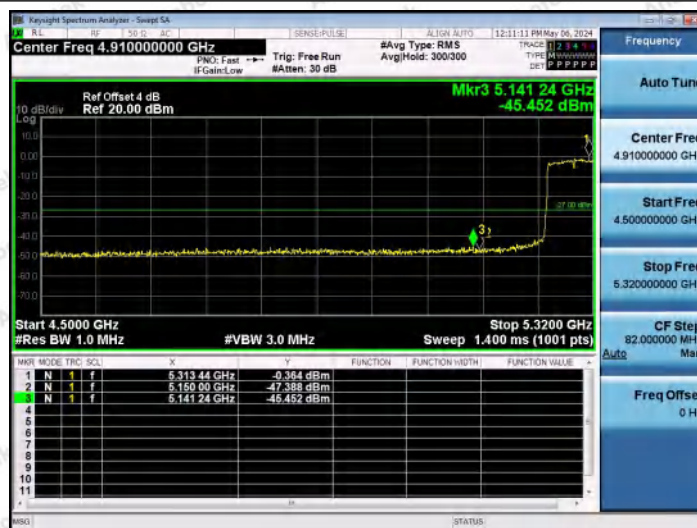
11AC80MIMO-Ant0-5290-PASS
