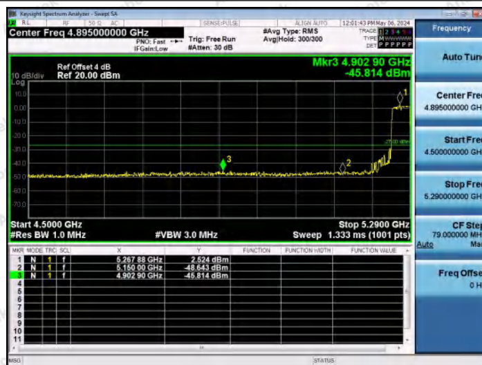
11AC40MIMO-Ant0-5270-PASS
