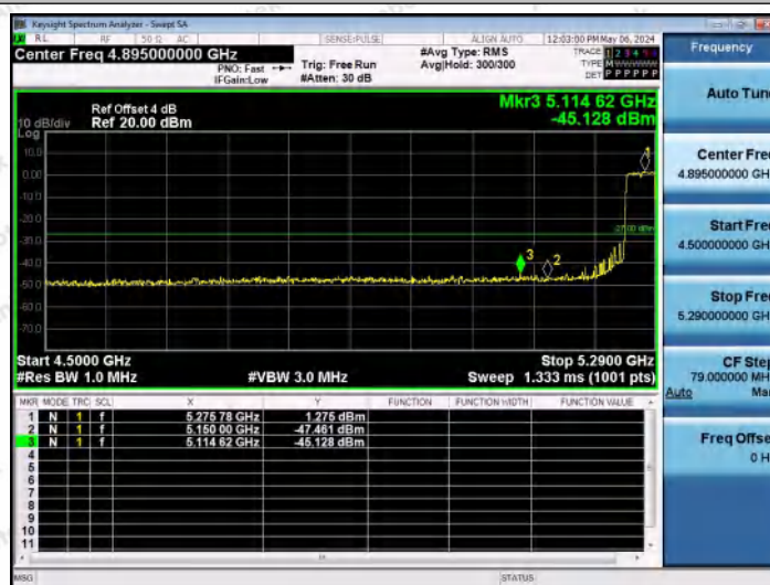
11AC40MIMO-Ant1-5270-PASS
