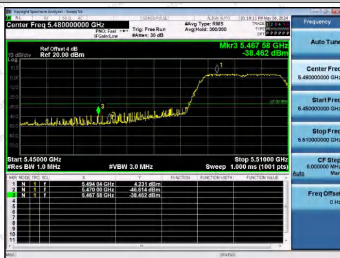
11N20MIMO-Ant0-5500-PASS
