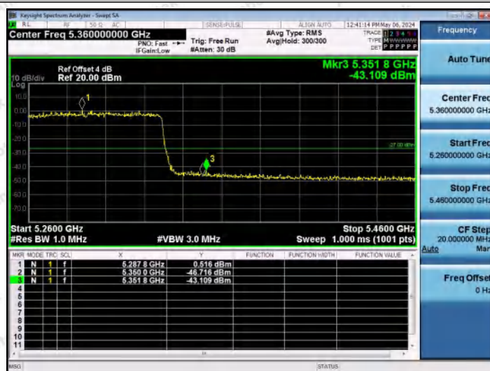
11AX80MIMO-Ant0-5290-PASS
