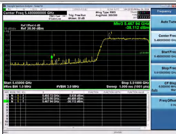
11AX20MIMO-Ant0-5500-PASS
