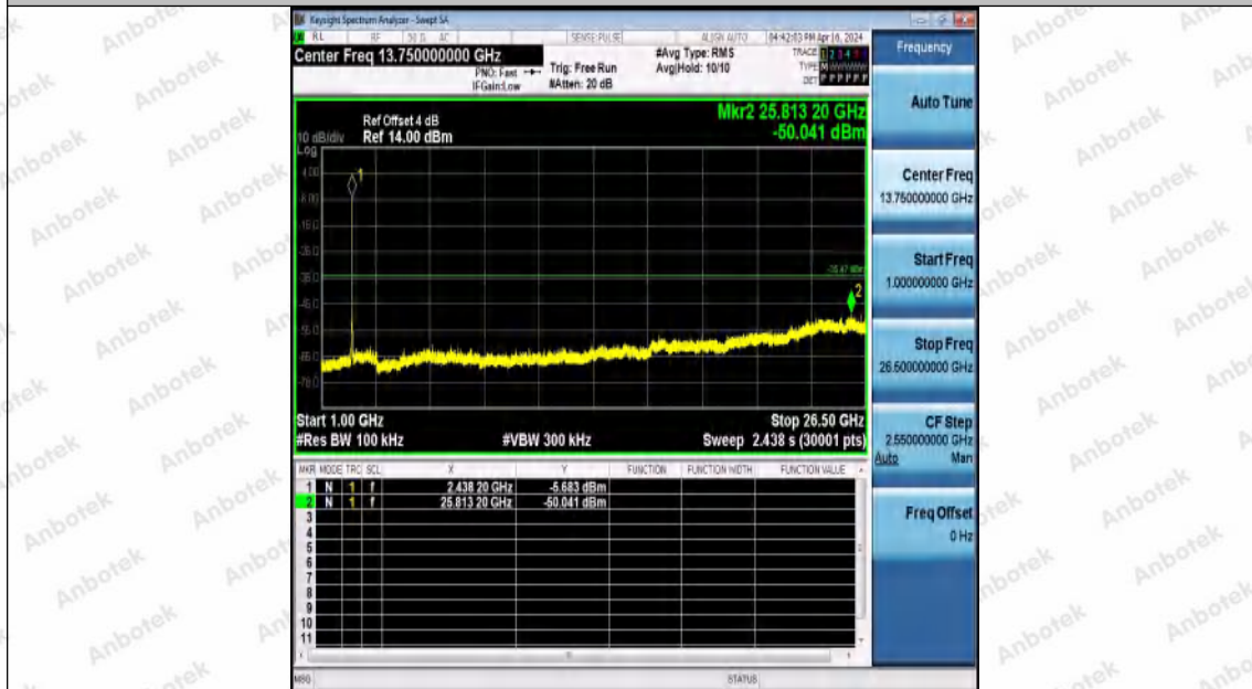
11AX20MIMO-Ant1-2437-1000~26500-PASS
