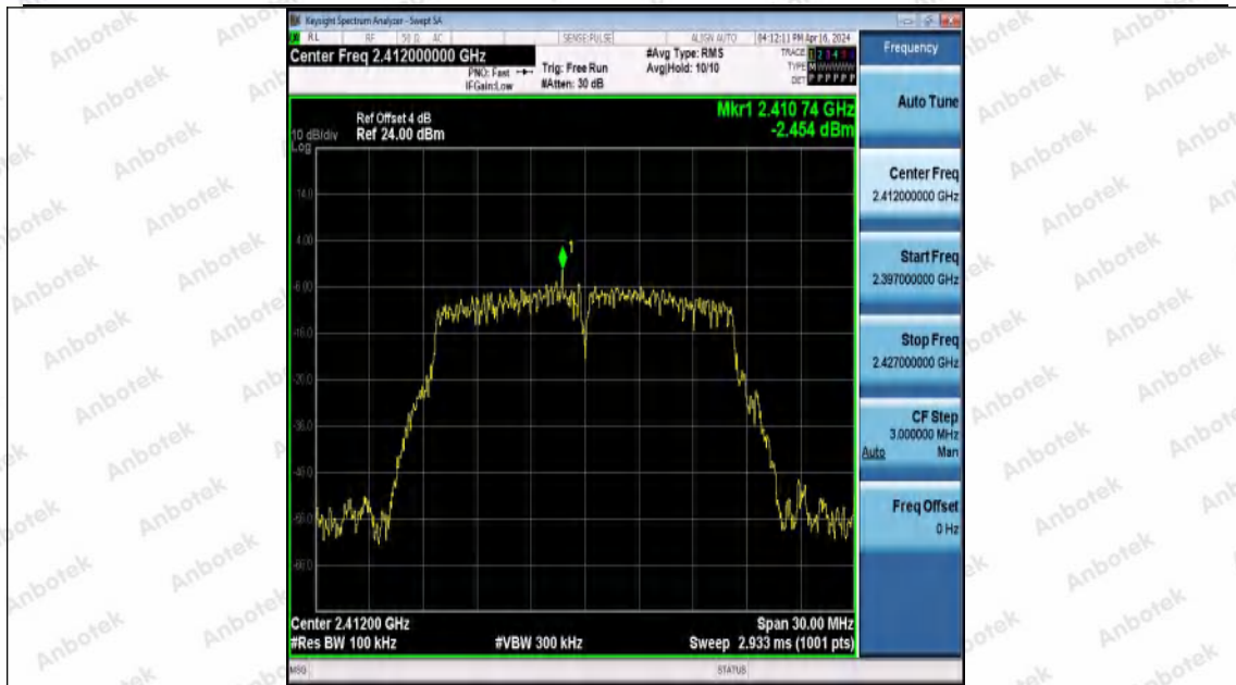
11G-Ant0-2412-0~Reference-PASS
