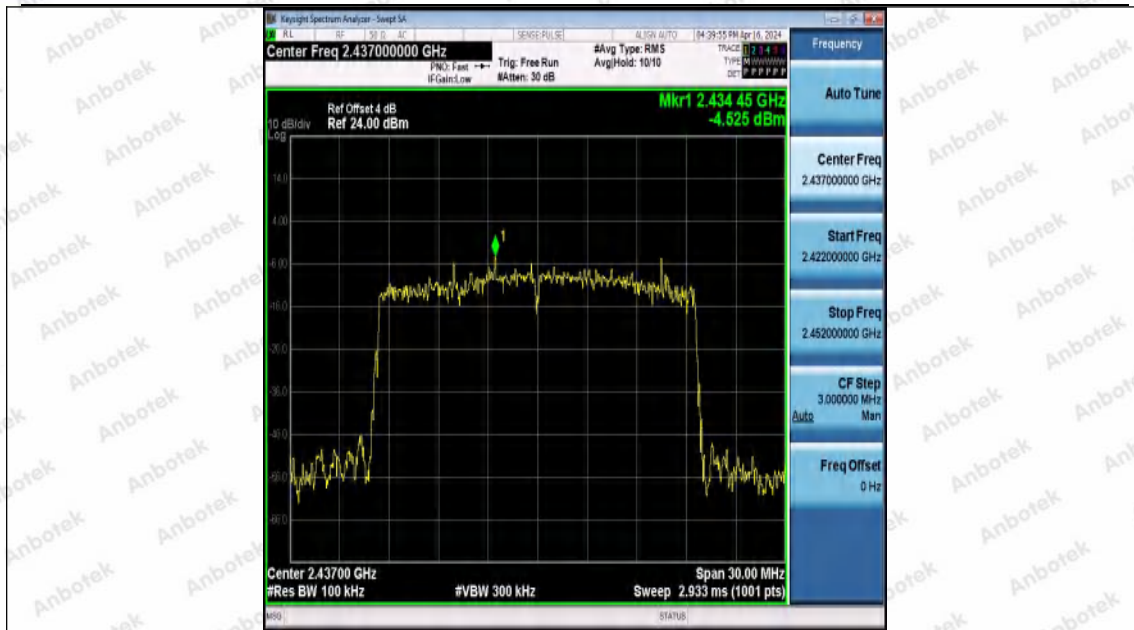
11AX20MIMO-Ant0-2437-0~Reference-PASS
