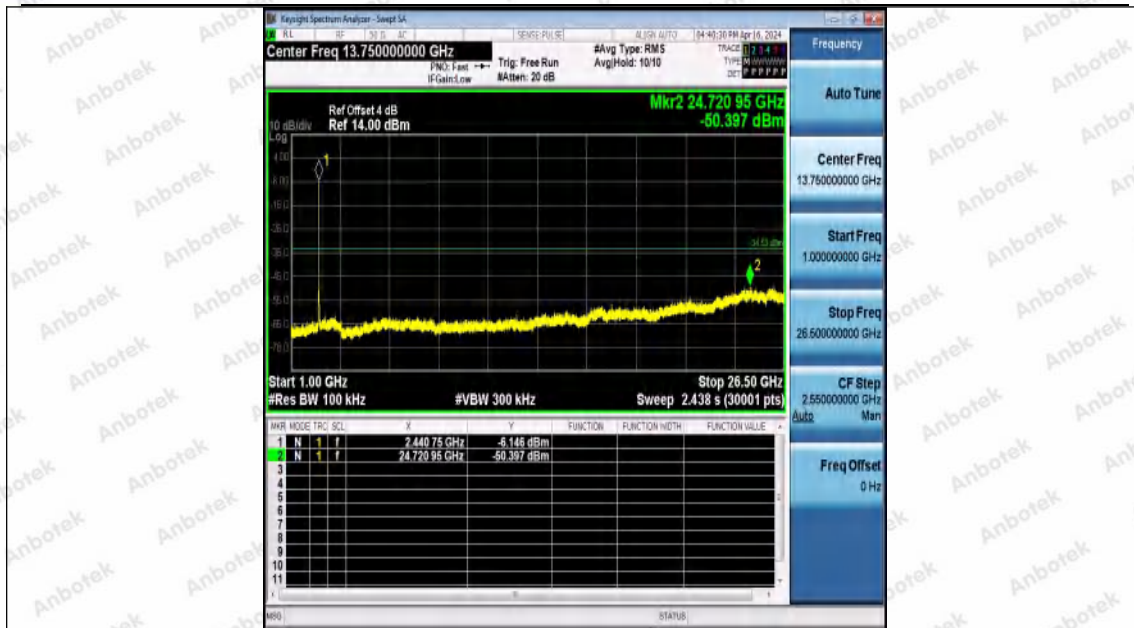
11AX20MIMO-Ant0-2437-1000~26500-PASS
