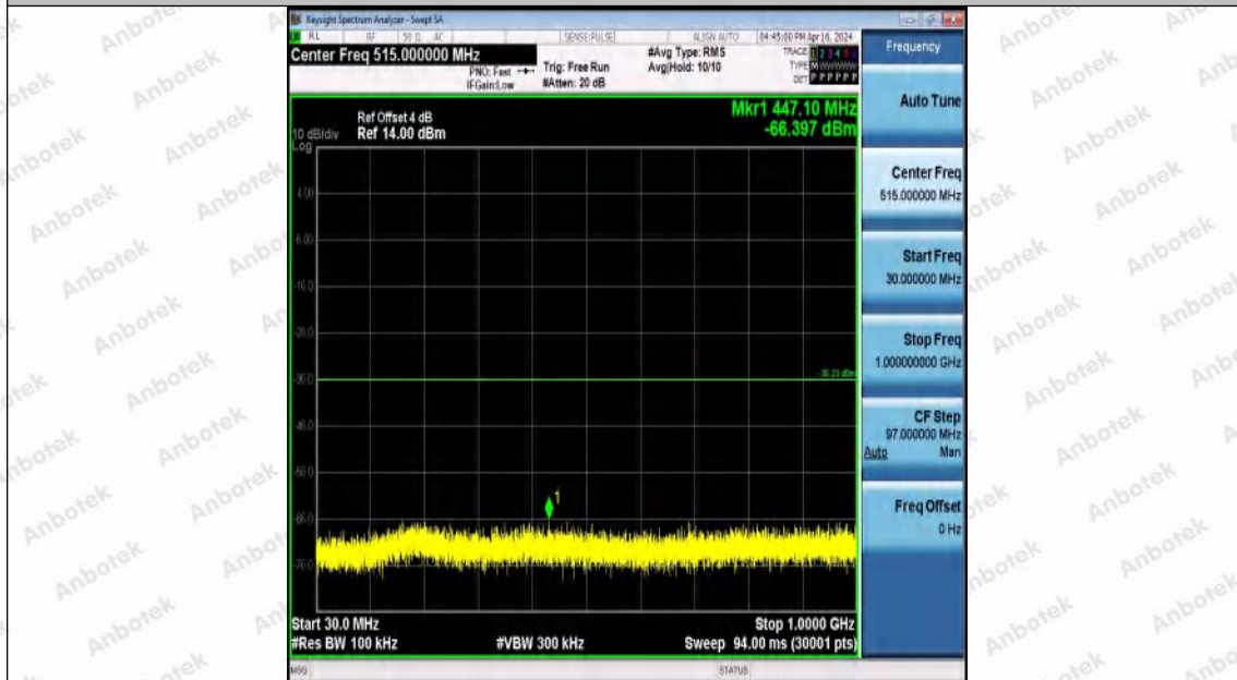
11AX20MIMO-Ant1-2462-30~1000-PASS
