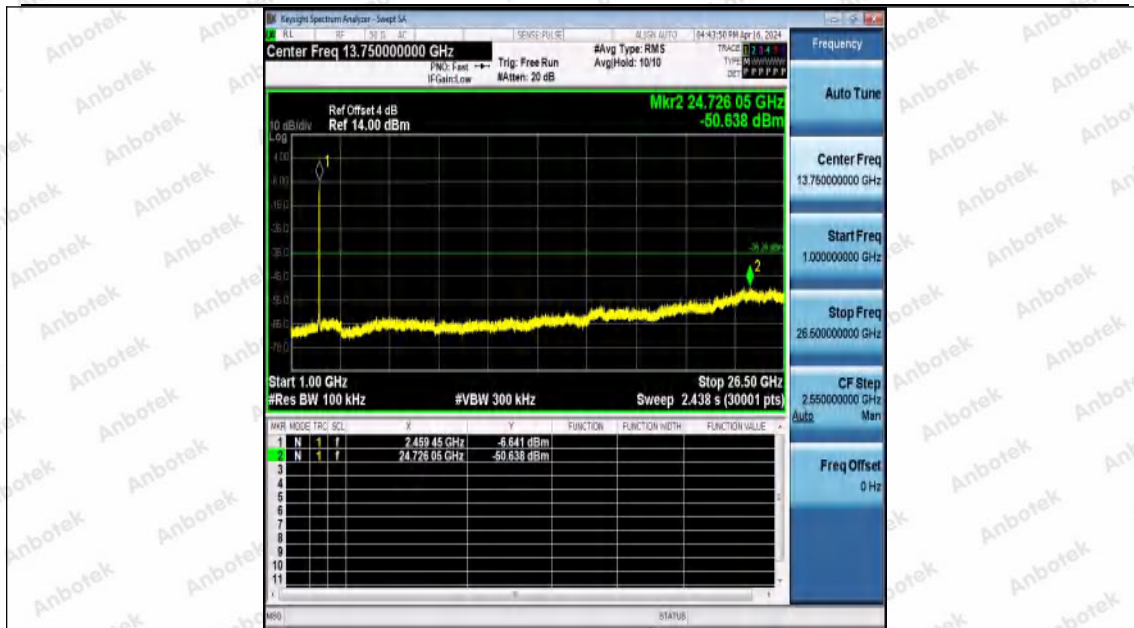
11AX20MIMO-Ant0-2462-1000~26500-PASS
