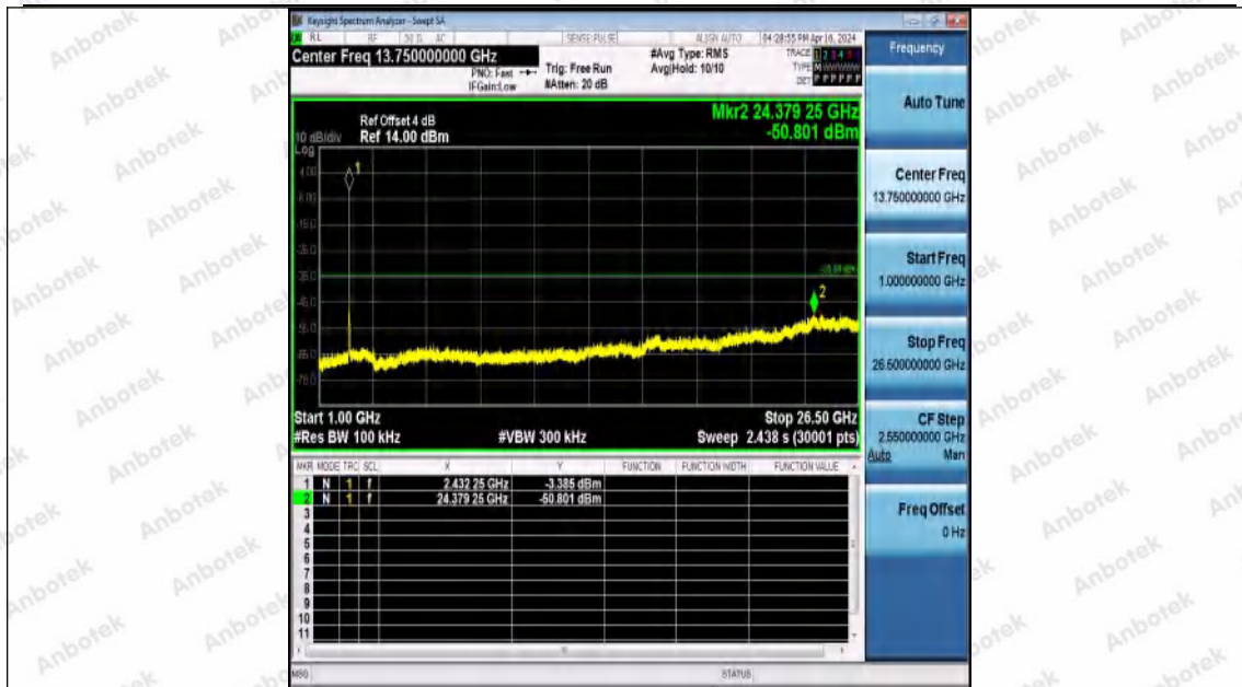
11N20MIMO-Ant0-2437-1000~26500-PASS
