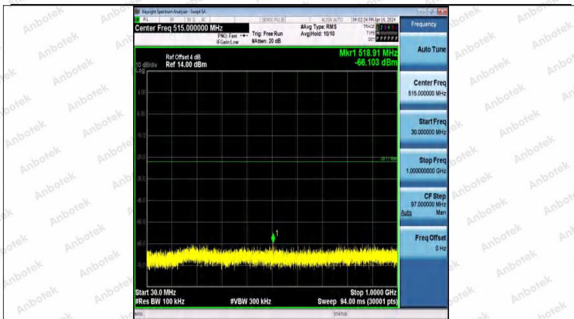
11B-Ant0-2437-30~1000-PASS
