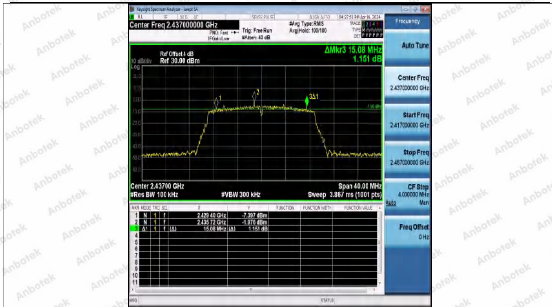
11N20MIMO-Ant0-2437-PASS
