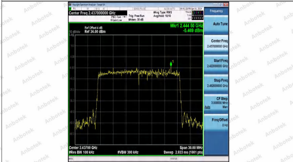
11AX20MIMO-Ant1-2437-0~Reference-PASS
