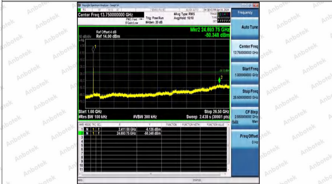
11AX20MIMO-Ant1-2412-1000~26500-PASS
