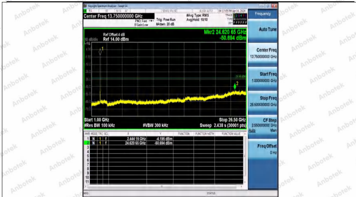
11G-Ant0-2437-1000~26500-PASS
