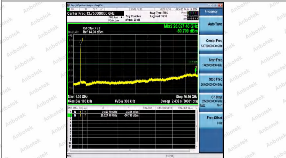
11N20MIMO-Ant1-2462-1000~26500-PASS
