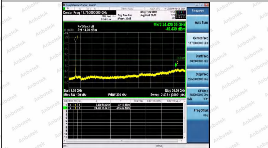
11N20MIMO-Ant1-2437-1000~26500-PASS
