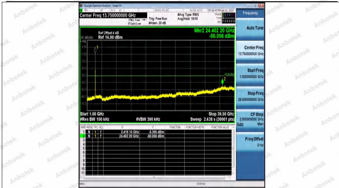
11AX20MIMO-Ant0-2412-1000~26500-PASS
