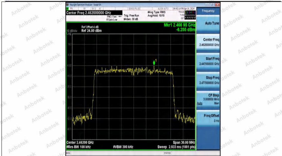
11AX20MIMO-Ant0-2462-0~Reference-PASS
