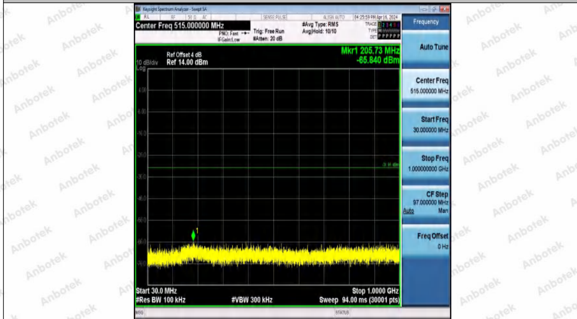
11N20MIMO-Ant1-2412-30~1000-PASS
