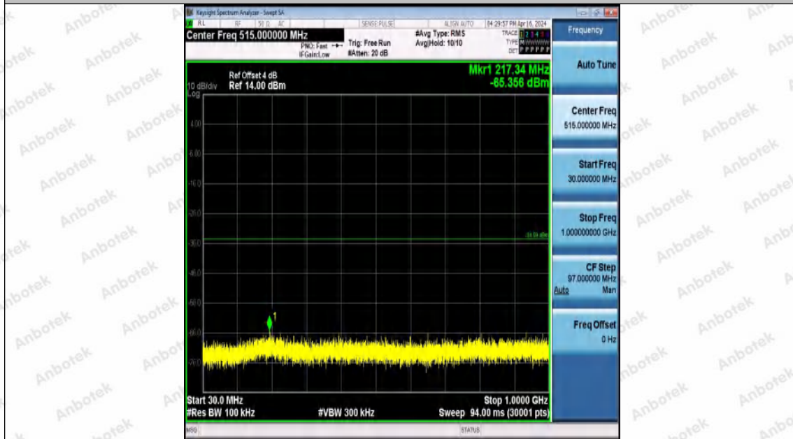
11N20MIMO-Ant1-2437-30~1000-PASS
