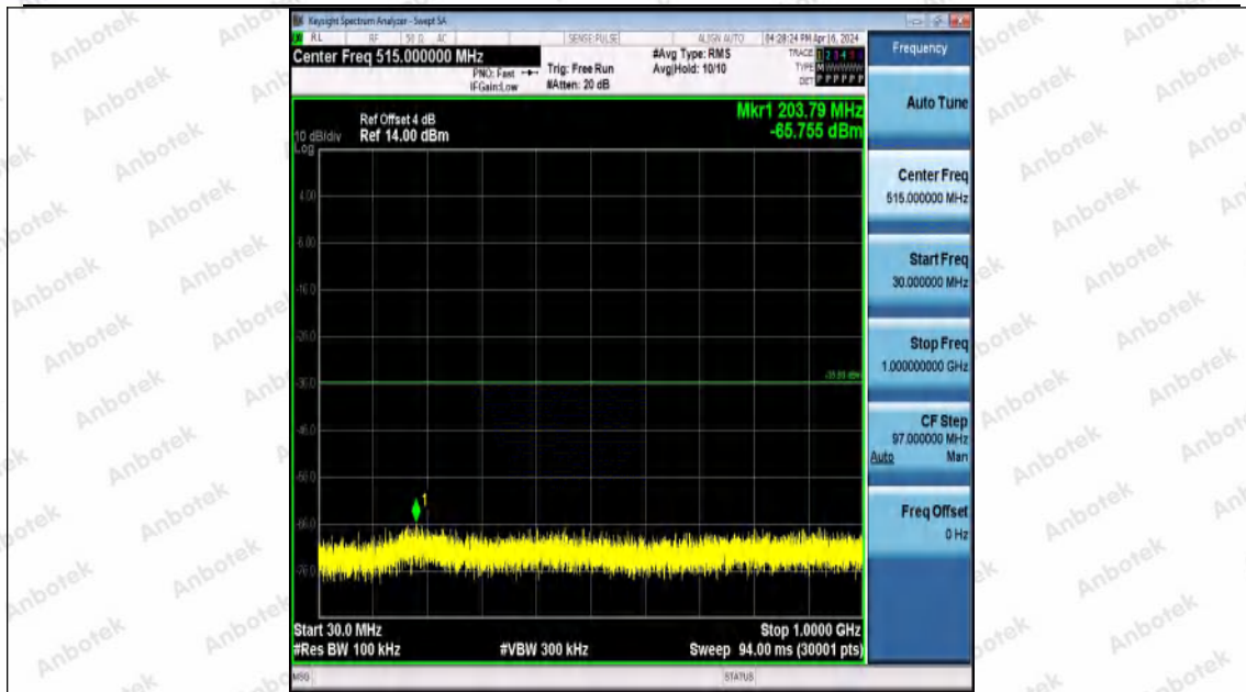
11N20MIMO-Ant0-2437-30~1000-PASS
