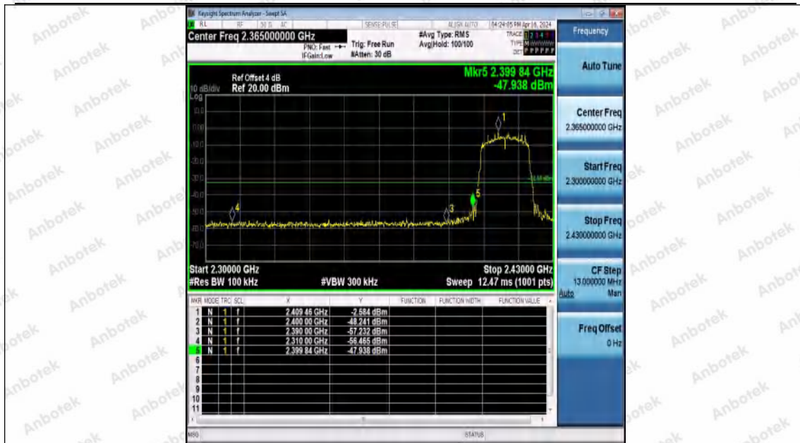
11N20MIMO-Ant0-2412-PASS
