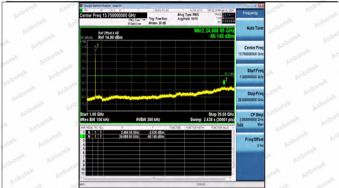
11N20MIMO-Ant0-2462-1000~26500-PASS
