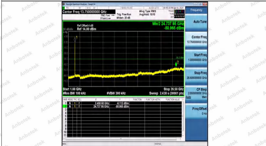
11AX20MIMO-Ant1-2462-1000~26500-PASS
