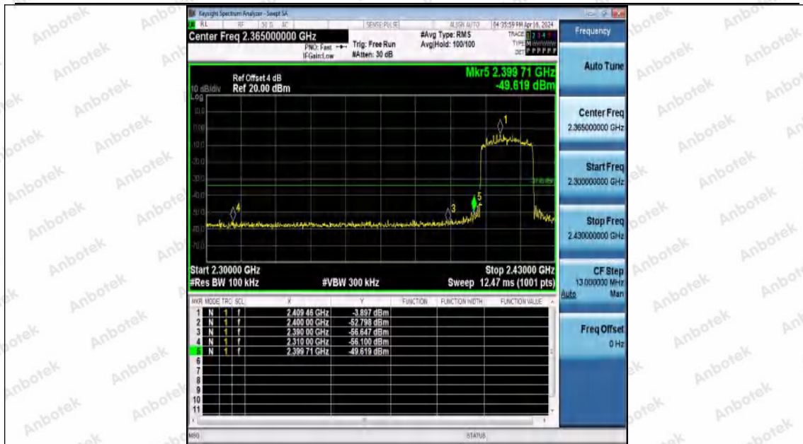
11AX20MIMO-Ant0-2412-PASS
