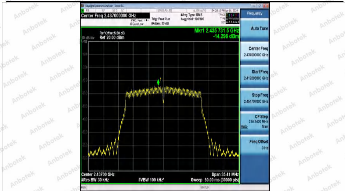
11N20MIMO-Ant0-2437-PASS
