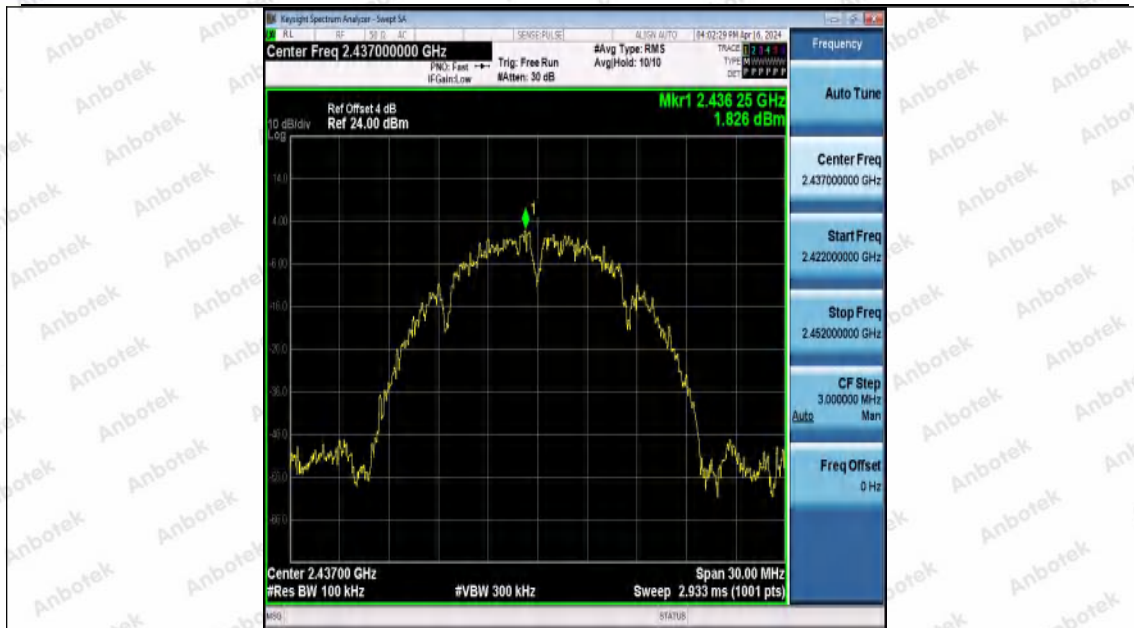
11B-Ant0-2437-0~Reference-PASS
