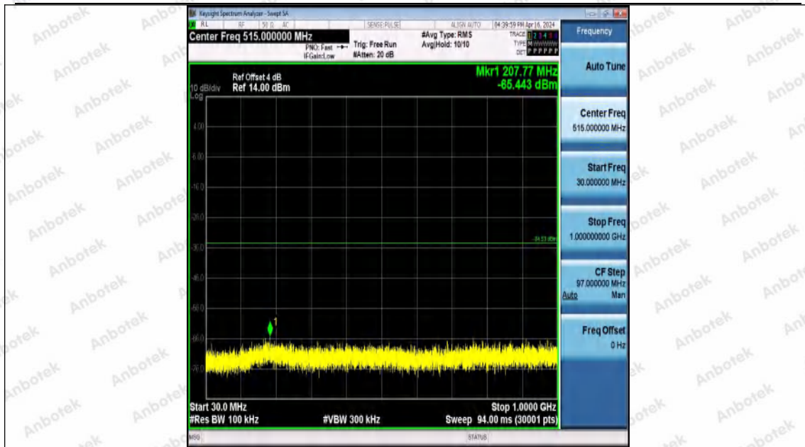
11AX20MIMO-Ant0-2437-30~1000-PASS
