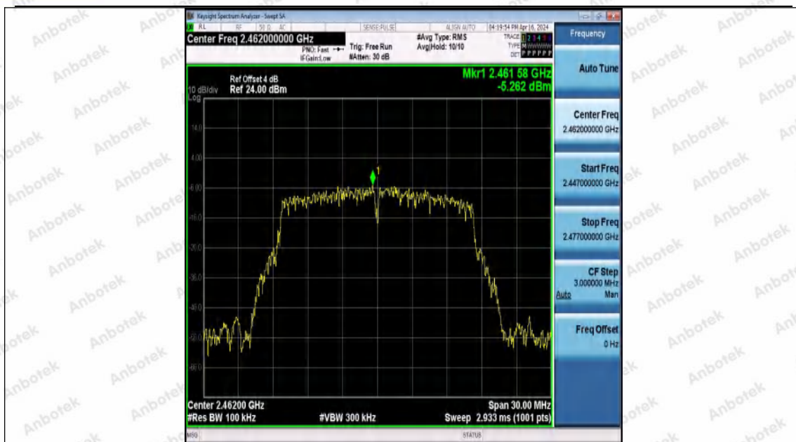
11G-Ant0-2462-0~Reference-PASS
