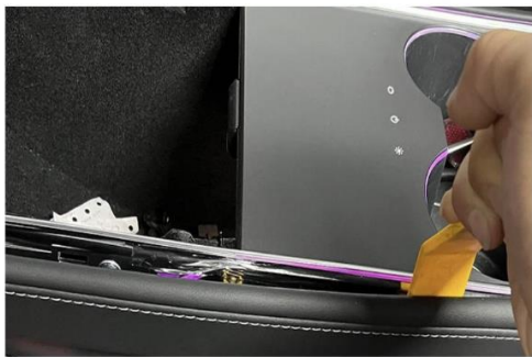
1. Pry open and remove the original central console cover plate
