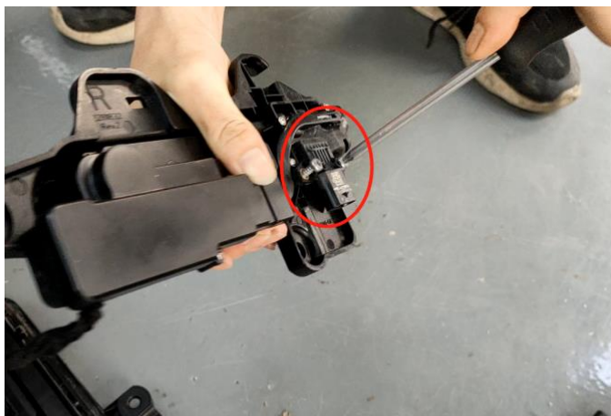
(10).将原车上的信号器拆装到相对应的电动把手上，用原车螺丝固定 Disassemble the signal on the original vehicle to the corresponding electric handle and fix it with the original vehicle screw
