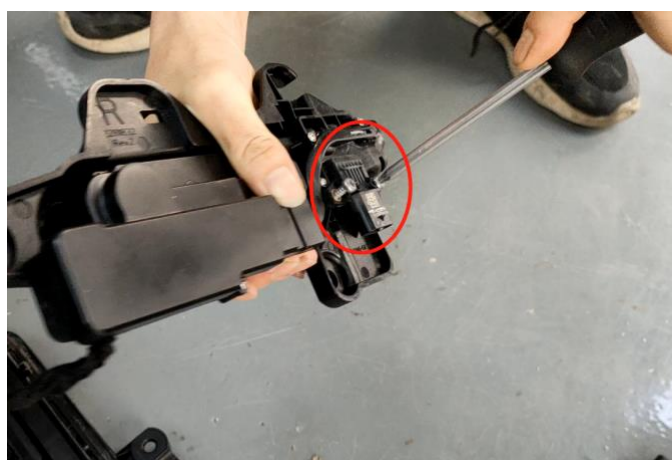
(7).将原车上的信号器拆装到相对应的电动把手上,用原车螺丝固定 Disassemble the signal on the original vehicle to the corresponding electric handle and fix it with the original vehicle screw
