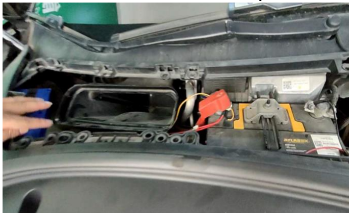
(1) 在前盖电池取电，左边找孔穿线至副驾驶 Connect the cable to the battery in the front cover, find a hole on the left side and thread the cable to the co-pilot
