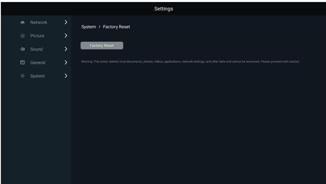
Figure 6-19 Factory reset
