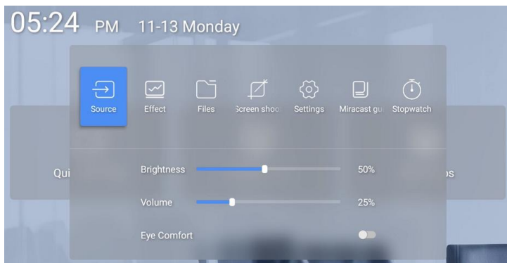
Figure 4-15 Menu
