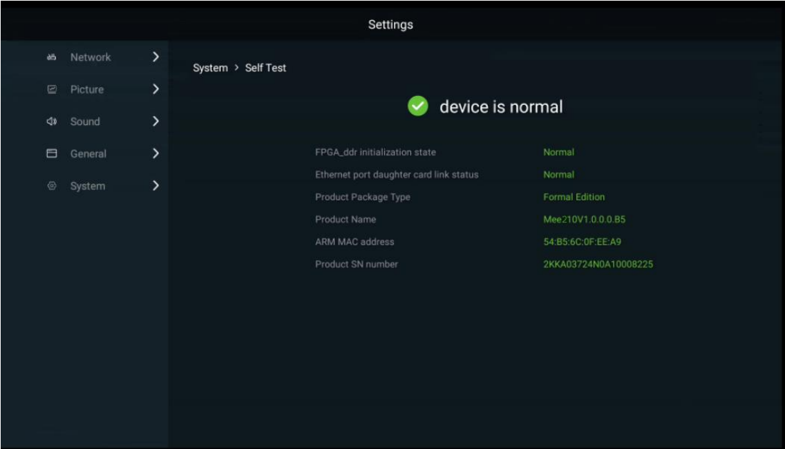
Figure 6-23 Self-test
