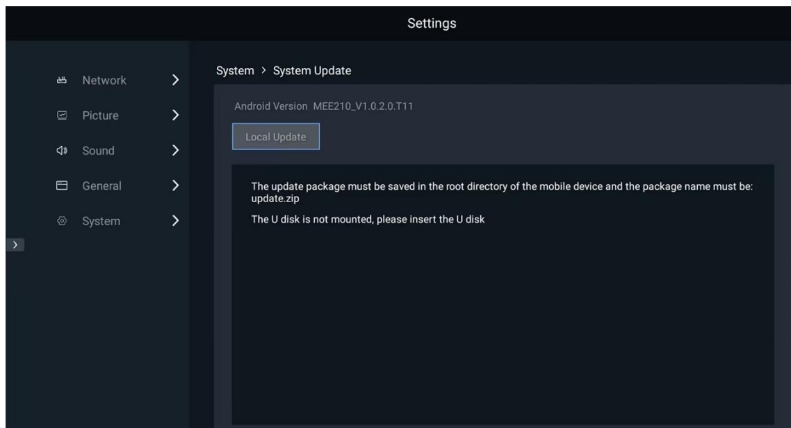
Figure 6-20 System update
