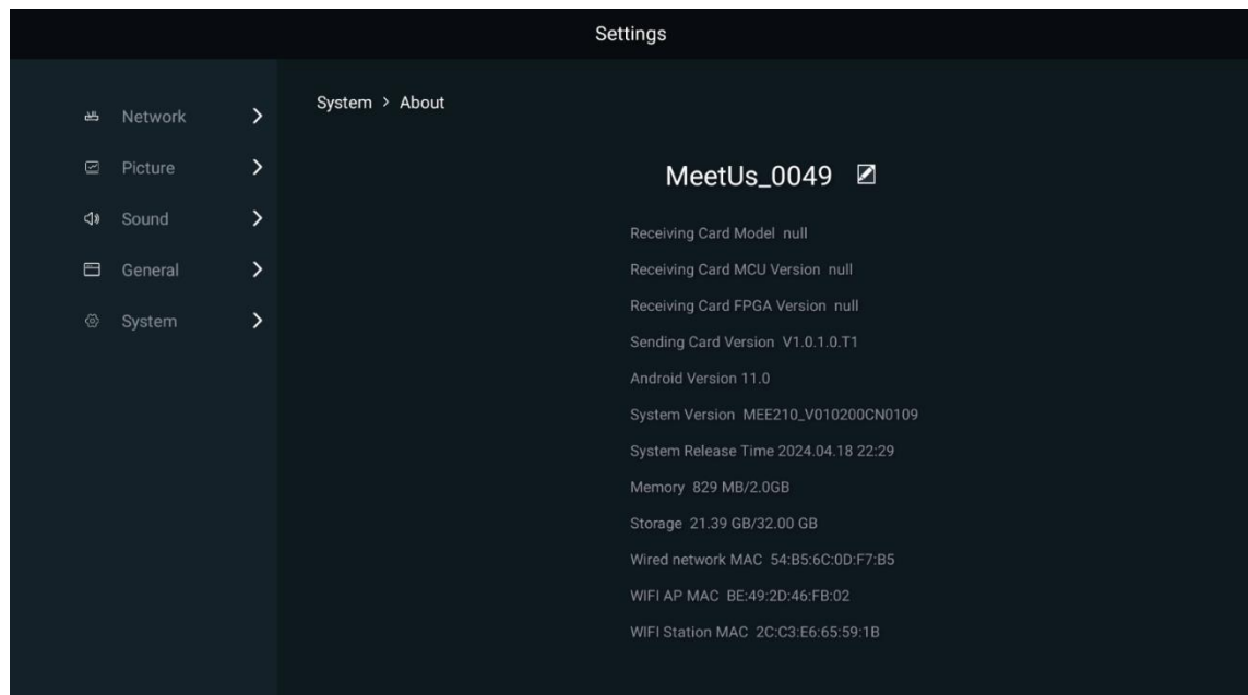
Figure 6-21 About
