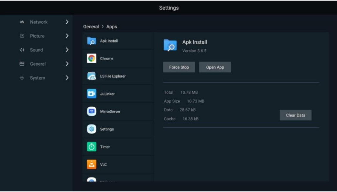
Figure 6-9 App management
