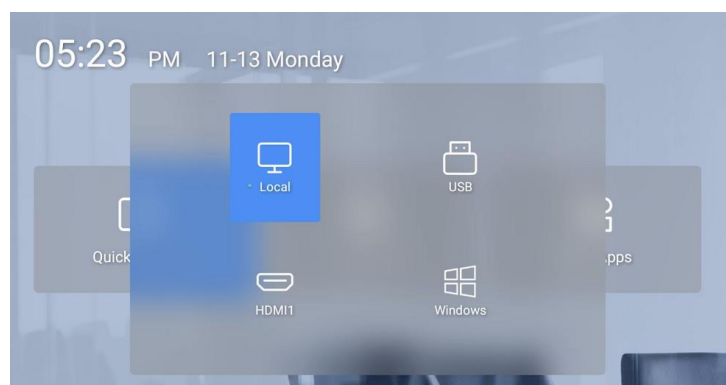
Figure 4-14 Presentation
