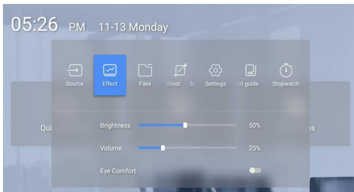
Figure 5-1 Menu
