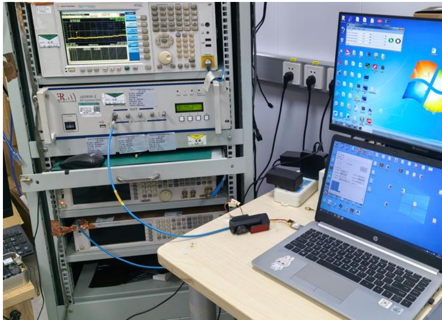
Photo of Conducted Emission Measurement
