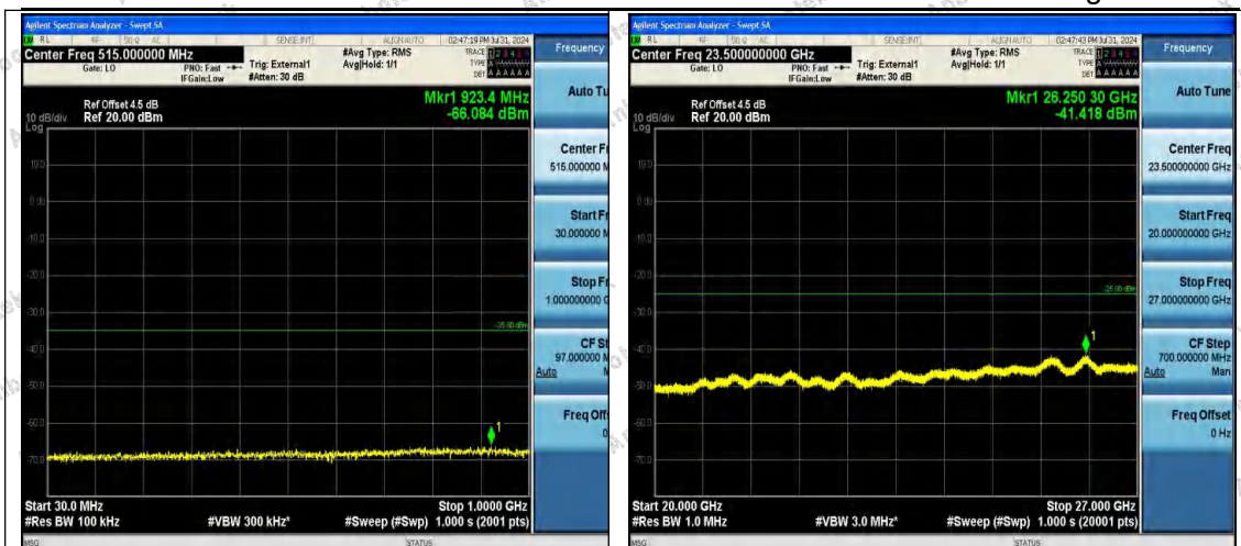
Band41_20MHz_16QAM_40620_1RB#0_30~10 00_30~1000
