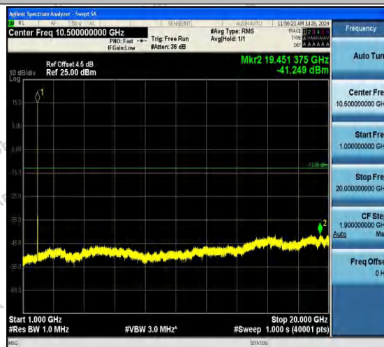
Band2-9538-3-1000~20000MHz-PASS
