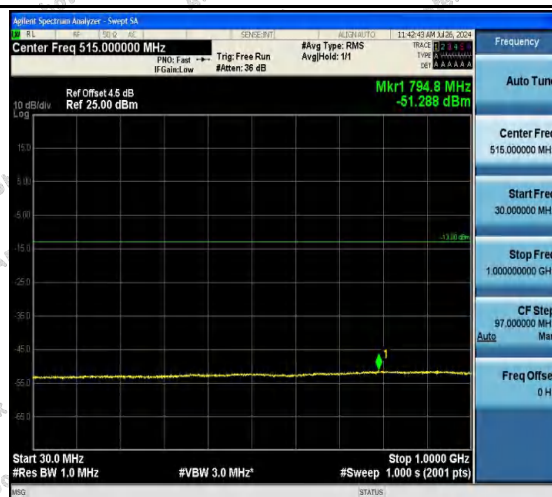
Band2-9400-2-30~1000MHz-PASS
