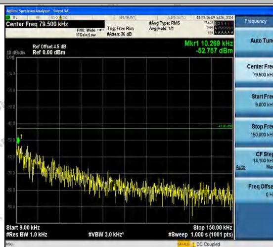
Band2-9538-2-0.009~0.15MHz-PASS
