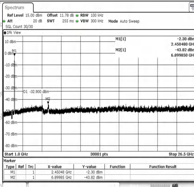
11N40SISO-Ant1-2452-1000~26500-PASS
