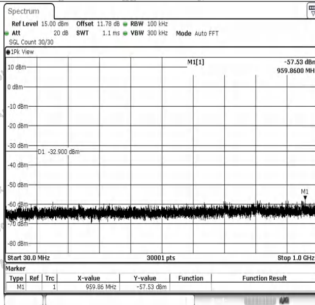
11N40SISO-Ant1-2452-30~1000-PASS
