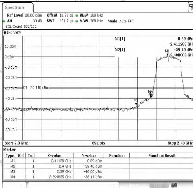
11G-Ant1-2412-PASS
