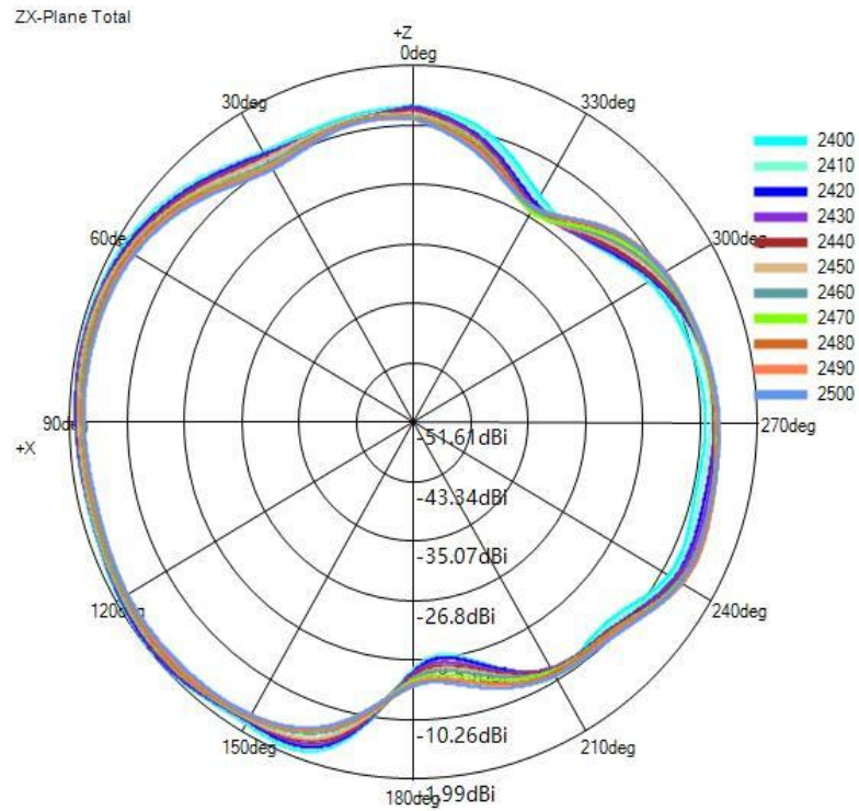
(1) X-Z Plane(unit:dBi):
