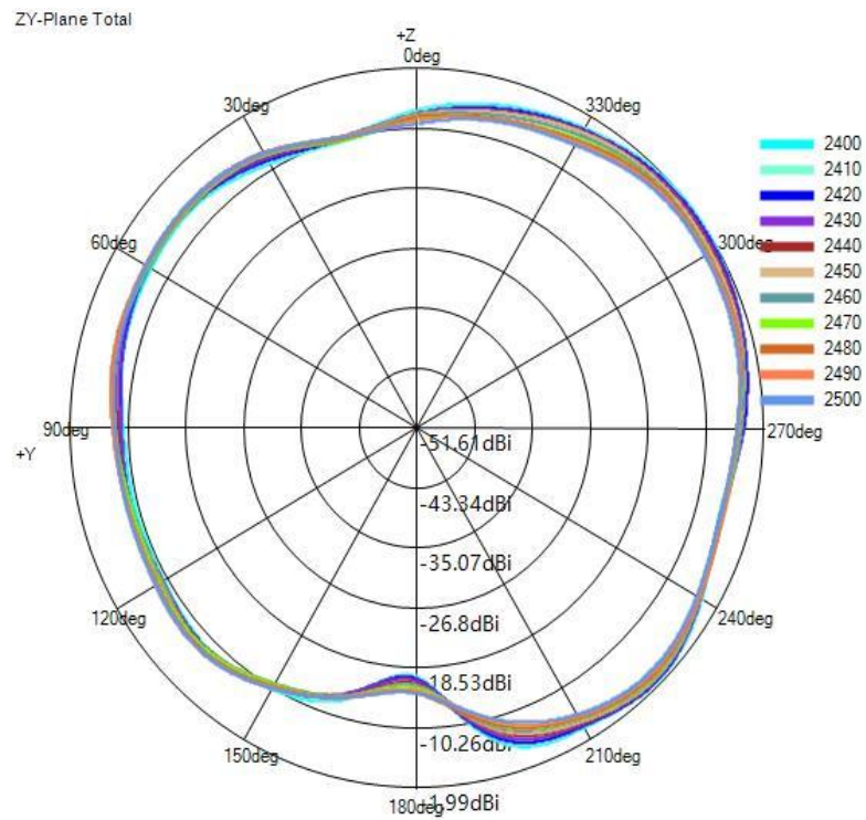
(2) Y-Z Plane(unit:dBi):
