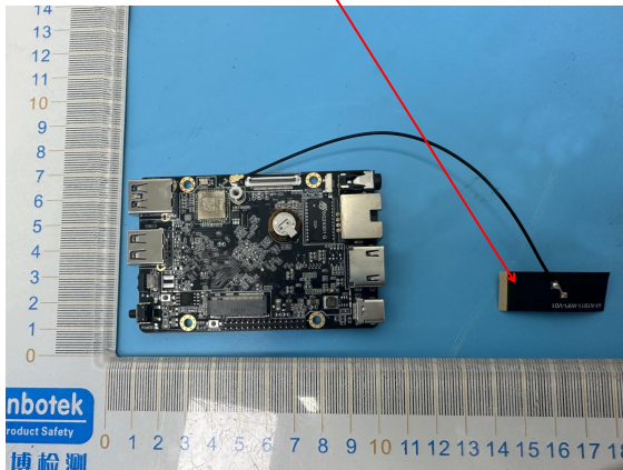
original antenna: 2.25dBi(Max)
