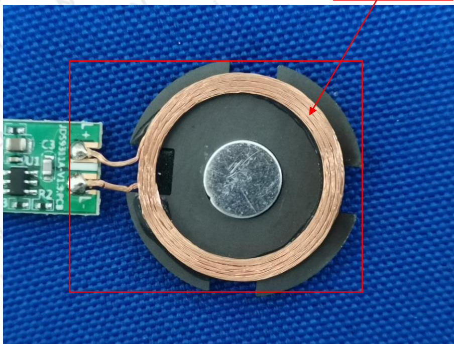
Coil Antenna
