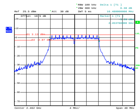
g_2462MHz_Chain 0
