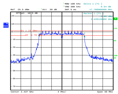
n20_2437MHz_Chain 0
