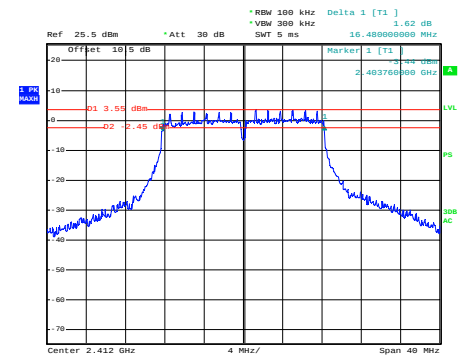
g_2412MHz_Chain 0
