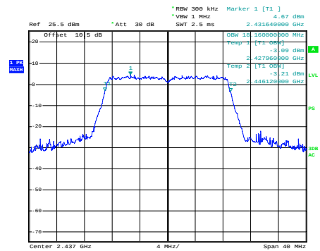
n20_2437MHz_Chain 0
