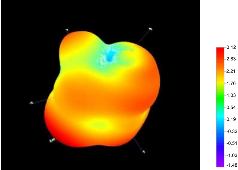
B1.1 3D Pattern for2400MHz
