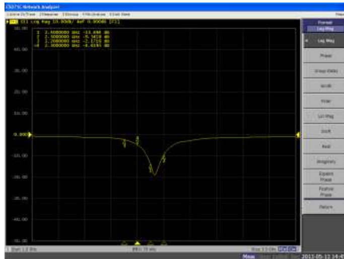
figure 2 Keyboard Antenna S11
