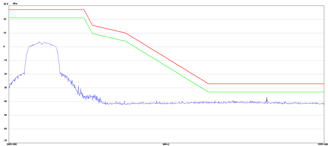
Horizontal High Channel (5825 MHz)-Above 1G
