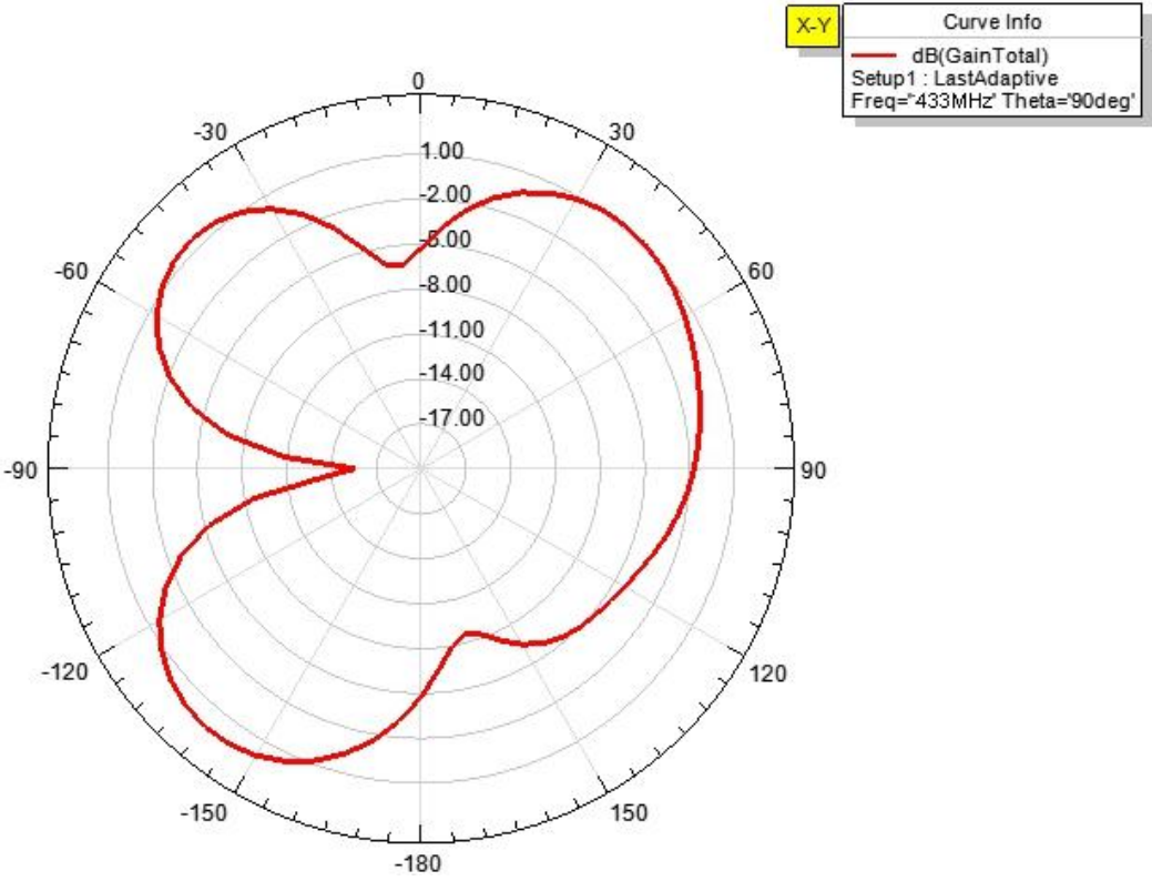
Radiation Pattern 2
