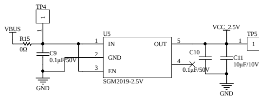
2.5V_LDO电路
