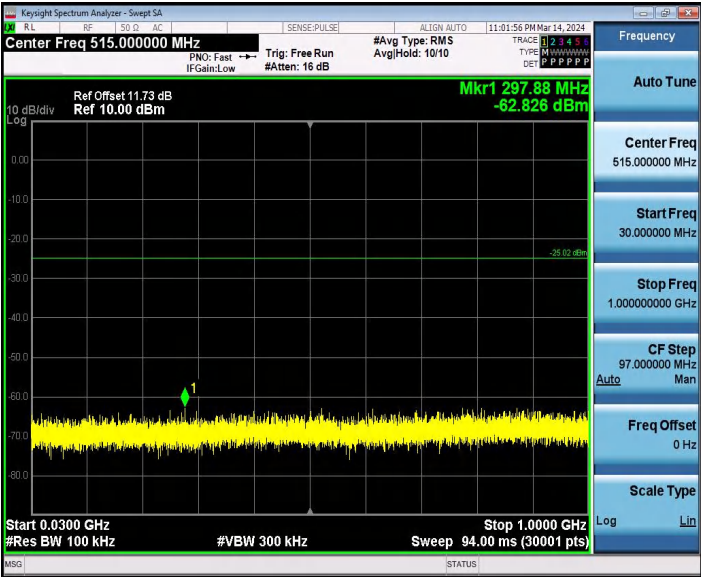
30MHz-1GHz
