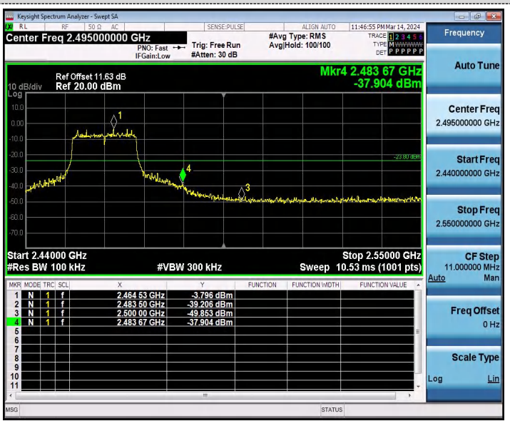
Right bandedge
