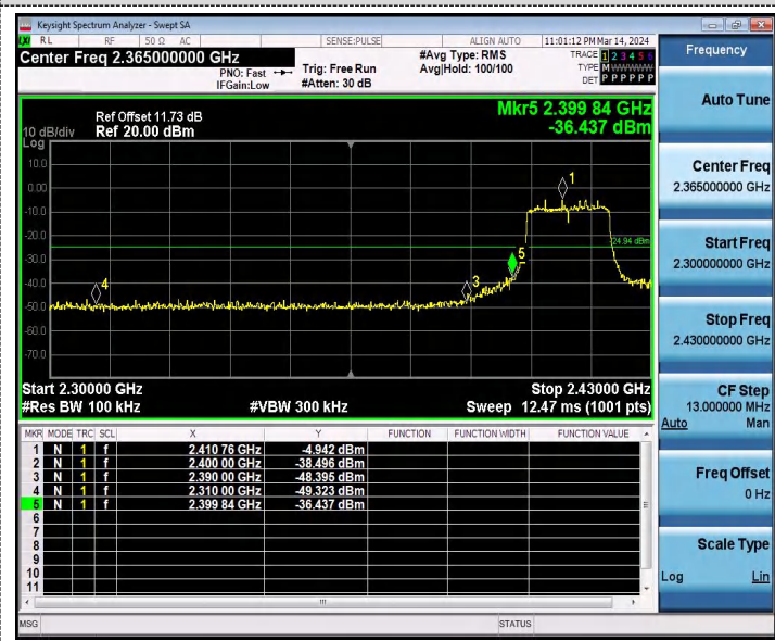
Left bandedge
