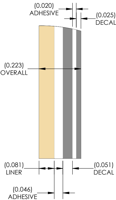
DETAIL A - LABEL & LAMINATE SCALE 100:1
