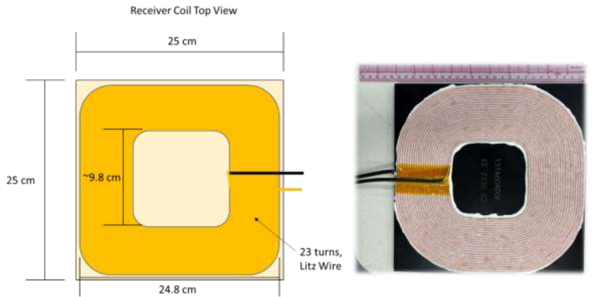
Figure 22: Receiver Internal Coil Top View
