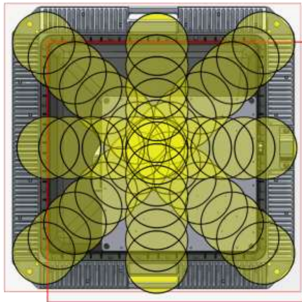
Figure 17: Top-side Measurement Locations of Lowest-coupling Conditions with the ELT-400 100 cm 2 Probe Represented by Yellow Circles (to scale)
