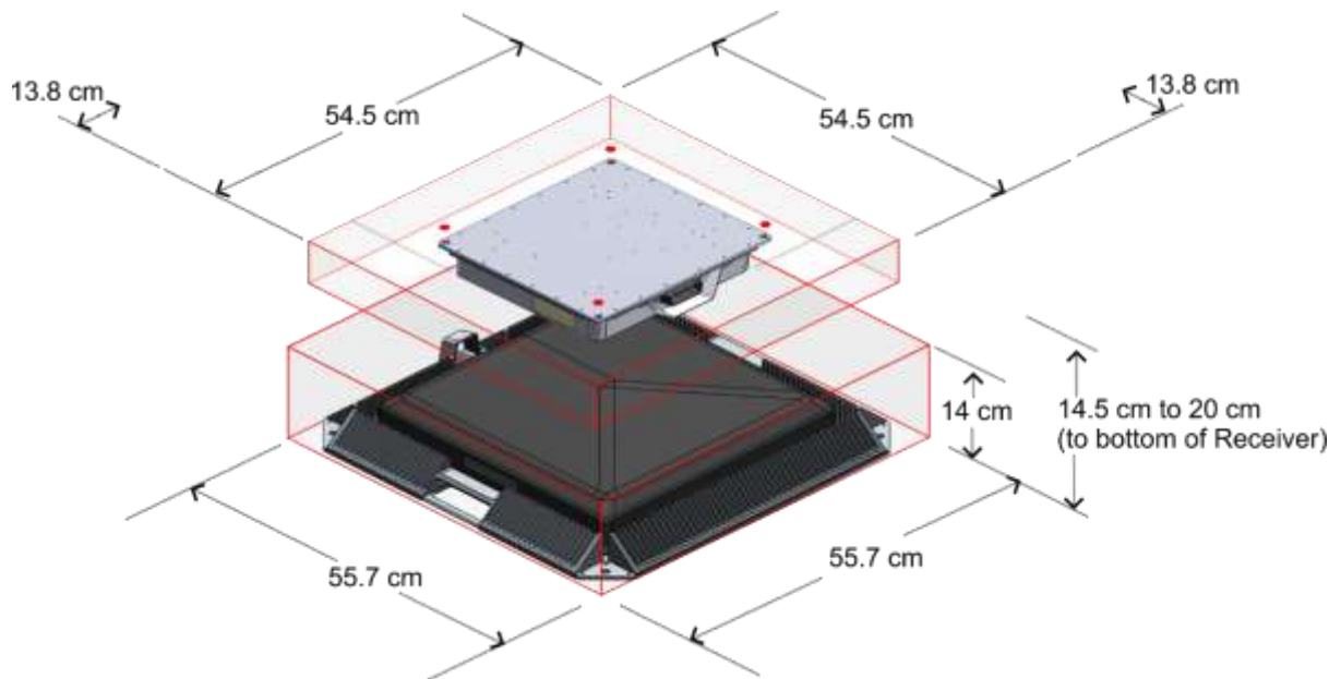
Figure 13: Off-Vehicle Setup with Plexiglass for Measurement Grid Reference
