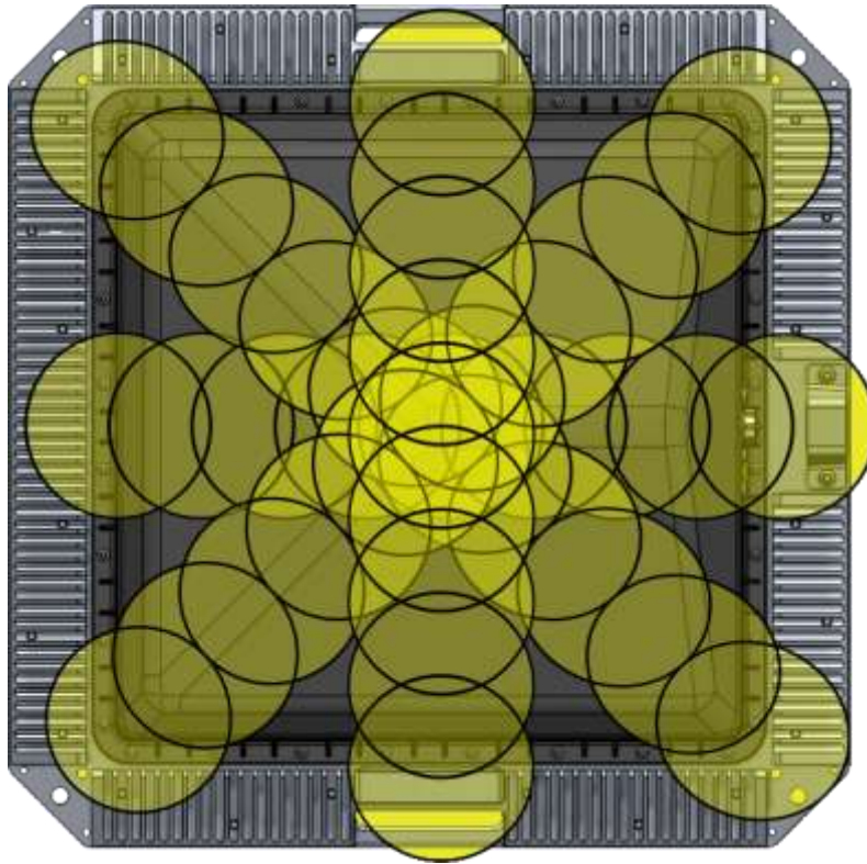
Figure 12: To-Scale Representation of Probe Locations for Standby Measurements
