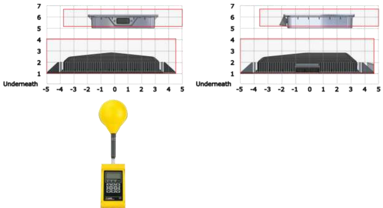
Figure 14: Two sides shown with grid locations setup for lowest-coupling position. Everything is shown to scale.
