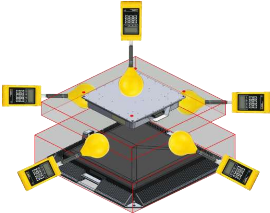
Figure 18: WiTricity WPT System Measurement of 5 Sides with Probes Shown to Scale.
