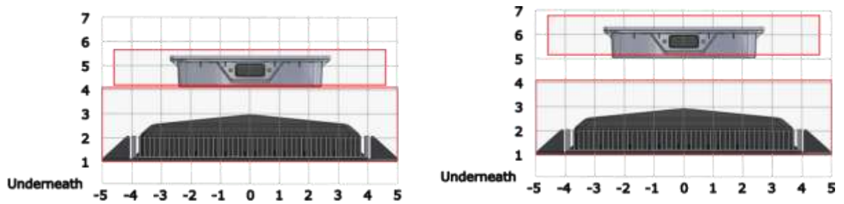
Figure 16: Maximum-coupling (lowest height) - Left; and Nominal-coupling (17 cm height) - Right: One Side of Each
