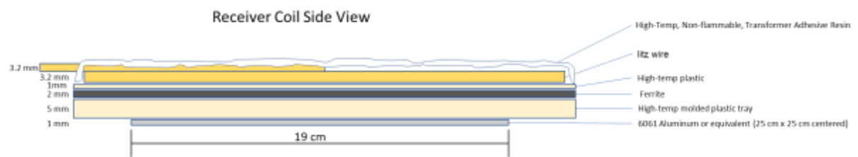
Figure 23: Receiver Internal Coil Side View / Stack-up
