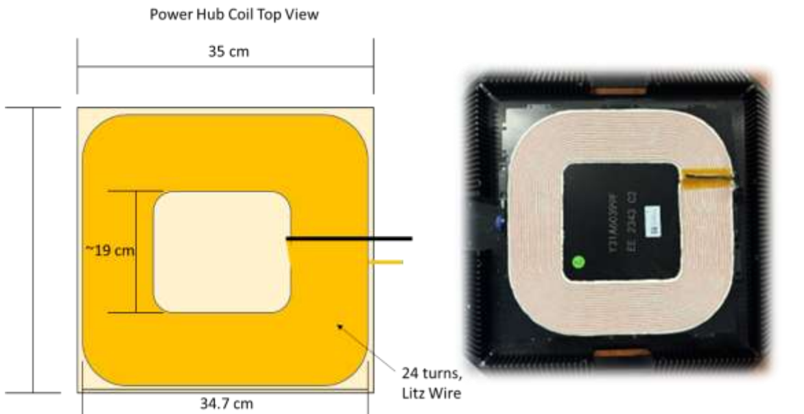
Figure 20: Power Hub Internal Coil Top View
