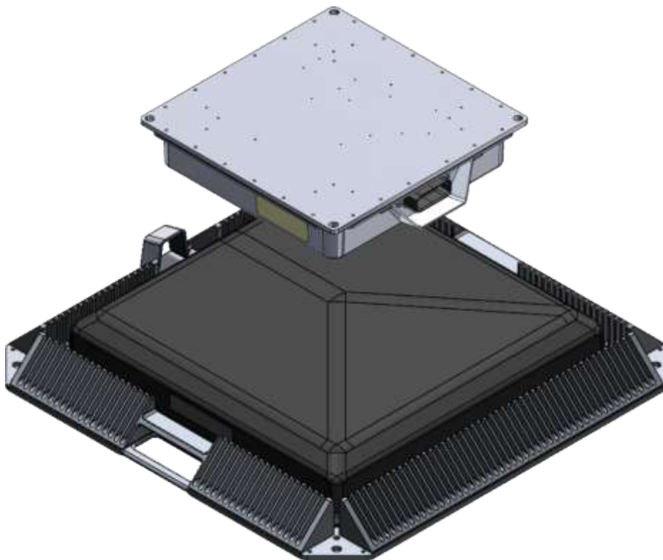
Figure 3: Example of WiTricity Receiver over the Power Hub
