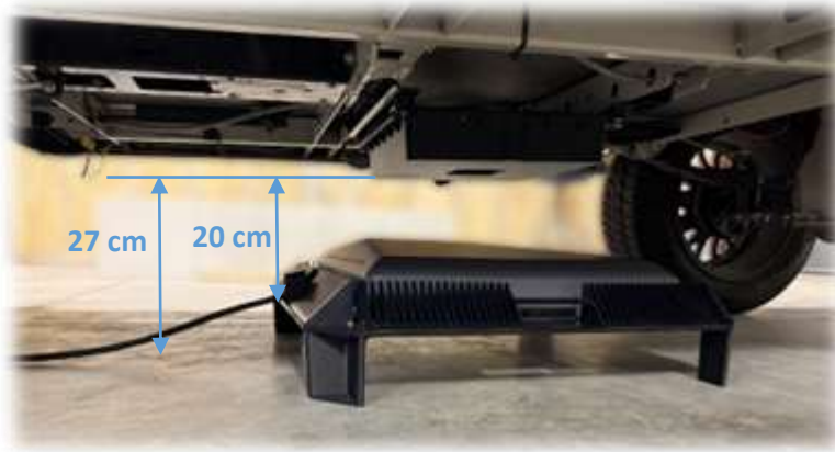
Figure 7: Receiver mounted on real vehicle with actual mounting hardware and Power Hub with 7 cm risers
