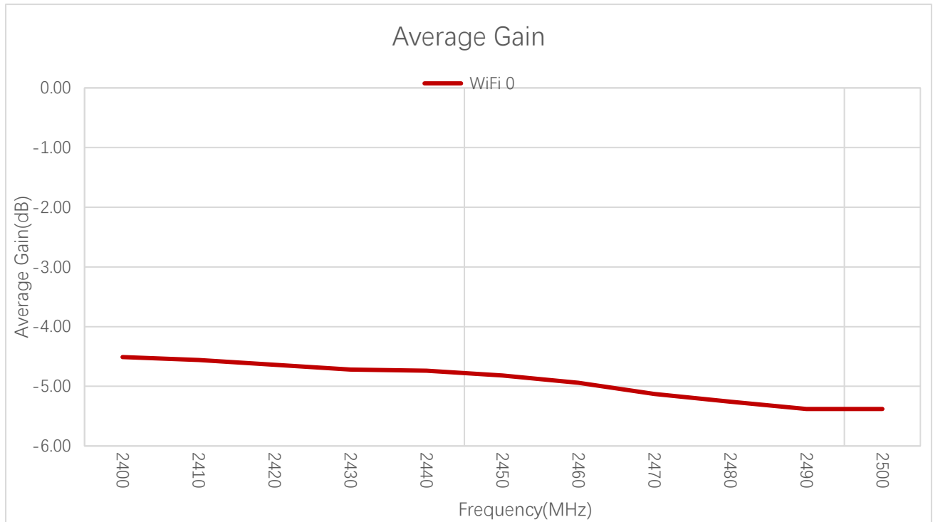
Average Gain (dB) – WIFI 0
