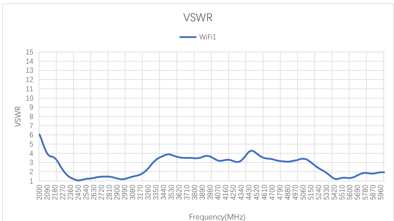
VSWR – WIFI 1
